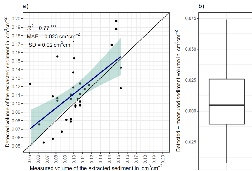
“Figure A3. a) Estimation of Time-of-Flight camera accuracy based on averaging two surface scans before and after the sediment extraction under controlled conditions. The x-axis shows the exact sediment volume measured with a cup. The y-axis represents the volume of the sediment calculated from the camera scans (according to Equation (4)). The blue line is the linear regression calculated from the measured and detected volume. The green shadow shows the confidence interval of 95% for the linear regression slope. ***p ≤ 0.001. MAE is the mean absolute error, SD is standard deviation and R 2 the coefficient of determination. b) Measured sediment volume subtracted from the detected sediment volume for all measurements.”
