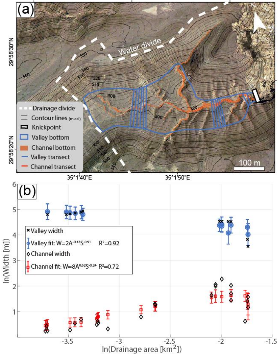
Fig 6: Variations in valley and channel widths along a reversed section (valley 12 in Tables 1 and 2, and Fig. 1d). (a) Valley (blue) and channel (orange) polygons and width transects, sketched over a 0.5 m resolution orthophoto. The slope break between the valley bottom and the hillslope is emphasized by the density change of the 2m contour lines (thin black lines). (b) Width-area-slope scaling of reversed valley width (data in black, fit in blue), which narrows with drainage area, contrasting with the width of the channel (data in black, fit in red) that increases downstream. This difference is expressed by the drainage area exponent, b , which is positive for the channel and negative for the valley.
