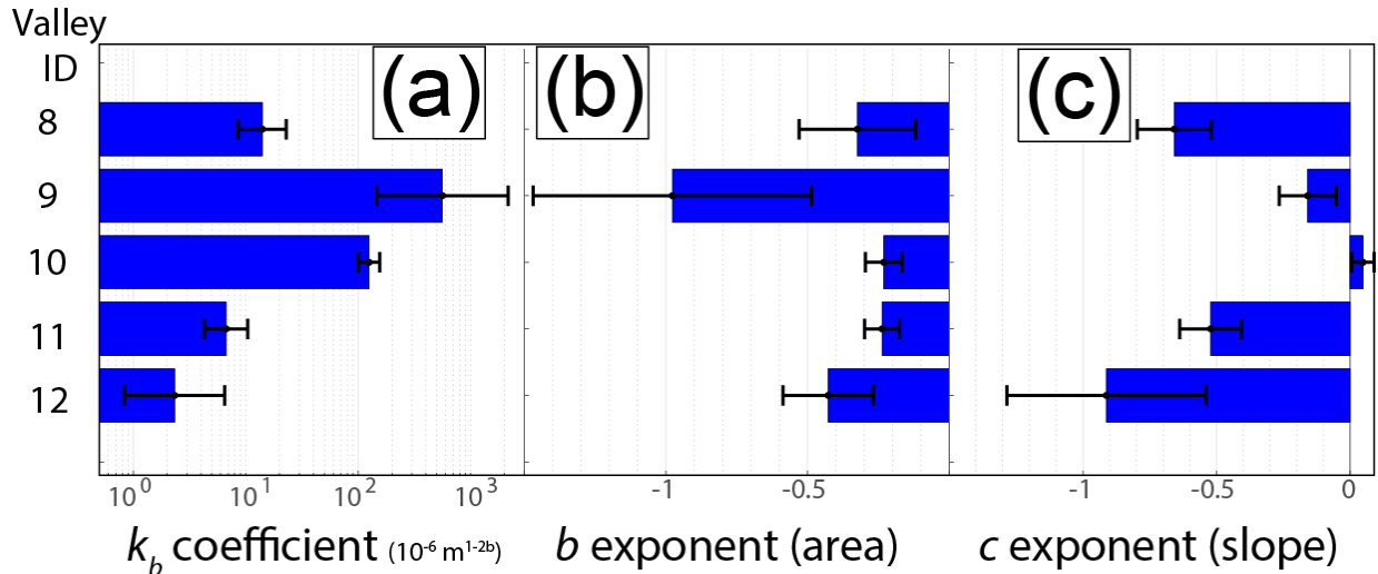
430 Figure 5: Bar plots of the k_b coefficient and b and c exponents in Eq. (2) for the reversed valley category (panels (a), (b), and 435 (c) respectively), fitted by multivariate regression. Error bars represent the 95% confidence interval. The k_b values show a large variability. The area exponents, b , are generally less negative than the d exponents fitted to Eq. (1) in Table (1) and Fig. (4). Except for valley 10, the slope exponents c have negative values. In valleys 8, 11, and 12, the c exponent is more negative than the area exponent, b , reflecting the key role of slope in reversed valley width prediction. Note the log-scale of the x-axis in panel (a).
