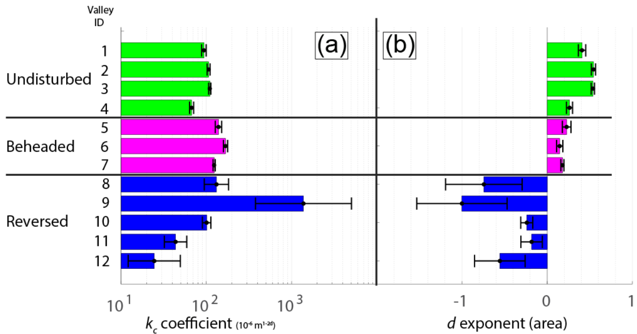
Figure 4: Bar plots of the k_c and d values (panels (a), (b), respectively) for valley sections of the categories defined in Fig. 1c. The error bars represent the 95% confidence interval. Unlike the k_c values, which lack a clear trend, the values of the d exponent (b) fall within a distinct range for each valley category. Note the log-scale of the x-axis in panel (a).
