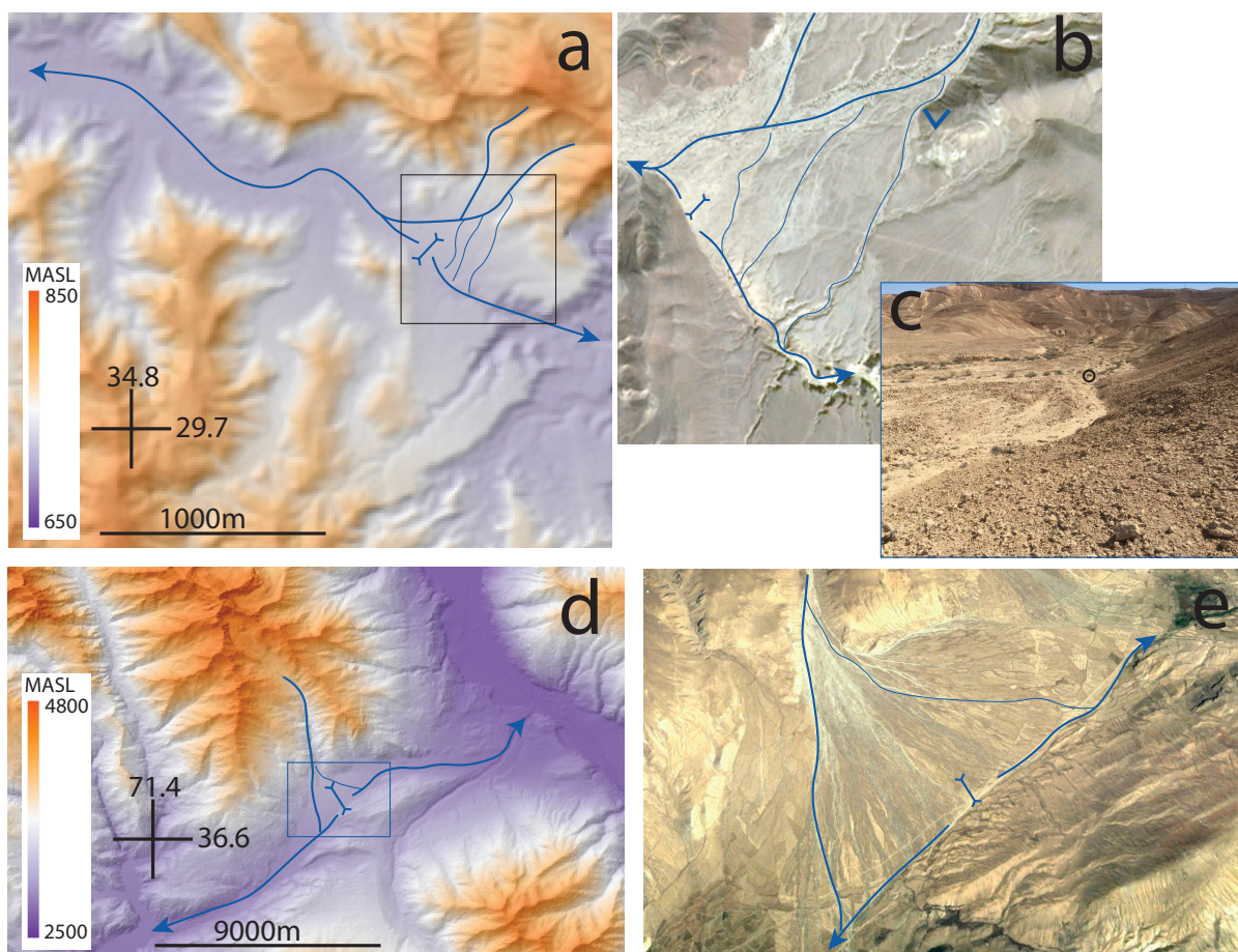
Figure 4. Examples of avulsions across windgaps (forked black line). Channels are marked in blue. (a) A map, based on a TanDEM-X DEM, of a windgap next to Mt. Berech in the Negev hilghlands along the Arava escarpment, Israel. Note that although the side tributaries marked in blue drain primarily north-west of the windgap, few bifurcating branches appear to route a fraction of the tributaries' discharge to the other side of the windgap. Black box marks the area shown in panel b. (b) An airphoto (©Google Earth 2020) showing the main channels of the side tributaries as well as their bifurcating branches. A black v-shaped symbol open to the north shows the locations from which the picture in panels c was taken. (c) View of an avulsion point looking upstream (north) from the aforementioned v-shaped symbol. Circle marks a backpack for scale, that is located at the bifurcation point. (d) A map, based on a GMTED2010 DEM, of the Ishkashim Pass area in Afghanistan. Note that although the side tributary (marked in blue) drains primarily south-west of the windgap, few bifurcating branches appear to route a fraction of its discharge to the other side of the windgap. Black box marks the area shown in panel e. (e) An airphoto (©Google Earth 2020) showing the bifurcation of a side tributary across the windgap.
