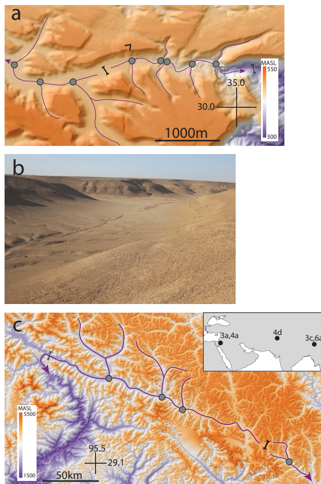
Figure 3. Examples of valleys with windgaps and major confluences with side tributaries (grey circles). Major channels are marked in blue and their flow direction is marked with an arrow. (a) A map, based on a TanDEM-X DEM, showing an example from wadi Grofit in the Negev highlands along the Arava escarpment, Israel. The current location of the windgap is marked by a bold forked black line. The approximated initial location of the windgap is marked with a thin forked black line ( Harel et al., 2019 ). A black v-shaped symbol open to the south-west shows the locations from which the pictures in panels b was taken. (b) A picture of the windgap shown in panel a, taken from the location of the aforementioned black v-shaped symbol towards south-west. (c) A map, based on GMTED2010 DEM, showing windgaps and confluences along the Parlung valley, China. The current location of the windgap is marked by a bold forked black line. A thin forked black line at the north-west portion of the map marks the approximate initial location of the windgap. In both the Grofit and Parlung examples, the windgap likely traversed confluences with side tributaries (grey circles), resulting in their barbed morphology, as it migrated to its current location. The inset map shows the general location of the field examples presented in this and other figures, figure numbers are specified next to each location.
