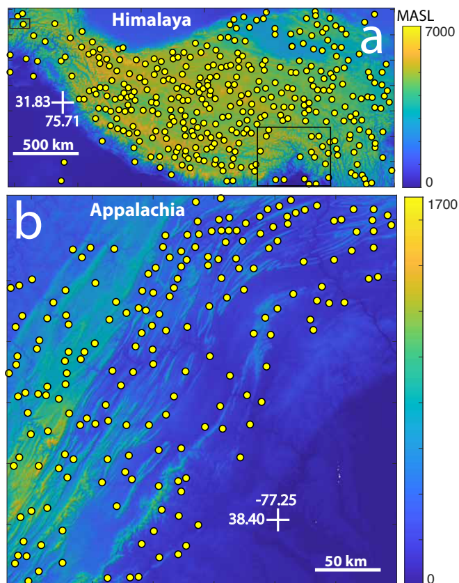
Figure 2. Windgaps in tectonically influenced areas. (a) A map of estimated windgap locations (yellow circles) in the Himalaya. The inset box at the bottom right marks the areas shown in figures 3c and 6, and the box at the upper left marks the area shown in Figure 4d-e. (b) A map of estimated windgap locations in the Appalachian fold-thrust belt. Windgaps locations were identified over GMTED DEMs ( Danielson and Gesch, 2011 ) by delineating the drainage divides associated with a channel network mapped with drainage area thresholds of 200 and 12.5 km 2 for the Himalayas and Appalachia, respectively (values hereafter are reported in the same order for these two areas). To identify major divides at relatively low topographic positions (i.e., windgaps) we isolated high order divides ( Scherler and Schwanghart, 2020 ), computed the local relief based on divide elevations within a radius of 30 and 5 km, respectively, and identified locations of minimal divide elevation within these radii. These radii are based on typical valley widths in these areas and are similar to the typical distance from divide to channel head based on the drainage area threshold that was used to define channels (scaled to distance via Hack's law). Of the locations of minimal divide elevation, we identified windgaps as locations with low along valley relief and high across valley relief, to do so, we identified locations of local divide relief that is higher than 200 and 100 m, respectively (i.e., common low-end reliefs for noticeable valleys in these areas), and a vertical elevation difference between the divide and closest streams (on each side of the divide) that is less than 20% of the local divide relief.
