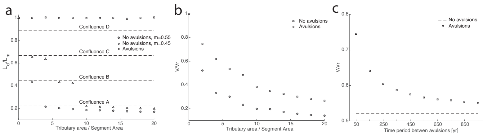
Figure 7. The influence of tributary area and avulsion frequency on windgap migration. (a) The influence of tributary area, and the value of the exponent m on the relative distance between the left boundary of the model domain and the stable windgap position. To account for tributary spacing and valley width, the drainage area of tributaries is normalized to the area of the valley segment between tributaries (i.e., Figure 5a). The windgap migration distance, L_d , is normalized by the distance, L_c , between the model boundary and the center of the model domain (5a-b), such that as the windgap migrates closer to this center, the value L_d/L_c is closer to unity. Note that stable windgap positions are typically next to a confluence on the victim channel whose location is marked by dashed horizontal lines, named A-D in accordance with Figure 5a. Note that when the trunk-tributary confluences are spatially fixed and the area of tributaries is relatively large, the windgap can attain a stable position relatively far from the center of the model domain, and that when avulsions are simulated, the windgap attains a stable position at the center of the model domain, similar to simulation without confluences where all nodes have the same drainage area. Also note that the distance to stable windgap locations varies with the value of the exponent m (here shown with m = 0.45 and m = 0.55 ). (b) The influence of tributary area (normalized as before) on the mean velocity of windgap migration. This velocity is computed based on the location and time of where/when the windgap reaches a stable position, and is normalized by the duration it takes for a simulation with an equal drainage area for all nodes but the same overall model drainage area (i.e., the local drainage area at each node is the mean area of all nodes for an equivalent model with confluences) to reach the same location. Note that the windgap migration velocity is highest in simulations with equal drainage area for all nodes, and is also higher in simulations with avulsions compared to those with no avulsions. (c) The influence of time interval between avulsion on the mean velocity of windgap migration (computed in the same procedure as described before), for the case where the area of tributaries is twice the segment area. The dashed line marks the velocity of an equivalent simulations without avulsions. The results plotted in panels a-c rely on a model configuration with 8 trunk-tributary confluences (4 at each side of the model center), 575 model nodes, \delta x = 100 m, w = 400 m, K = 1 \times 10^{-5} \text{ m}^{1-2m} \text{ yr}^{-1} , n = 1 , m = 0.45 , D = 0.24 \text{ m}^2 \text{ yr}^{-1} (for panel a also m = 0.55 , where D is set to D = 0.68 \text{ m}^2 \text{ yr}^{-1} to maintain a constant Péclet-based length scale with the model of m = 0.45 (i.e., Perron et al., 2009)).
