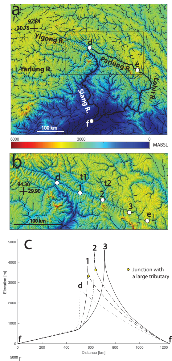
Figure 6. Simulated windgap migration along the Parlung valley. (a) A regional map, based on 15 arc-second GMTED2010 DEM (approximately 500 m resolution) showing the Yigong, Parlung, Lohit, Siang and Yarlung rivers (location is shown as a box in figure 2a). Reconstructions of a paleo-drainage pattern (Lang and Huntington, 2014; Govin et al., 2018; Zhang et al., 2019) suggest that the Yigong and Parlung used to drain southeast to the Lohit, until the Yigong was captured by the Siang river. This created a windgap at the top of the beheaded Parlung valley, just east of the capture point. The approximate capture location is marked by point d. Point e marks the current location of the windgap between the north-west flowing Parlung and south-east flowing Lohit rivers. Point f marks the confluence of the Lohit and Siang rivers. Thin dark lines mark river systems with drainage area larger than 10^8 m^2 , and the bold dark lines mark the river system that is simulated in panel c. A black rectangle marks the area shown in panel b. (b) Map of the Parlung river basin. The Parlung reversed its flow direction following the capture, likely through windgap migration from the capture point (point d) to the current location of the windgap (point e). As the windgap migrated, portions of the valley that used to drain eastward through the Lohit reversed their flow direction. Points 1, 2 and 3 mark simulated stable windgap locations in conjunction with panel c. The labels t1, and t2, mark large tributaries of the Parlung river. (c) Profiles of simulated initial and steady-state topography. The symbol f marks the model boundaries at the location of the Lohit-Siang confluence, as shown in panel a. The symbols d, 1, 2, 3, mark the windgap locations, in conjunction with panel b, for the cases of: d - a profile at the time of capture of the Yigong-Parlung by the Siang (the initial topography of the simulations); 1 - a profile of a simulated stable windgap position that develops after the Yigong-Parlung capture caused eastward windgap migration along the Parlung valley. Note that this stable location is just west of a confluence with a large tributary (t1). The confluence location is shown in panel b (point 1) and marked with a yellow circle on the topographic profile in panel c); 2 - a stable windgap position that developed by simulating an avulsion (i.e., shifting the confluence of tributary t1 to the aggressor's side of the windgap: left of the windgap location in profile 1). Note that this new stable windgap position is just west of a confluence with a large tributary t2 (the confluence location is shown in panel b and marked with a yellow circle on the topographic profile in panel c). 3 - a stable windgap position that is attained through avulsion simulation, where tributaries with drainage area larger than 10^7 m^2 are allowed to avulse. The simulations use the following parameters: n = 1 , m = 0.5 (e.g., Wang et al., 2017; Yang et al., 2018), \delta x = 500 m (i.e. in accordance with DEM resolution), D = 2 m^2 yr^{-1} , K = 7.96 \times 10^{-6} yr^{-1} , U = 0.005 m yr^{-1} .
