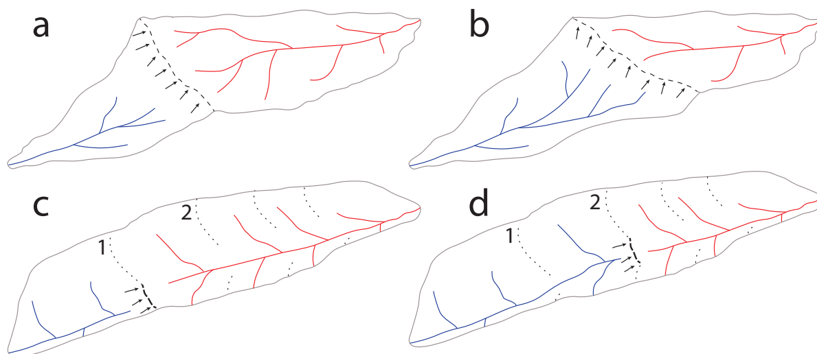
Figure 1. Schematic illustration of a typical (a,b) vs. along valley (c,d) divide migration. (a) Illustration of a typical divide migration process where the divide (dashed line) is located along a ridge line (after Whipple et al. (2017)). (b) The same setting as in panel a, after the divide migrated some distance. Note that as the ridge line migrates it erases the tributaries of the victim basin. (c) Illustration of a windgap (dashed line) migration along a valley. Note that the tributaries that drain to the valley can be preserved through the migration process, so that the migrating windgap can traverse confluences with tributaries through its migration. (d) Same setting as in panel c, after the windgap migrated some distance. Note that the low order drainage divides between tributaries (dotted lines) can merge with the migrating windgap to form a high order divide (for example see the low order divides marked 1 and 2 in panels c and d).
