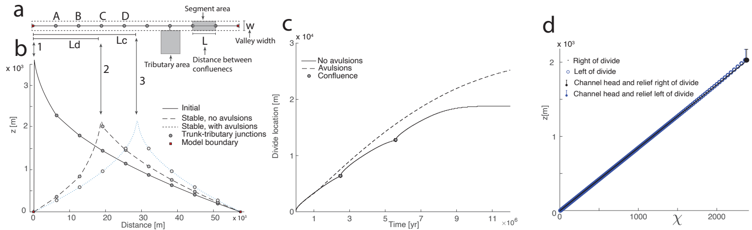
Figure 5. Simulations of along valley windgap migration across confluences with tributaries. (a) Plan view schematic of a 1-dimensional model domain that simulates a valley (valley boundaries marked by a dashed line) of constant width ( w ) that is drained by a trunk channel (dark line) with equally spaced ( L ) confluences with tributaries (grey circles). The drainage area of a segment between confluences is fixed ( L \times w , schematically represented by a grey rectangle). The drainage area of a tributary is the local area that is added at each confluence (an example is represented here by a grey rectangle). L_d and L_c mark the distance from the left edge of the model domain to the location of a stable windgap position and to the center of the model domain, respectively, and are referred to in figures 7 and 8. Confluences marked A-D are referred to in figure 7a. (b) An example of simulated topographic profiles along the trunk channel: (1) A topographic profile of the simulation's initial condition (solid line, trunk-tributary confluences marked by dark grey circles); (2) Simulated steady state topography that develops from the initial condition in profile #1 through a fixed confluences simulation (dashed line, trunk-tributary confluences marked by medium grey circles). Note that the windgap attains a stable position away from the center of the model domain (i.e., L_d < L_c ). Also note that this steady position occurs adjacent to a trunk-tributary confluence on the victim's side of the windgap; (3) Simulated steady state topography with avulsions (dotted line, light grey circles mark the mean location of trunk-tributary confluences - which is the same as that of the fixed confluences). (c) Simulated windgap location vs. time for the simulations in panel b. For the fixed confluences simulation (solid line), note the changes in windgap migration velocity (i.e., the gradient of the line in the figure) as the windgap migrates across tributary confluences (grey circles). Note that these changes in migration velocity are not apparent in a simulation with avulsions (dashed line) and that the overall windgap velocity is higher when avulsions are simulated. Note that the plot shows the model duration until the windgap in the fixed confluences simulation attained a stable position (case 2 in panel b), and that in the avulsions simulation the windgap continued migrating until it attained a stable position at the center of the model domain (case 3 in panel b, at a distance of about 30 km from the initial windgap location). (d) A \chi - z plot (Perron and Royden, 2013) for case 2 in panel b. The plot demonstrates that this windgap position is stable although it is not in the center of the model domain. Note that the relief from each channel head to the windgap is also marked (see legend). The channel head is defined based on where the topographic profile shifts from concave to convex. The channel head right of the divide (a black filled circle in the \chi - z plot) is at the adjacent tributary confluence (grey filled circle just right of the divide in profile 2, panel b). Panels a-d are based on a model configuration with 8 trunk-tributary confluences (4 at each side of the model center), 575 model nodes, node spacing: \delta x = 100 , confluence spacing: L = 6400 m, valley width: w = 400 m, tributary area equals 2 segment areas (i.e., 2 * L \times w ), hillslope diffusion coefficient: D = 0.24 \text{ m}^2 \text{ yr}^{-1} , exponents: n = 1 , m = 0.45 , channel erodibility: K = 1 \times 10^{-5} \text{ m}^{0.1} \text{ yr}^{-1} , time interval between avulsions 50 [yr].
