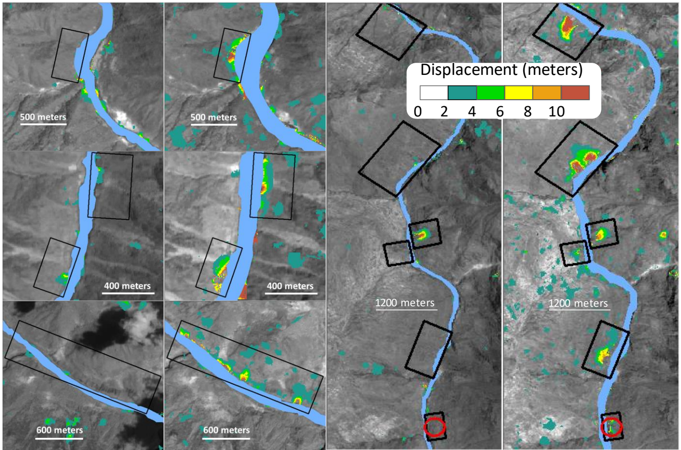
Figure 3. Moving slopes in four selected sections along the Jinsha River (a-d) before (2015.11-21-2018.11) and after (2018.11-21-2019.11) the Baige floods. Left The left subplots (a1, b1, c1, and d1) are pre-flood results, and the right subplots (a2, b2, c2, and d2) are post-flood results. MD is short for the village-Mindu village. The background images are cloud-free grey-scale Sentinel-2 images before and after the 2018 floods. The red circles indicate concurrent landslides, and the black squares are slope slippages.
