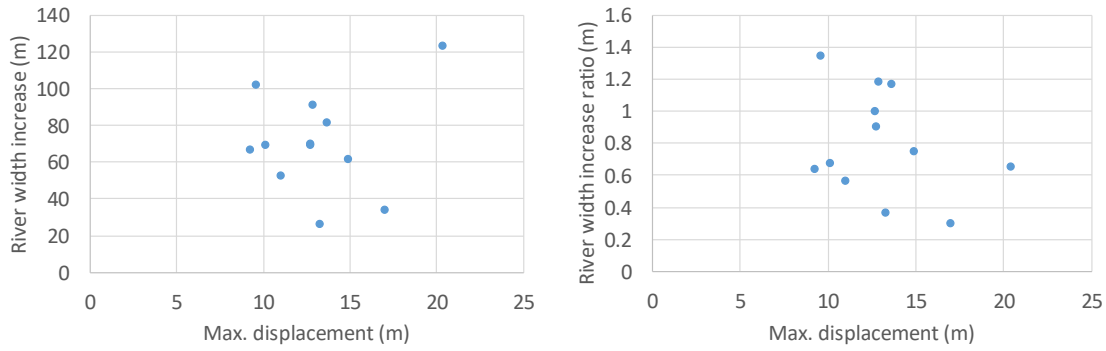
Figure 8. The r Relation between measured maximum slope displacements and river width increase (a) and rate of river width increase rate (b).
