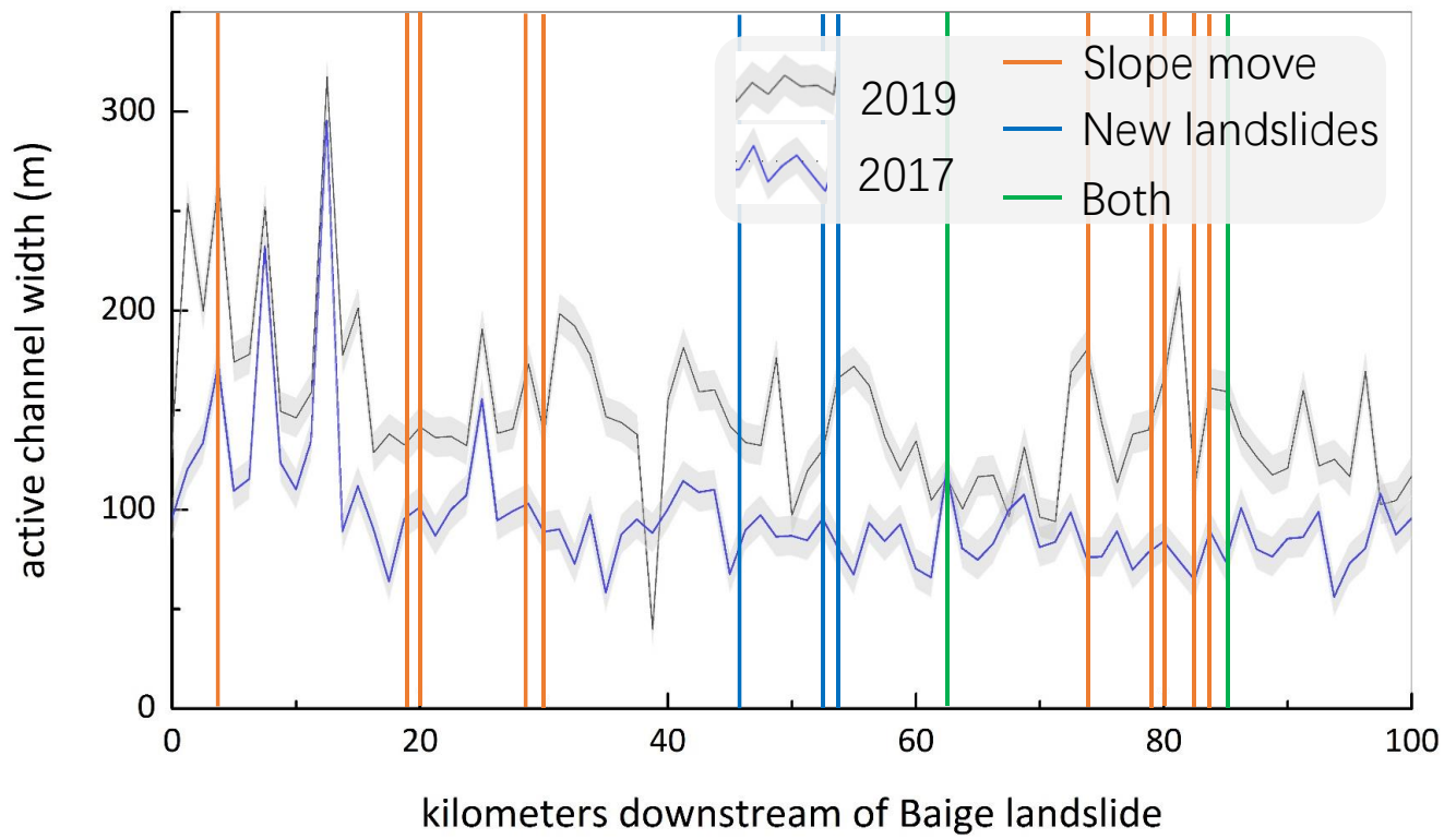
Figure 6. River widths before and after the Baige floods. The greygray shading indicates an uncertainty of \pm 1 pixel in the Sentinel-2 imagery.
