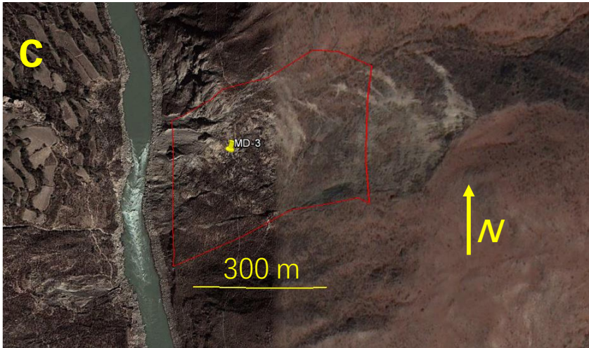
Figure 9. Tensile cracks of on major hillslopes before the 2018 Baige floods as seen from shown by high-spatial-resolution images from © Google Earth.
