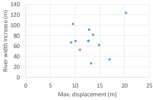
390 Figure 8. Relation between measured maximum slope displacements, river width increase (a) and rate of river width increase (b).
