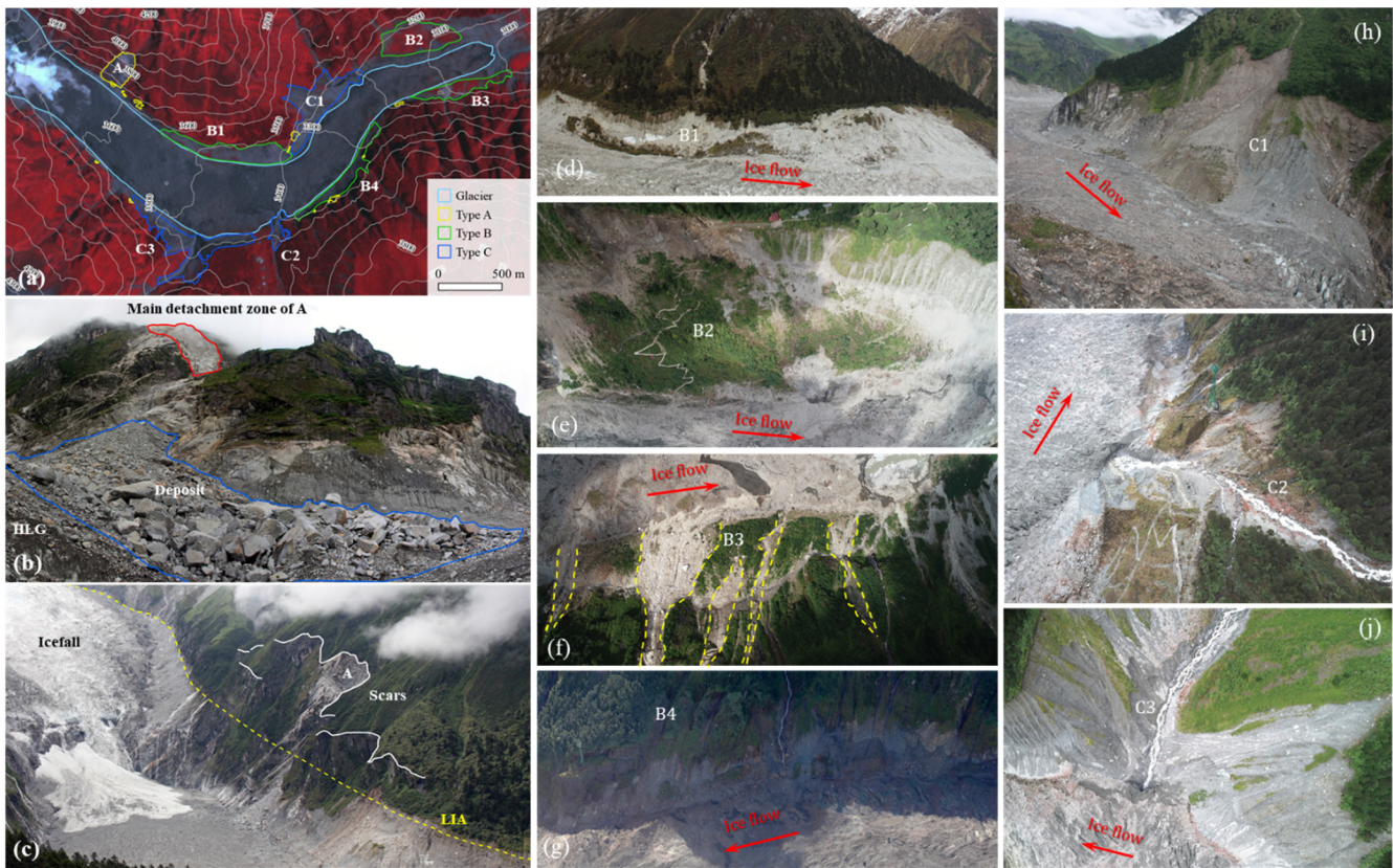
Figure 5: (a) The distribution of three type of PSFs based on Landsat image. (b) The particulars of type A failures in the upper part of the HLG's ice tongue. Main detachment zone (red), Deposit (blue). (c) The scars (white lines) surrounding the rockfall A. Subplots (d, e, f, and g) and (h, i and j) are closer photographs of Type B and Type C failures, respectively, field photo by Qiao Liu.
