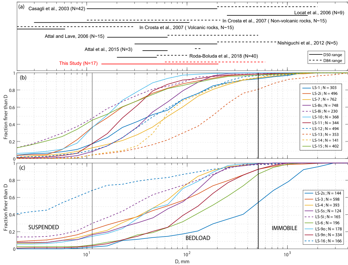
Figure 2. (a) range of D_{50} and D_{84} for various studies, excluding the coarsest and finest distributions of each study. (b) and (c) cumulative distribution function for the 16-17 sampled landslide deposits. For visibility, panels (b) and (c) show surface and inner distributions best fit by a log-normal distribution for LS-5, LS-8 and a Weibull distribution LS-2, respectively. Note that LS-16 is poorly fit by both and thus 20 distributions in total. For visibility some lines are dashed and the distribution are shown in two panels. Vertical lines are approximate boundary for grain transport by suspension and bedload, for a flood associated with fluid shear stress of 220 Pa (see section Implications for sediment transport).
