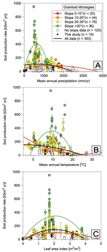
915 Figure 4: Soil production rates from this study (blue diamonds) and other studies in hillslopes with granit lithologies versus: A) Mean annual precipitation, B) Mean annual temperature, and C) Leaf area index. Data are separated in slope bins and plotted with a binomial fit. Curves shown in subplot were calculated with polynomial regressions through the data to help visualize the trend in observations for locations with different hillslope angles.
