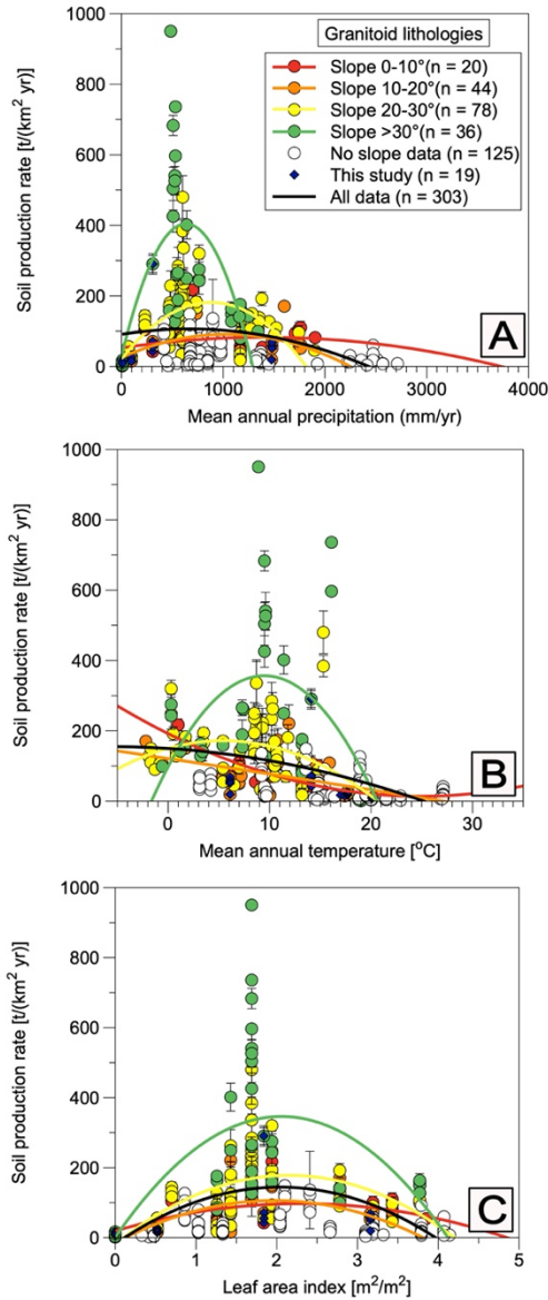
Figure 4: Soil production rates from this study (blue diamonds) and other studies in hillslopes with granit lithologies versus: A) Mean annual precipitation, B) Mean annual temperature, and C) Leaf area index. Data are separated in slope bins and plotted with a binomial fit. Curves shown in subplot were calculated with polynomial regressions through the data to help visualize the trend in observations for locations with different hillslope angles.
