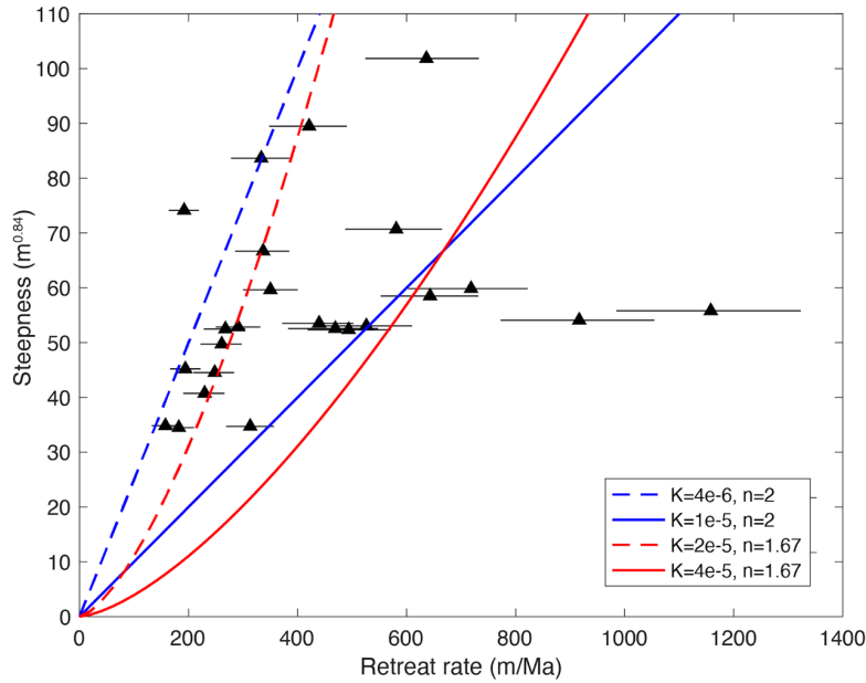
Figure 15 Channel steepness against escarpment retreat rates with 1\sigma uncertainty for catchments in the Western Ghats. Retreat rates of the escarpment are calculated using the Basin Projection method with an azimuth of N57E. Lines are model prediction of steepness and retreat rates from Eq. (2) for a range of the slope exponent n and K where the dimensions of K are m^{1-0.84n}/yr .
