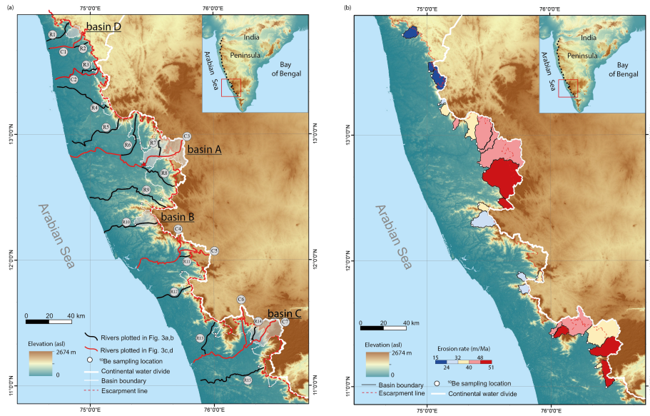
Figure 2 (a) Topographic map of the southern Western Ghats escarpment in India (location is indicated in the inset figure). The black dashed line denotes the escarpment defining the Western Ghats, and we take the southern limit of the Deccan Traps as the boundary between the northern and southern segments. The 10 Be sample locations of Mandal et al. (2015) are indicated by grey circles. (b) Cosmogenic 10 Be-derived erosion rates. Erosion rate is recalculated from the published concentrations following the method of Lupker et al. (2012). See Table 1 for the data.
