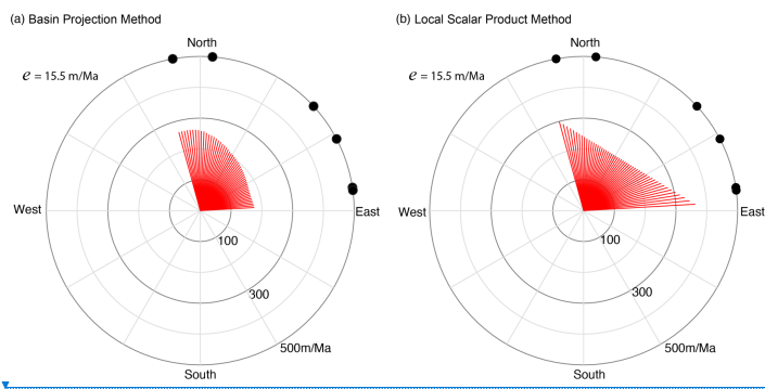
645 Figure 9 Escarpment retreat rate as a function of azimuth of a horizontal mass flux vector using (a) the Basin Projection Method; (b) the Local Scalar Product Method. Basin is from the Western Ghats with location indicated as Basin D in Fig. 2. Measured ^{10}\text{Be} concentration is 172426 ( \pm 8125 ) atoms/g and corresponds to a mean vertical erosion rate of 15.5 m/Ma. The azimuth of the tangential red lines denotes the assumed escarpment retreat direction, and the length of the radial vector is the consequent retreat rate for that direction and the measured ^{10}\text{Be} concentration. Black dots are orientations of characteristic tributaries of the escarpment-draining channels of this basin.
