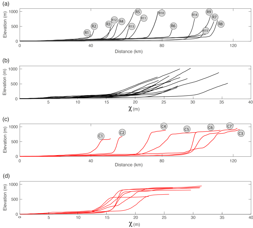
170 Figure 3 River profiles and corresponding transformed \chi profiles in the south Western Ghats. Locations of these rivers are indicated in Fig. 2a. Rivers are extracted from 90 m SRTM data and use a threshold drainage area of 1 km 2 . The \chi value of rivers is calculated using a base level of sea level, concavity of 0.42 and precipitation is not included. (a-b) Profiles of escarpment rivers that initiate from the escarpment. (c-d) Profiles of escarpment rivers that initiate from the plateau interior and drain through the escarpment.
