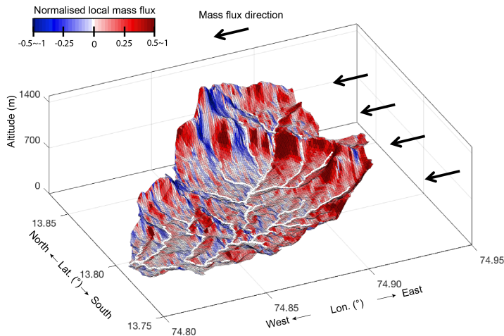
610 Figure 8 Local mass flux of elemental surfaces of an escarpment-draining basin in Western Ghats. Basin location is indicated as Basin D in Fig. 2 and is also shown in Fig. 6. The basin surface is discretized into elemental surfaces and colour-coded with the relative magnitude of the local mass flux for a horizontal rock velocity in the direction indicated. Flux is normalized to the catchment-averaged mass flux. Thick white lines are channels extracted from the DEM for a minimum drainage area of 1 km 2 .
