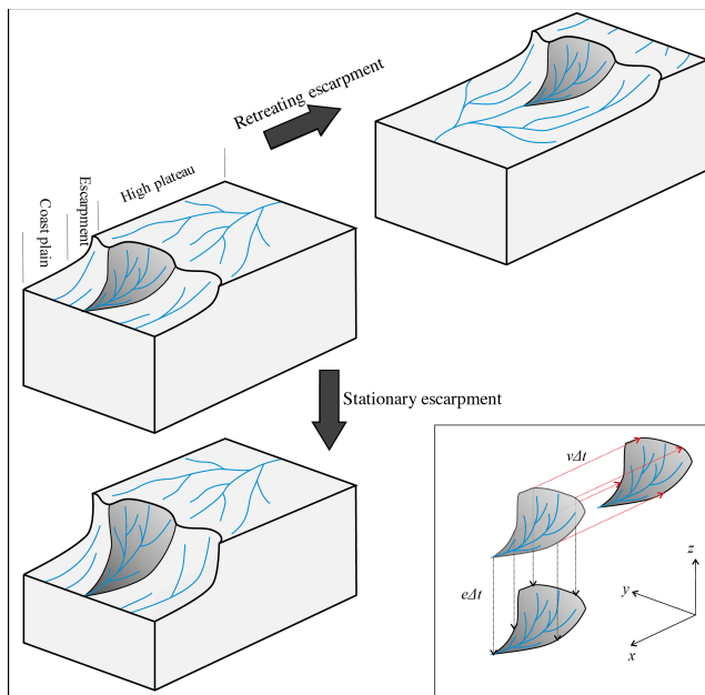
90 Figure 1: Conceptual diagram showing two scenarios of escarpment evolution: a retreating escarpment or a down-cutting escarpment with stationary water divide. The grey surface denotes the surface of an elemental escarpment-draining catchment.
