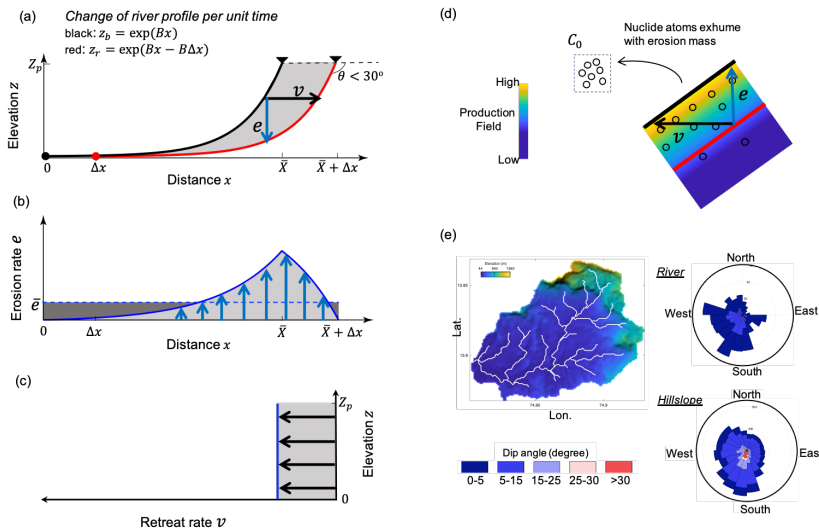
535 Figure 7 Relationship between mass flux through a surface and the velocity for a retreating escarpment. (a) Land surface, assumed to be exponential in form, retreating into a pre-existing highland at constant velocity, v . The surface lowering at any point is given as e . (b) Surface lowering rate as a function of distance. (c) Horizontal velocity as a function of elevation. Velocity is constant in both elevation and distance. Area under the curves (light and dark grey) in (a), (b) and (c) represents the mass flux and is equal in all cases. (d) ^{10}\text{Be} production zone below a dipping surface. Rock motion in either vertical or horizontal direction brings particles to the surface with an integrated production. For a constant flux, v and e scale so that the time of passage through the production zone is independent of direction, so surface concentration is independent of direction. (e) Elevation of a typical catchment in the Western Ghats with rose diagrams showing frequency and magnitude of slope with direction for channels (upper) and hillslopes (lower).
