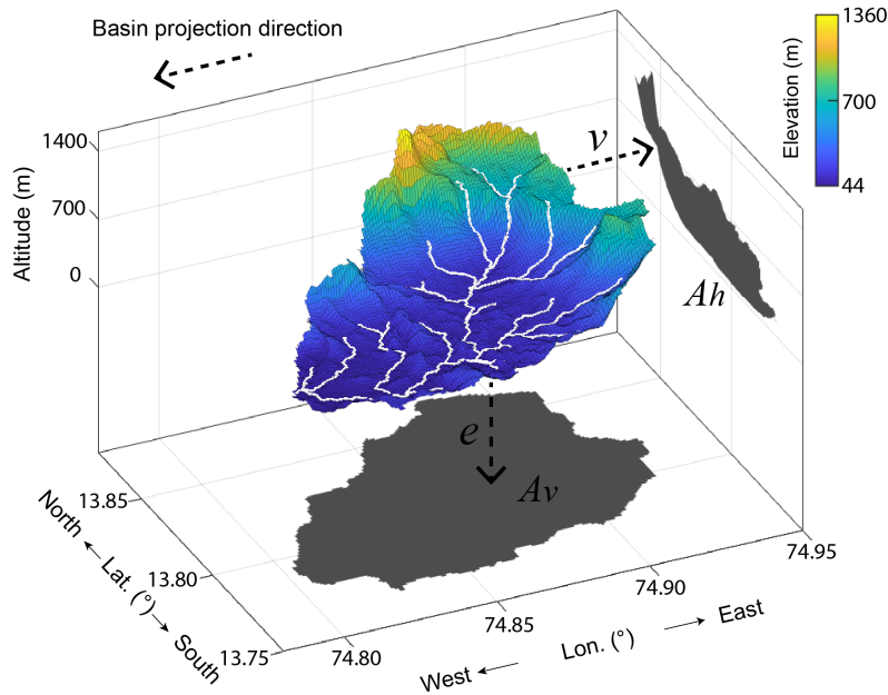
490 Figure 6 Depiction of the flux of mass through the surface of a drainage basin from the coastal escarpment of the Western Ghats, India. Basin position is indicated as basin D in Fig. 2. Spatial surface of drainage basin and its projection in the vertical and a horizontal direction. Projected areas are A_v and A_h , respectively. Thick white lines denote channels extracted from the DEM for a minimum drainage area of 1 km 2 .
