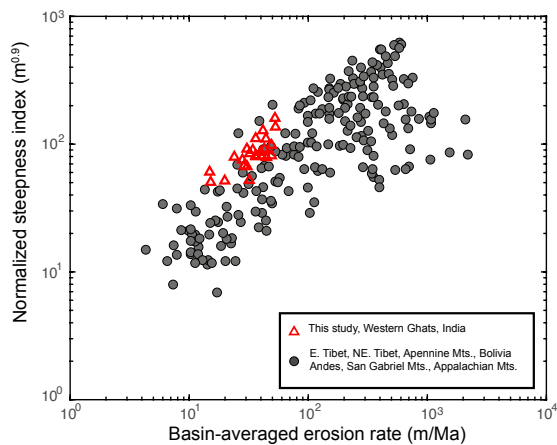
250 Figure 5 Normalised channel steepness index and cosmogenic ^{10}\text{Be} -derived basin-averaged erosion rates from the Southern Western Ghats (red-lined triangles) with comparison to a compilation of global data by Kirby and Whipple (2012) (grey dots). The steepness of Western Ghats rivers are from slope-area analysis using a uniform concavity of 0.45 to be consistent with the global data.
