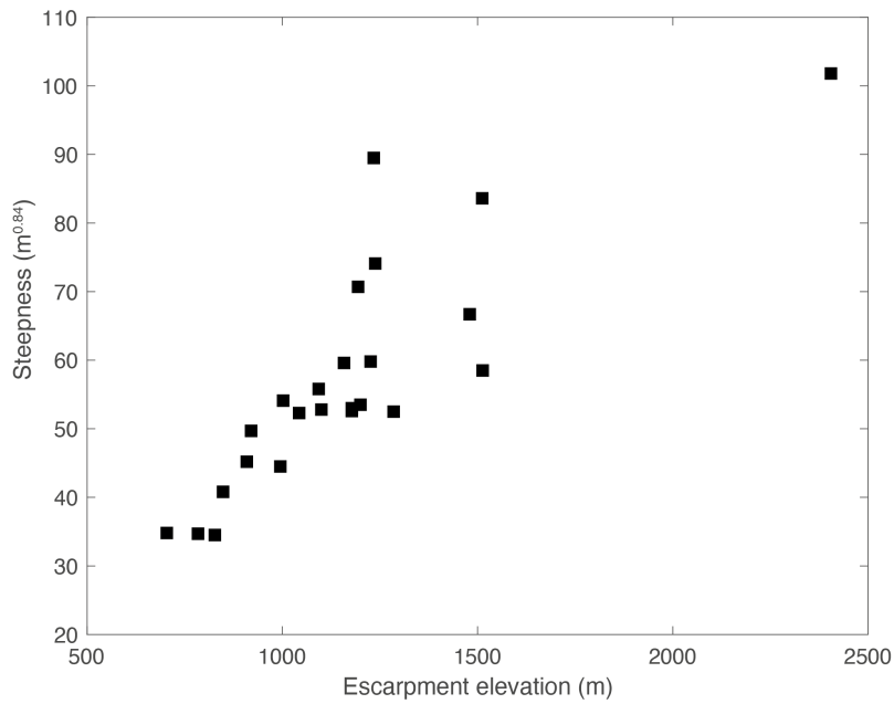
770 Figure 14 Relationship between channel steepness and escarpment height in the Western Ghats. The channel steepness is calculated from slope-area plots using a uniform concavity of 0.42. Correlation is consistent with the theory that morphology has evolved to erode pre-existing topography at a constant rate of retreat. See Table 1 for the data.
