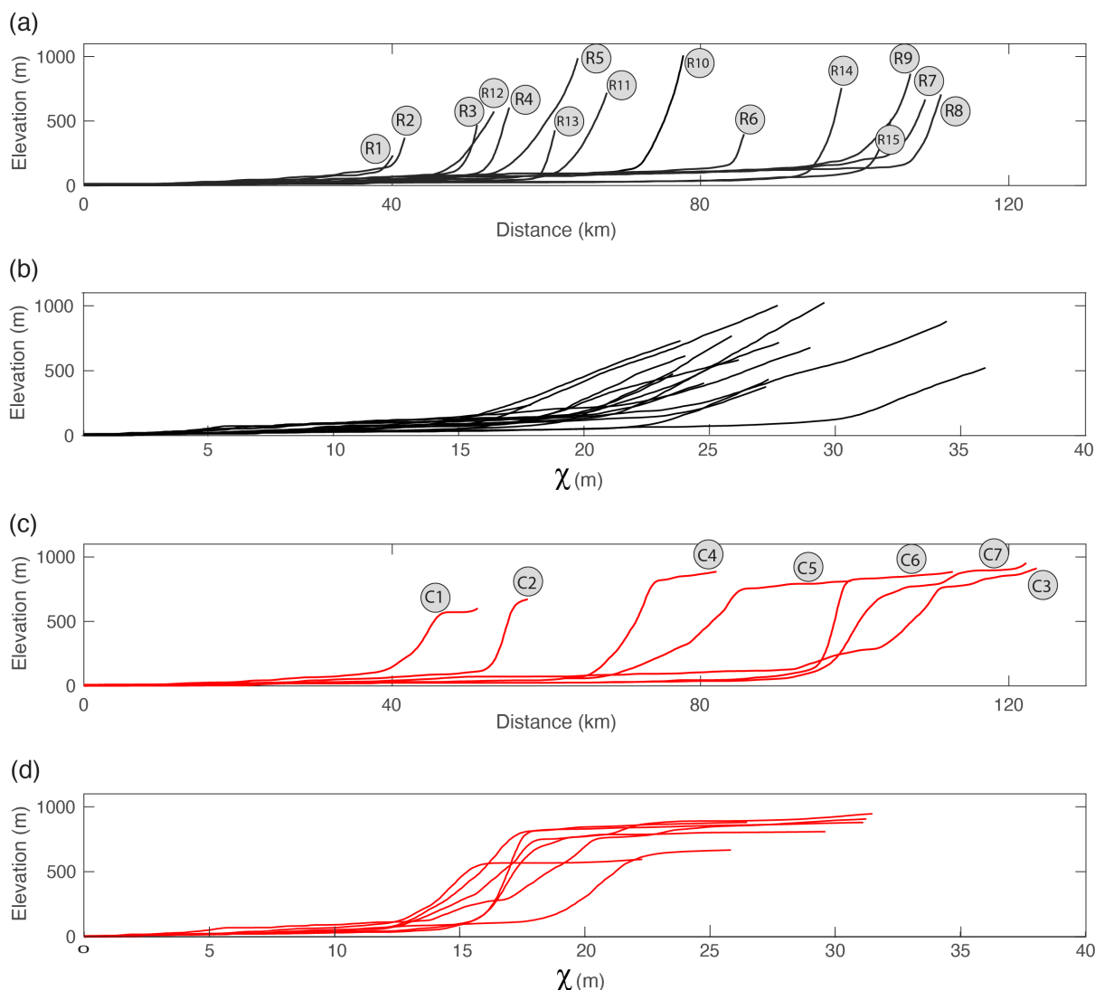
145 Figure 3 River profiles and corresponding transformed \chi profiles in the south Western Ghats. Locations of these rivers are indicated in Fig. 2a. Rivers are extracted from 90 m SRTM data and use a threshold drainage area of 1 km 2 . The \chi value of rivers is calculated using a base level of sea level, concavity of 0.42 and precipitation is not included. (a-b) Profiles of escarpment rivers that initiate from the escarpment. (c-d) Profiles of escarpment rivers that initiate from the plateau interior and drain through the escarpment.
