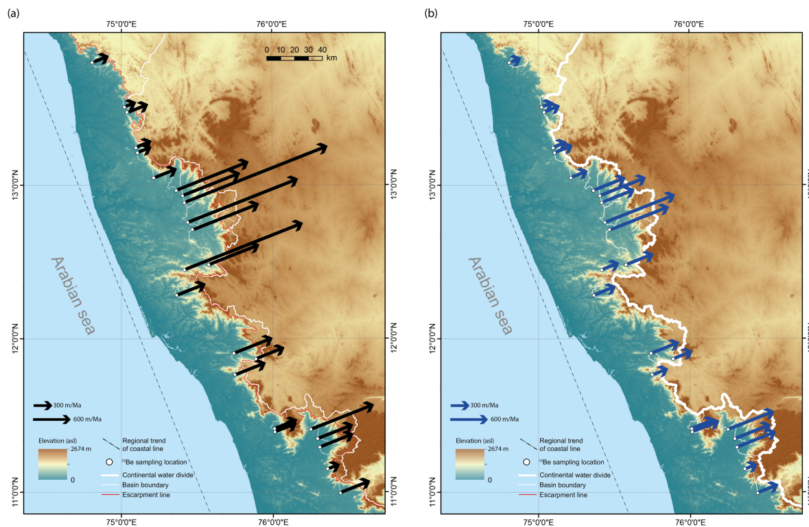
535 Figure 11 Escarpment retreat rates in the normal direction of the reference coastal line on the topography base map of southern Western Ghats. Rates from (a) the Local Scalar Product method and (b) from the Basin Projection method. Arrows represent the escarpment retreat vector: the azimuth denotes the retreat direction while the length denotes the retreat rate in that direction. The black dashed line indicates the trend of the modern coastline and escarpment.
