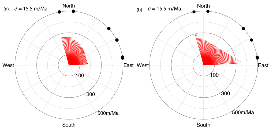
460 Figure 9 Escarpment retreat rate as a function of azimuth of a horizontal mass flux vector using (a) the Basin Projection Method; (b) the Local Scalar Product Method. Basin is from the Western Ghats with location indicated as Basin D in Fig. 2. Measured ^{10}\text{Be} concentration is 172426 ( \pm 8125 ) atoms/g and corresponds to a mean vertical erosion rate of 15.5 m/Ma. The azimuth of the
