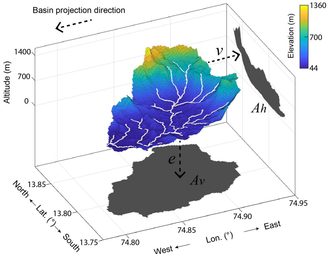
Figure 6 Depiction of the flux of mass through the surface of a drainage basin from the coastal escarpment of the Western Ghats, India. Basin position is indicated as basin D in Fig. 2. Spatial surface of drainage basin and its projection in the vertical and a
