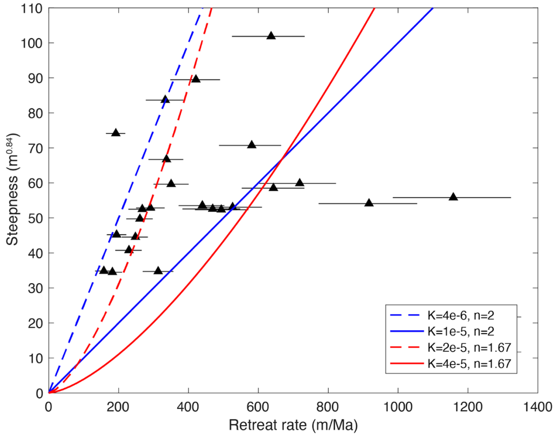
560 Figure 14 Channel steepness against escarpment retreat rates for catchments in the Western Ghats. Retreat rates of the escarpment are calculated using the Basin Projection method with an azimuth of N57E. Short solid lines indicate 1 \sigma uncertainty of retreat rates. Lines are model prediction of steepness and retreat rates from Eq. (2) for a range of the slope exponent n and K where the dimensions of K are \frac{m^{1.84-0.84n}}{yr} .
