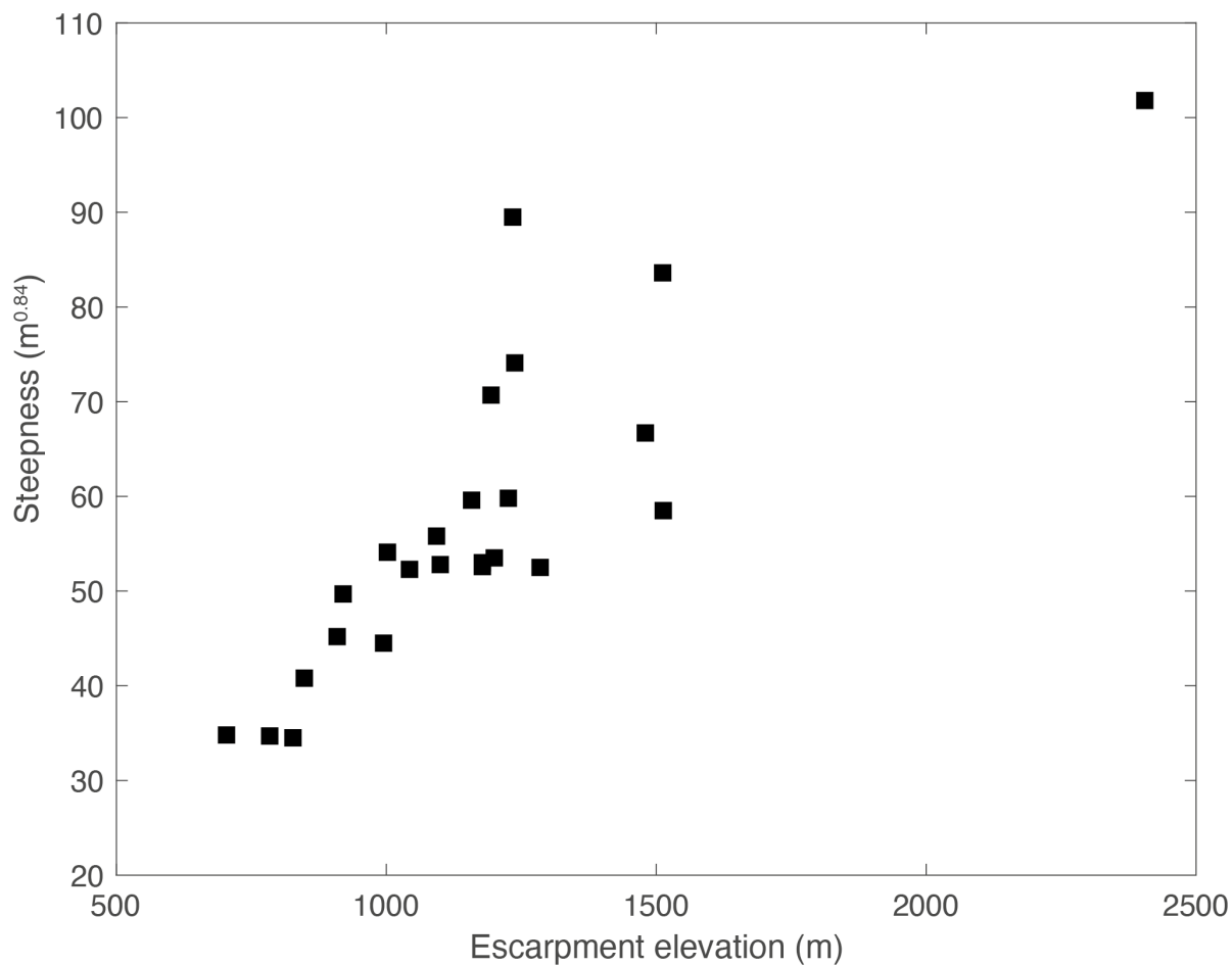
555 Figure 13 Relationship between channel steepness and escarpment height in the Western Ghats. The channel steepness is calculated from regression of slope-area plots using a uniform concavity of 0.42. Correlation is consistent with the theory that morphology has evolved to erode pre-existing topography at a constant rate of retreat.
