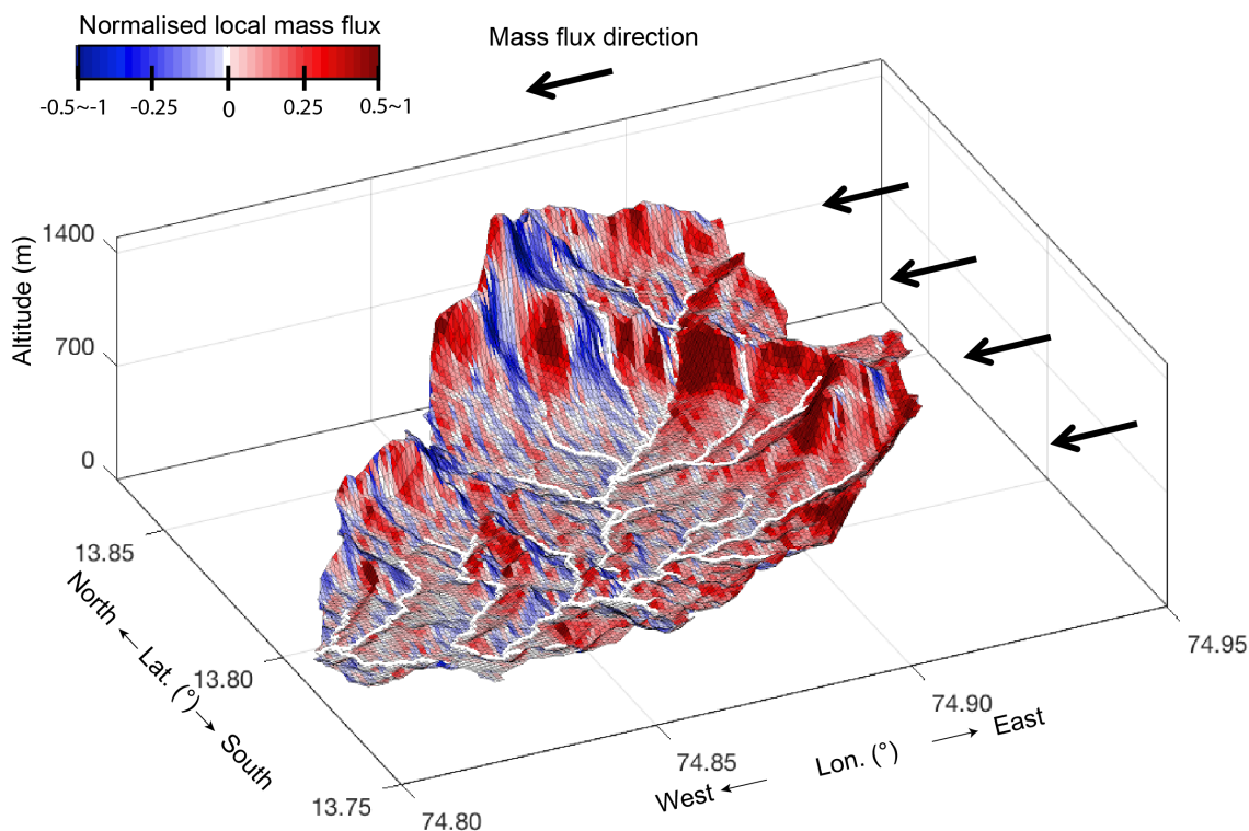
435 Figure 8 Local mass flux of elemental surfaces of an escarpment-draining basin in Western Ghats. Basin location is indicated as Basin D in Fig. 2 and is also shown in Fig. 6. The basin surface is discretized into elemental surfaces and colour-coded with the relative magnitude of the local mass flux for a horizontal rock velocity in the direction indicated. Flux is normalized to the catchment-averaged mass flux. Thick white lines are channels extracted from the DEM for a minimum drainage area of 1 km 2 .
