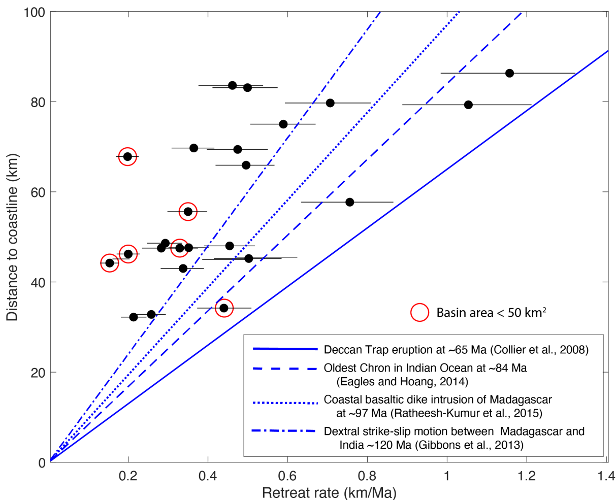
540 Figure 12 Current distance from the coastline against inferred retreat rate of Western Ghats escarpment basins from detrital ^{10}\text{Be} concentrations with 1\sigma uncertainty. Retreat rates of the escarpment are calculated using the Basin Projection method with azimuth taken as N57E. See Table 2 for the data. Age of rifting is constrained by various events as indicated and is expected to be at older than these constraints. Basins smaller than 50\text{ km}^2 are indicated with open red circles.
