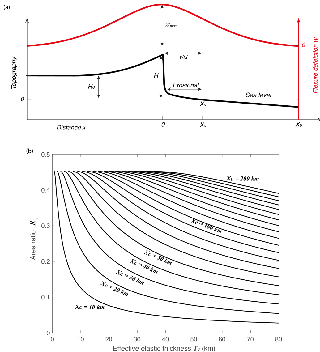
Figure 15 (a) Schematic model of isostatic flexural uplift due to escarpment erosion and retreat. Flexural uplift is calculated assuming removal of mass v\Delta t treated as a line load at x = 0 ; (b) Area ratio showing vertical erosion of coastal plain not accounted for in our horizontal retreat model. Ratio represents an overestimate of our retreat rates and is up to a few tens of percent at small T_e if sample is taken distant from escarpment.
