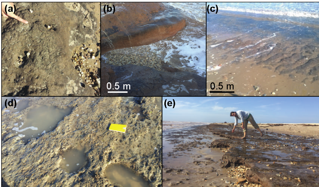
475 Figure 2: a) Wetting and drying on the cliff. b) Focused abrasion creating embayment at the cliff face. c) Focused abrasion creating runnels on the shore platform . d) Potholing and pothole coalescence on the shore platform. e) Differential erosion and abrasion leading to production of a decimeter scale step on the shore platform.
