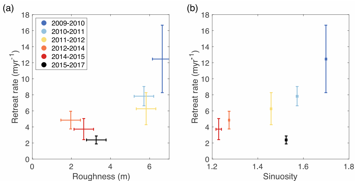
Figure 7: a) Mean roughness of the second shoreline being differenced vs. mean cliff retreat rate. b) Sinuosity of the second shoreline being differenced vs. mean cliff retreat rate.
