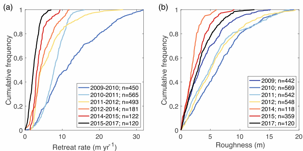
455 Figure 5: a) Cumulative distribution function of retreat rate for each time interval. b) Cumulative distribution function of cliff roughness for each time interval.
