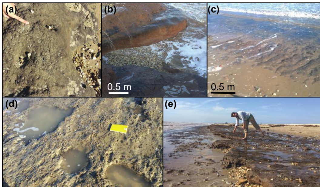
Figure 3: a) Wetting and drying. b) Focused abrasion creating embayment at the cliff face. c) Focused abrasion creating runnels. d) Potholing and pothole coalescence. e) Differential erosion leading to production of a decimeter scale step.
