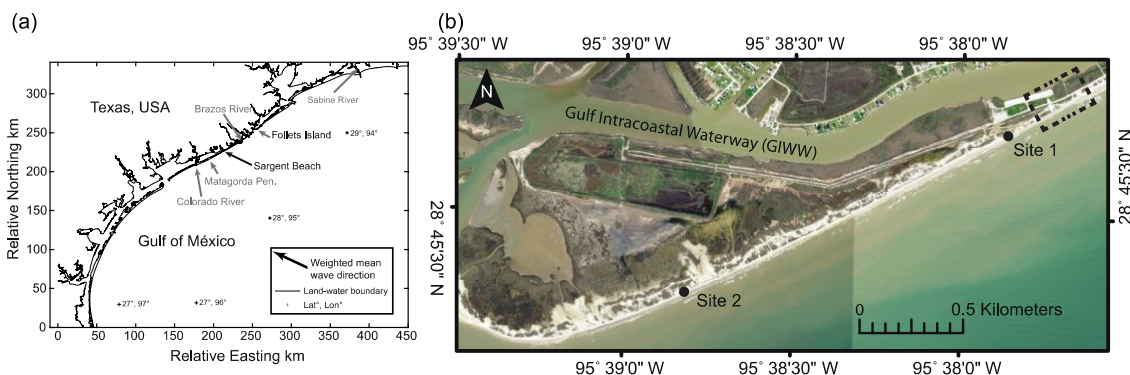
440 Figure 1: a) Regional map of the Texas coast showing the location of Sargent Beach. b) Aerial image of two survey sites at Sargent Beach, Texas. Site 1: sea cliff. Site 2: wave-cut platform. The dashed box represents the area where there is the least amount of land between the open ocean and the GIWW.
