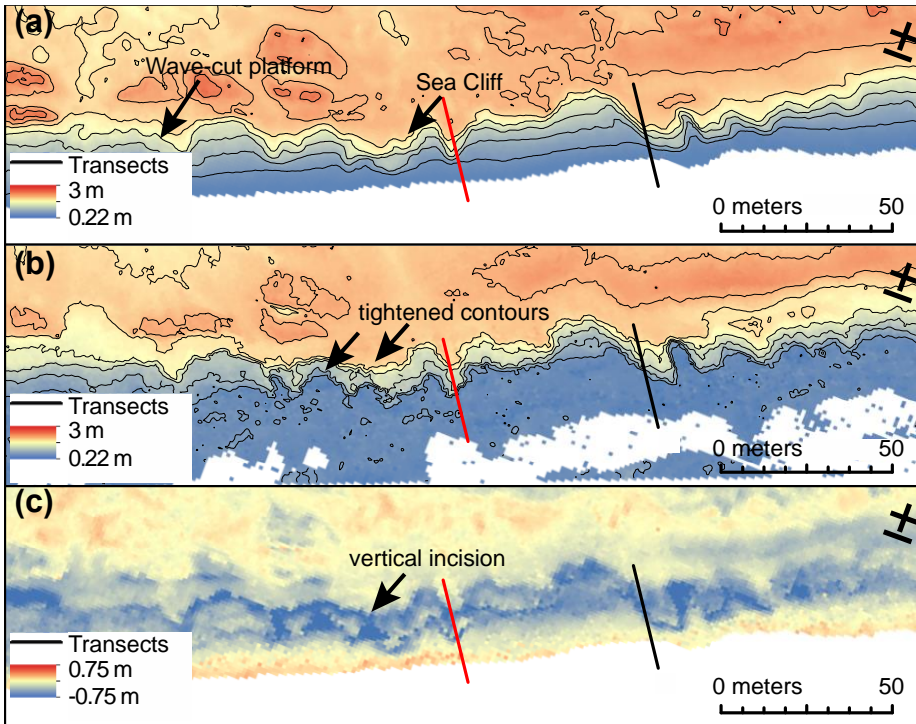
Figure 9: a) 2016 Lidar collected by the USACE at Site 1. Contour interval is 0.3 m. Transects are indicated by the black solid lines. Arrows point to location on the beach where elevation and contour spacing indicate either the sea cliff or the wave-cut platform. b) 2017 Lidar collected after Hurricane Harvey ©Bureau of Economic Geology. Contour interval is 0.3 m. Transects are indicated by the black solid lines. c) Difference between a) and b). The arrow points to the site of vertical incision.
