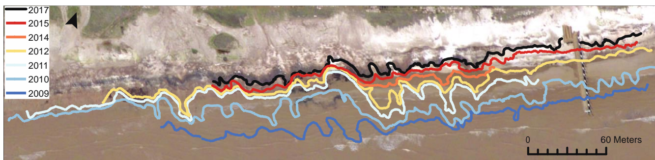
450 Figure 4: Plan-view of shorelines delineated from subsequent ~annual aerial images. Site 1 (see Fig. 1). Arrow points north. Image source: NOAA. Hurricane Harvey: Emergency Response Imagery of the Surrounding Regions. 2017.
