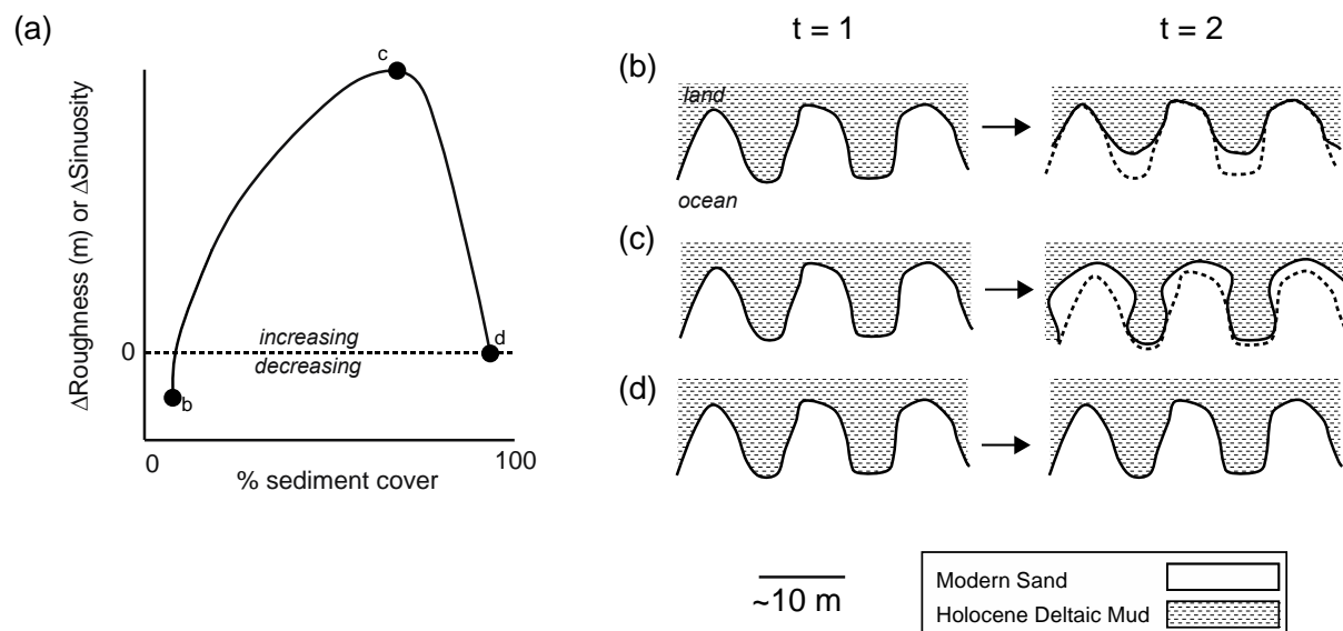
480 Figure 11. a) Conceptual diagram of relationship between change in cliff roughness or sinuosity with sediment cover percentage. Positive represents increasing roughness or sinuosity and negative represents decreasing roughness or sinuosity. Planview conceptual diagrams of cliff face erosion when b) no sediment cover, c) intermediate sediment cover, or d) 100% sediment cover. Dashed line represents t = 1 cliff face. Land is at the top and ocean is at the bottom for each panel.
