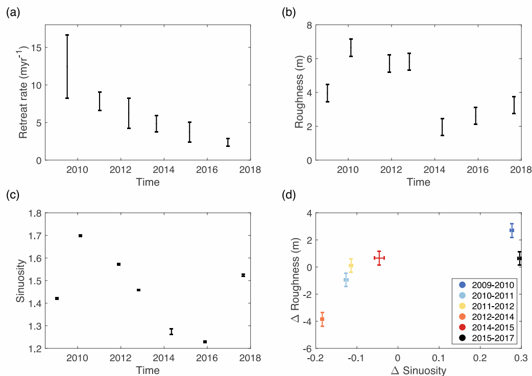
Figure 6: a) Mean cliff retreat rate ( \text{m yr}^{-1} ) through time. b) Mean cliff roughness (m) through time c) Mean cliff sinuosity through time. d) Change in cliff sinuosity vs change in cliff roughness. Error bars represent propagated error.
