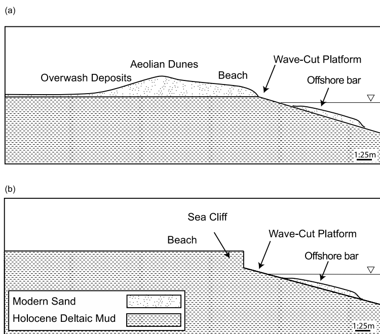
445 Figure 2: a) Generalized cross section of wave-cut platform. b) Generalized cross section of wave-cut platform and sea cliff system. ~1:25 m vertical exaggeration.
