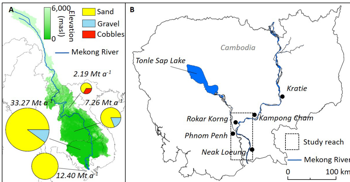
435 Figure 1: A) Established sediment extraction rates (Mt yr -1 ) across the Mekong River basin in 2013. The composition and volume of material extracted are disaggregated by country taken from Bravard et al. (2013). The size of the pie charts scales with the volume extracted. B) Location of the study reach in Cambodia (dashed box) from Kampong Cham to the Vietnamese border.
