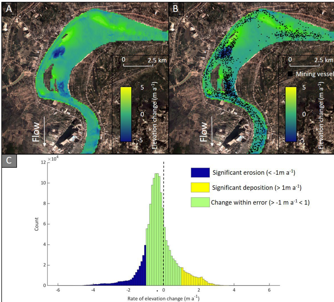
470 Figure 7: A) Rate of elevation change between 2013 and 2019 of the Mekong River near Rokar Korng highlighting areas of erosion (blue) and deposition (yellow). B) Overlay on the map depicted in A are the locations of all observed mining vessels during the period 2016 to 2020 demonstrating that the zones of greatest erosion observed in A correspond to areas of high mining activity. C) Histogram of elevation changes for this reach between 2013 and 2019. The median rate of bed elevation change is -0.25 \text{ m yr}^{-1} (mean elevation change is -0.16 \text{ m yr}^{-1} ). The dashed line demarks zero net change in elevation. Image background in panels A and B are 475 PlanetScope monthly composite scenes from December 2020 (Planet Team, 2018).
