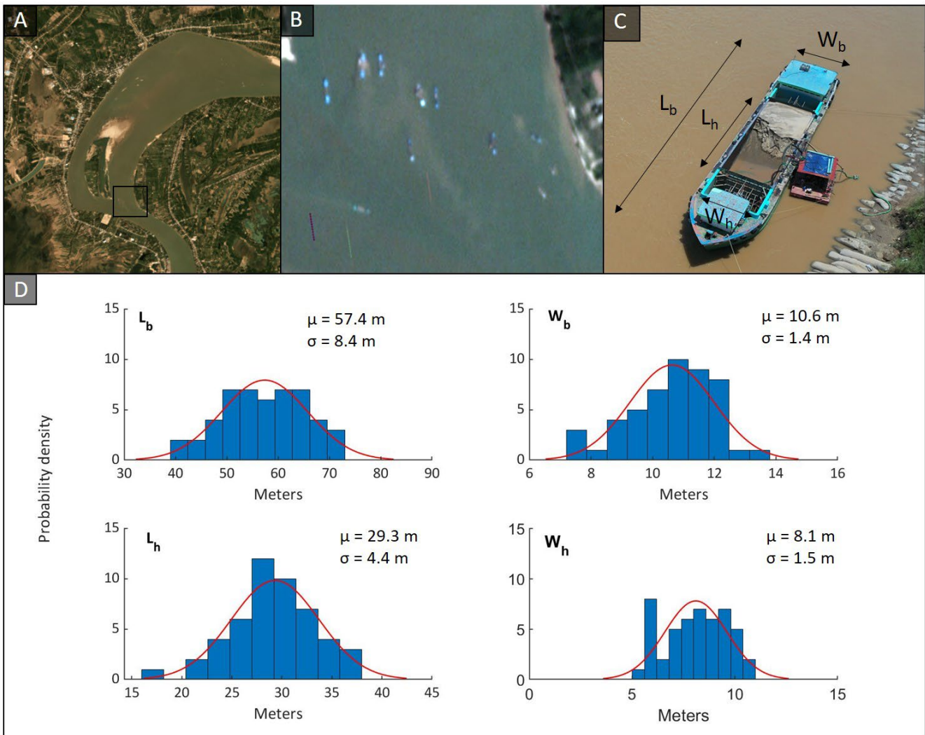
440 Figure 2: A) Example PlanetScope monthly composite image of a stretch of the Mekong river from December 2018 (Planet Team, 2018). The square highlights the area depicted in panel B. B) Zoomed in area of PlanetScope imagery (Planet Team, 2018) for the Mekong showing how mining vessels are identifiable within the satellite imagery. C) Dimensions of mining vessels recorded including the boat length ( L_b ), the boat width ( W_b ), the hold length ( L_h ) and the hold width ( W_h ). These latter two dimensions are important for the calculation of extraction volumes as they define the volume of sand each boat can transport when fully laden. Image is the authors own. D) Estimated dimensions of the mining vessels active on the Mekong taken from Google Earth imagery. 50 boats were measured and dimensions were recorded as depicted in panel C.
