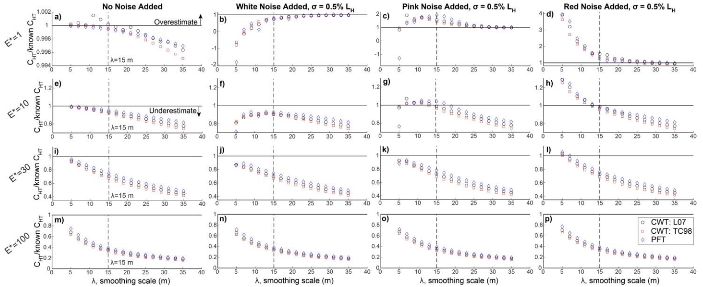
Figure 10: Ratio of C_{HT} of synthetic hillslopes where E^*=1, 10, 30, and 100 measured at various smoothing scales, \lambda , with: no noise added (first column), \sigma=0.5\% L_H white noise (second column), pink noise (third column), and red noise (Brownian) noise (fourth column). Ratio of C_{HT} is quantified as the quotient of the C_{HT-w} or C_{HT-p} and the model-specified C_{HT} . Black horizontal line in each panel corresponds with where the measured C_{HT} equals the actual synthetic C_{HT} (i.e. ratio=1). Points that plot above the line correspond with locations where C_{HT} is overestimated (sharper hilltops than expected); points that plot below are underestimations (broader hilltops than expected). See text for details but note systematic underestimation of C_{HT} as E^* increases, even for the surface with no added noise. Dashed vertical line indicates \lambda=15 m. Note that y-axis differs between E^*=1 plots. L07: Lashermes et al. (2007); TC98: Torrence and Compo (1998).
