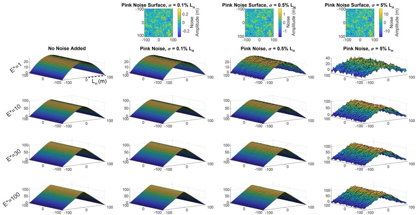
955 Figure 8: Synthetic hillslopes constructed using Equation 11. Upper row shows pink noise surfaces that are added to the original hillslope form (left column); yellow colors correspond with positive deviations from the hillslope (convex noise) and blue with negative deviations (concave noise). Each row of hillslopes corresponds with range of dimensionless erosion rates, from E^*=1 -100. Note the increased prominence of planar hillslopes as E^* increases; the z-axis on each plot may differ. Noise does not vary with E^* ; thus the magnitude of noise relative to hillslope relief is more visually apparent at lower E^* (See \sigma=5\% L_H column for clear example). Note that all results in Fig. 10C, G, K, and O correspond with the third column here ( \sigma=0.5\% L_H ). See supplemental for corresponding figures for \sigma=0.1\% L_H and \sigma=5\% L_H cases. 960
