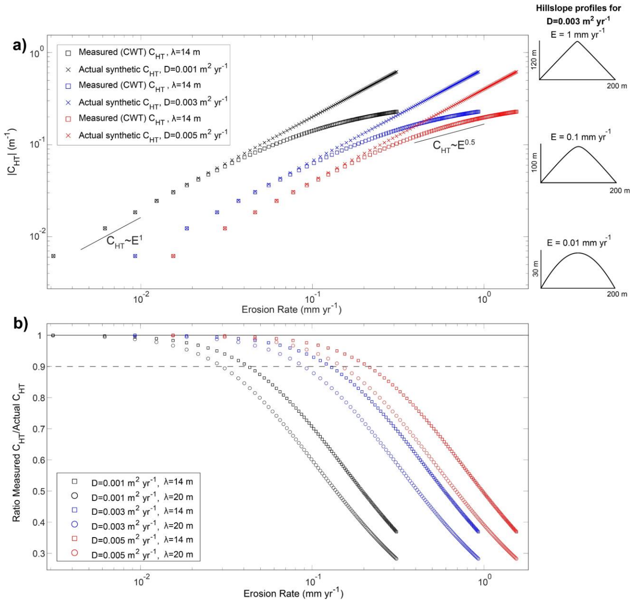
Figure 11: A) The absolute value of C_{HT} plotted against erosion rate for synthetic hillslopes constructed for E^*=1-100 , corresponding to erosion rates of \sim 0.01-1\ mm\ yr^{-1} for diffusivities ranging from D=0.001-0.005\ m^2\ yr^{-1} ( \frac{\rho_s}{\rho_r}=0.5 ). Crosses correspond with the actual C_{HT} for each synthetic hillslope constructed for a given E^* . Squares are C_{HT-w} , using the L07 \lambda definition. In this case \lambda = 14\ m . Note the linear relationship between C_{HT} and erosion rate at small erosion rates, in agreement with Equation 1. As erosion rate increases, the relationship between measured C_{HT} and E is no longer linear but could be potentially expressed as a power law. The erosion rate at which this deviation occurs is visualized in panel B. An example square root relationship is plotted at these erosion rates for reference (Gabet et al., 2021). Note example synthetic hillslopes profiles (for D=0.003\ m^2\ yr^{-1} ) spanning the range of erosion rates on right side of panel (y-
