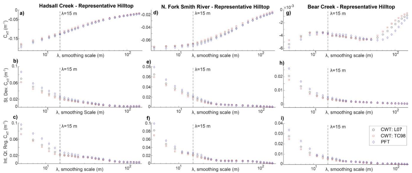
840 Figure 3: Curvature extracted from representative hilltop at Hadsall Creek, NFSR, and Bear Creek for a range of \lambda . Upper row is C_{HT} measurements, second row is the standard deviation of C_{HT} , and the bottom row is the interquartile range of C_{HT} . Note that the scaling break that identifies where tree throw pits are filtered out depends on the size of the considered hillslope and consistency of pit-mound topographic in a landscape. Here, though, a break exists at \lambda \approx 15 m for Hadsall Creek (especially apparent in standard deviation and interquartile range) and the NFSR and Bear Creek at \lambda \approx 11-20 m (note that second break at \sim 60 m in Bear Creek corresponds to the introduction of concave valleys). These scaling breaks are generally consistent with those observed for the OCR by Roering et al. (2010) and are visible for CWT and PFT \lambda definitions. L07: Lashermes et al. (2007); TC98: Torrence and Compo (1998). 845
