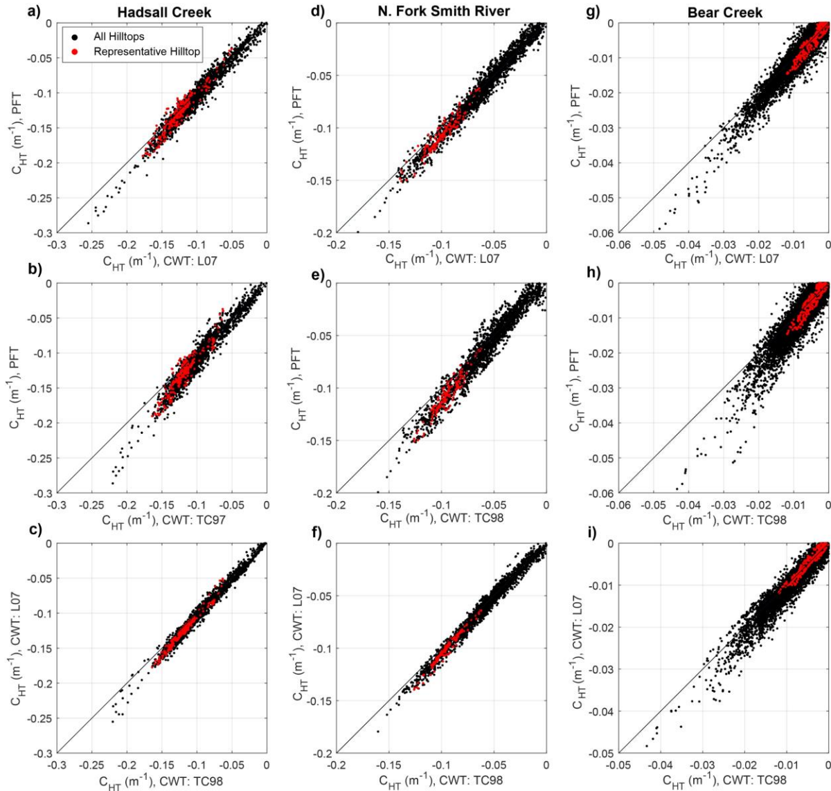
Figure 5: Comparison of C_{HT} calculation methods for \lambda=15 m. Black dots correspond with curvature measured at nodes for all mapped hilltops (roads, landslides, valley bottoms, etc. removed). Red points correspond with the representative
