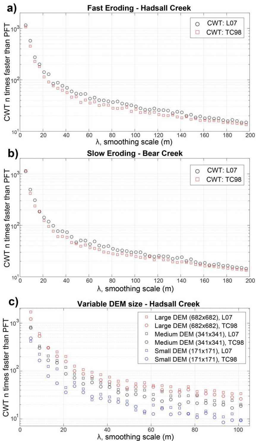
850 Figure 4: Speed of the CWT compared to the PFT for different smoothing scales, \lambda . A, B: Relative speed of the CWT to the PFT for small portions (513x513 single precision grid, cell size of 0.9144 m) of the Hadsall and Bear Creek
