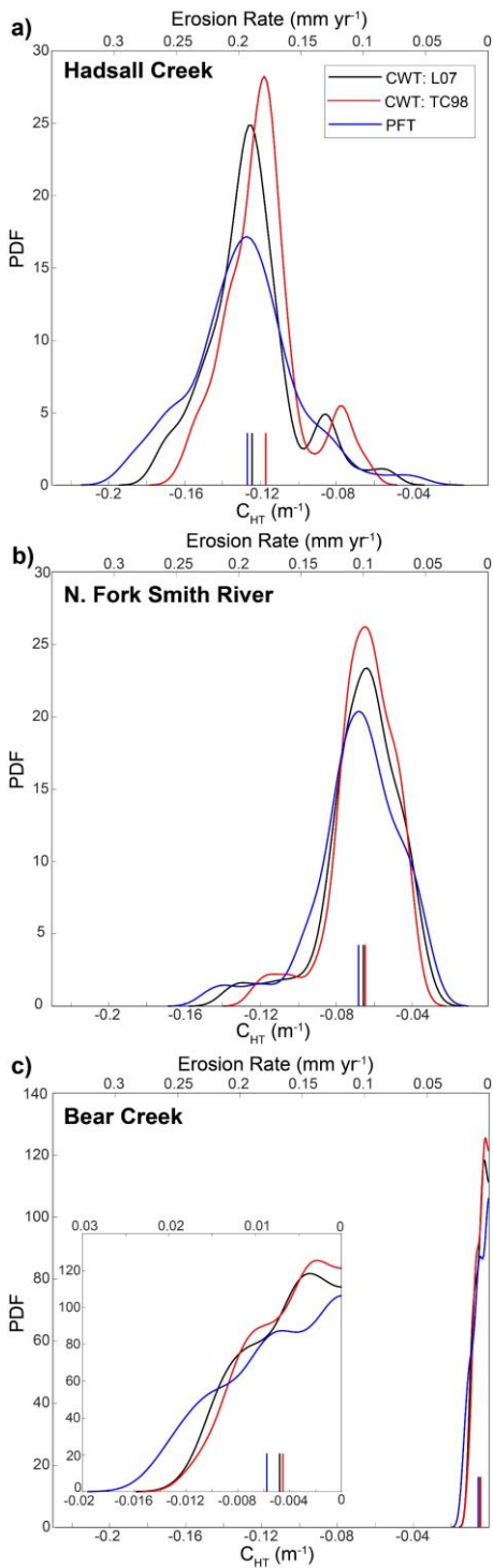
900 Figure 6: Probability density functions of C_{HT} (bottom x-axis) and erosion rate calculated using Equation 1 (top x-axis) for the representative hilltop at each OCR field site. See Fig. S1 for all mapped hilltops version. Note agreement between each C_{HT} calculation method. Further, note dramatic variability in C_{HT} between sites (all panels use same x-axis; inset
