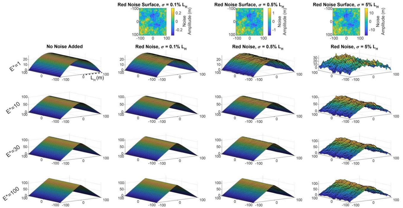
Figure 9: Synthetic hillslopes constructed using Equation 11. Same as Fig. 8, but with red noise added (see supplemental for white noise example). Upper row shows red noise surfaces added to the original hillslope form (left column); yellow colors correspond with positive deviations from the hillslope (convex noise) and blue with negative deviations (concave noise). Each row of hillslopes corresponds with dimensionless erosion rates from E^*=1-100 . Note the increased prominence of planar hillslopes as E^* increases. Noise does not vary with E^* ; thus the magnitude of noise relative to hillslope relief is more visually apparent at lower E^* (See \sigma=5\% L_H column for clear example). Note that compared to Fig. 8, the surface noise exhibits longer wavelength noise, made apparent by larger concave and convex regions. Note that all results in Fig. 10D, H, I, and P correspond with the third column here ( \sigma=0.5\% L_H ). See supplemental for corresponding figures for other \sigma=0.1\%L_H and \sigma=5\%L_H cases.
