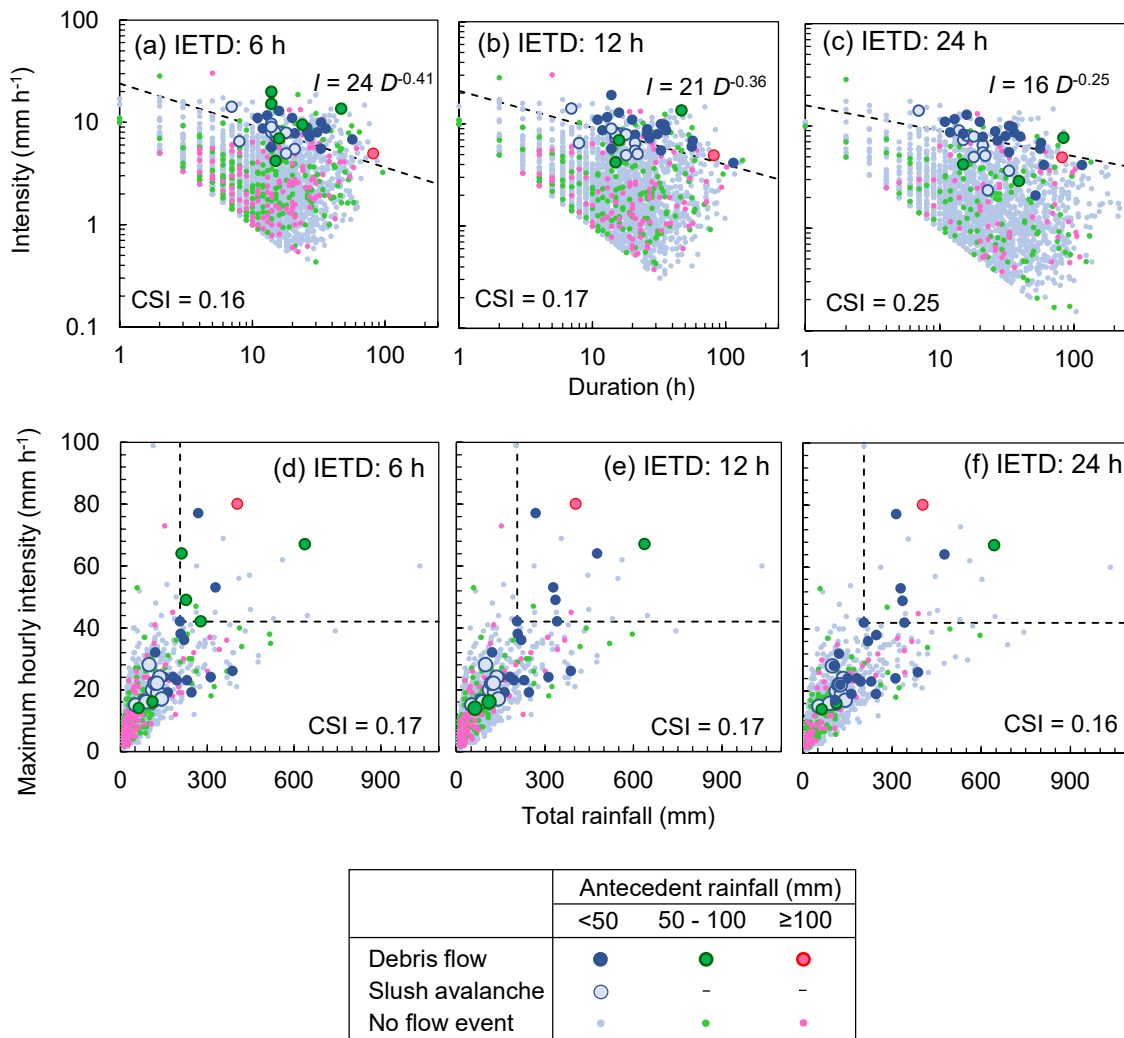
360 Figure 8: Rainfall thresholds for triggering debris flows and slush avalanches. Comparison of the duration and intensity of rainfall events with or without debris flows and slush avalanches that were calculated with an inter event time definition (IETD) of (a) 6 h, (b) 12 h, and (c) 24 h. Dashed lines indicate the rainfall thresholds with the highest critical successful index (CSI). Comparison of the total rainfall and maximum hourly rainfall intensity of rainfall events with or without debris flows and slush avalanches that were calculated with an IETD of (d) 6 h, (e) 12 h, and (f) 24 h.
