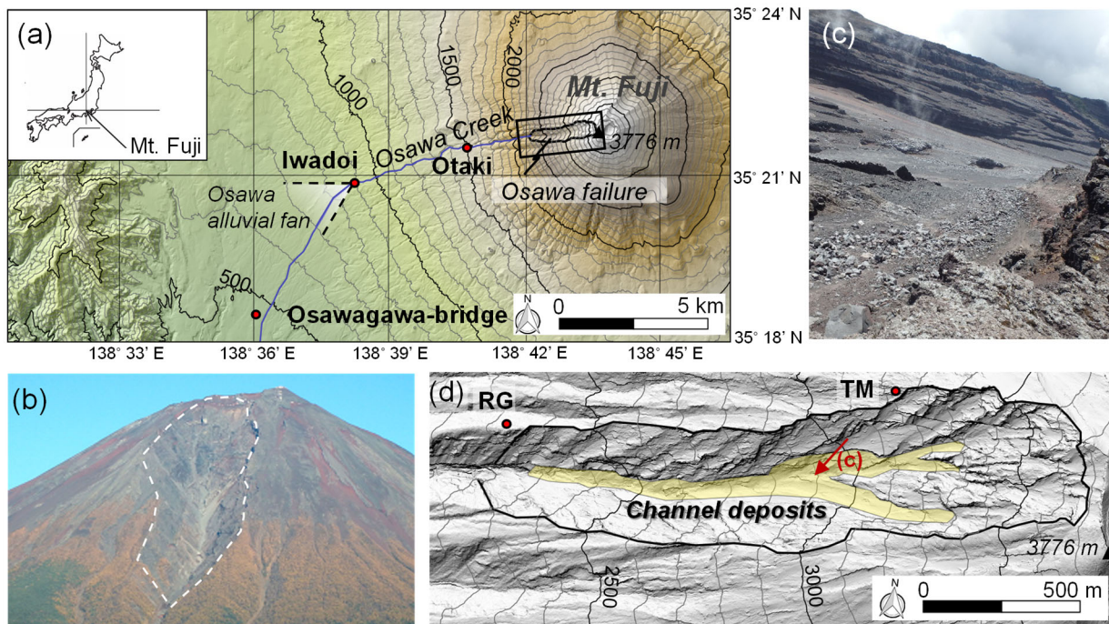
105 Figure 1: Topographic map and photographs of the Osawa failure. (a) Topographic map of the area around the Osawa failure and 110 Osawa Creek. The area shown in (d) is located within the black-outlined box. (b) Full view of Mt. Fuji. The location of the Osawa failure is indicated by the white dashed line. (c) Channel deposits in the Osawa failure. The location where this photograph was taken is indicated by the red arrow in (d). (d) Topographic map of the area around the Osawa failure. RG and TM indicate the locations of a rain gauge and ground temperature sensors, respectively. The summit meteorological station is located on the triangle of the mountain peak.
