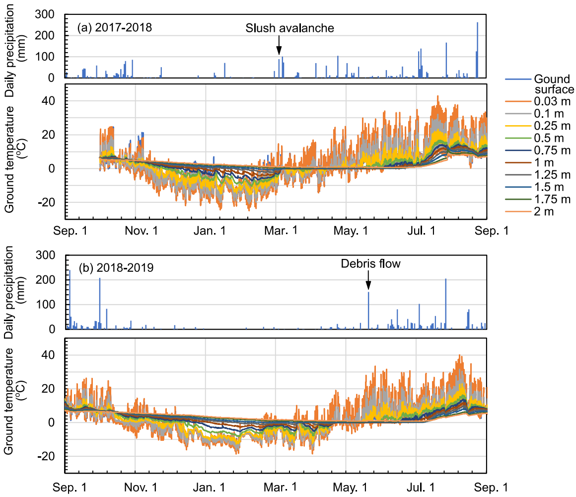
290 Figure 4: Temporal changes in the ground temperature at 3,220 m a.s.l. from September 1, 2017 to September 1, 2019. Daily precipitation is also shown in the figure.
