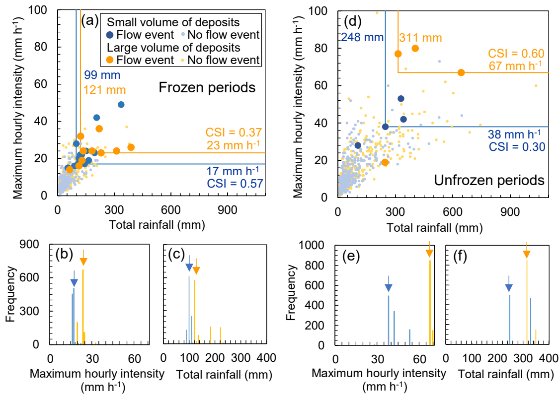
435 Figure 12: Comparison of the total rainfall and maximum hourly rainfall in rain events with or without debris flows and slush avalanches, plotted according to the volume class of channel deposits. The boundary between the two volume classes was set to 350,000 m 3 . (a) Comparison during frozen periods. The lines in the plots indicate the rainfall thresholds that optimally separated rainfall events that induced debris flows and slush avalanches and those that did not. Frequencies of (b) maximum hourly rainfall intensity and (c) total rainfall, which produced the highest critical successful index (CSI), obtained by 1,000 bootstrap resamplings 440 during frozen periods. (d) Comparison during unfrozen periods. Frequencies of (e) maximum rainfall intensity and (f) total rainfall obtained by bootstrap resampling.
