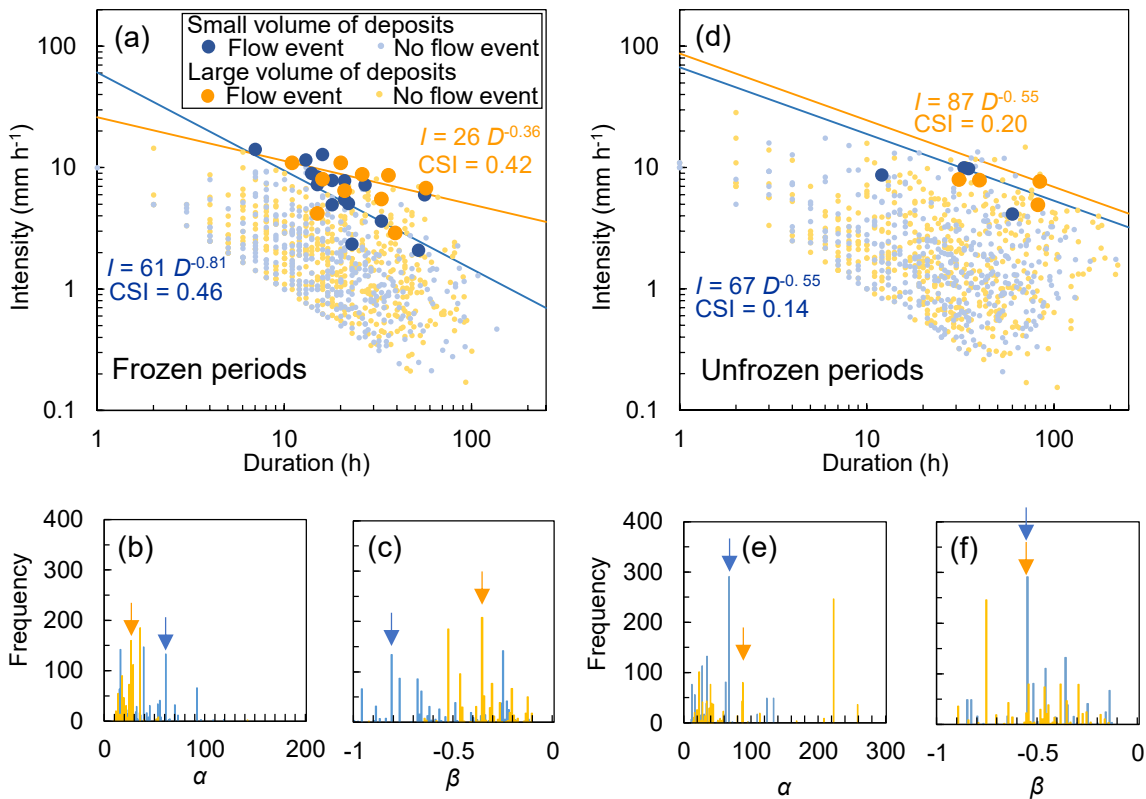
430 Figure 11: Comparison of the duration and intensity of rainfall events with or without debris flows and slush avalanches, analyzed according to the volume of channel deposits. The boundary between the two volume classes was set to 350,000 m 3 . (a) Comparison during frozen periods. The frequencies of (b) constant \alpha and (c) slope of the power law curve \beta , which produced the highest critical successful index (CSI), obtained by 1,000 bootstrap resamplings during frozen periods. (d) Comparison during unfrozen periods. (a) Comparison during frozen periods. Frequencies of the (e) constant \alpha and (f) slope of the power law curve \beta obtained by bootstrap resampling during unfrozen periods.
