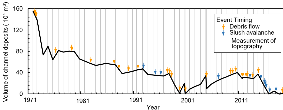
270 Figure 3: Temporal changes in the volume of channel deposits in the Osawa failure (original data from Fuji Sabo Office, 2020).
