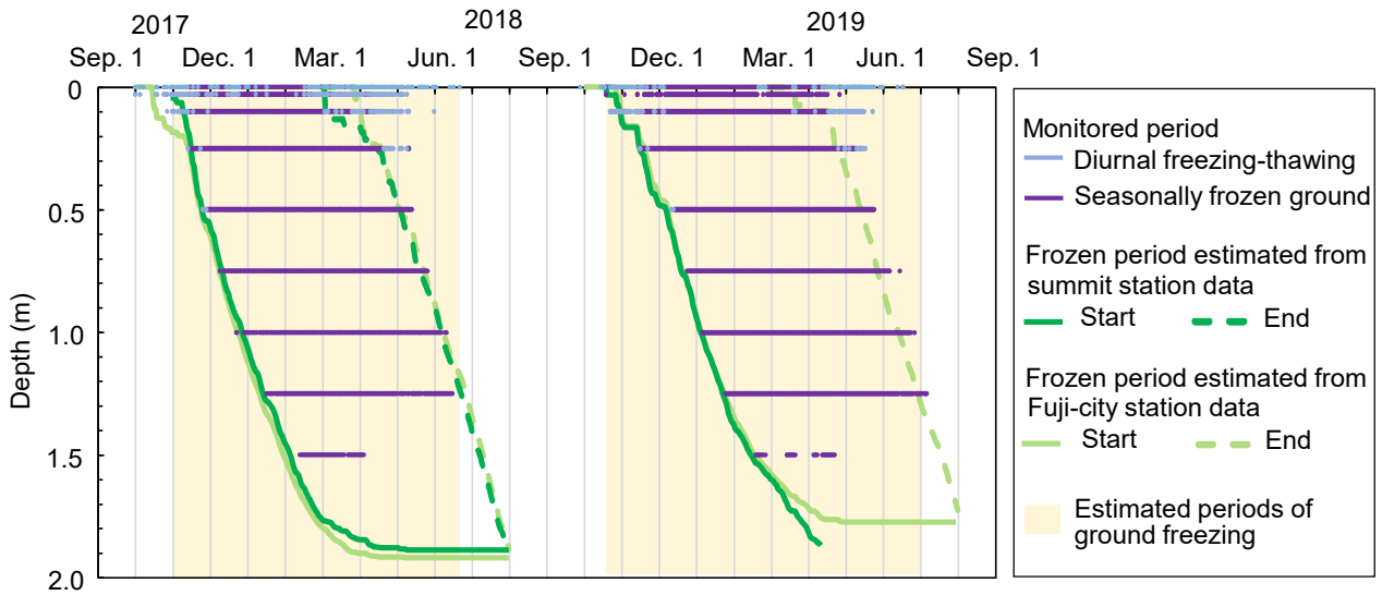
295 Figure 5: Comparison of observed and estimated periods of diurnal freeze-thaw activity and seasonal ground freezing at 3,221 a.s.l. The timing of thawing in 2019 could not be estimated using data from the summit station due to monitoring equipment failure. Periods of ground freezing were estimated using summit station data, whereas the end of the frozen period in 2019 was estimated using data from the Fuji City station.
