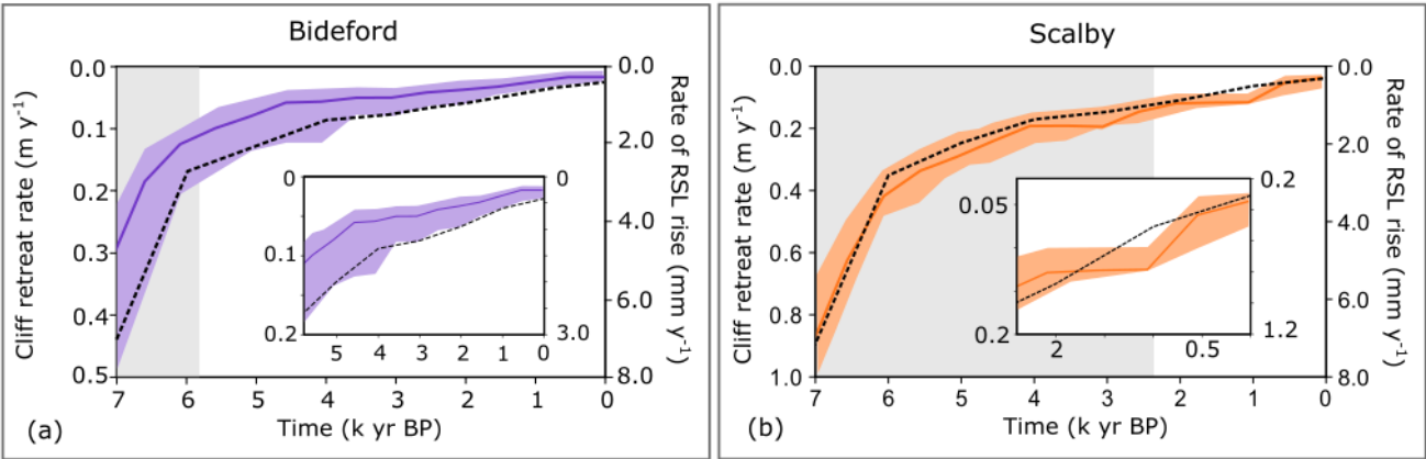
Figure 7: A time series of cliff retreat rate (m yr -1 ) shown by the solid line and shaded area across the late Holocene (from 7000 yr BP to present day) calculated from modelled cliff positions every 100 years. The first 1 kyr is excluded as this corresponds to the burn in period of the model. The rate of RSL rise (mm yr -1 ) is shown alongside cliff retreat rates by the dashed black line. Inset plots show the cliff retreat rates and rate of RSL rise for the time period that correspond with the distance across the shore platform over which measured data were analysed (~250 m). For Bideford (a), the past 5800 years of modelled cliff retreat correspond with the 250 m intertidal shore platform. For Scalby (b), the past 2700 years of modelled cliff retreat correspond with the 250 m intertidal shore platform. The grey shaded area corresponds to the cliff retreat rates which occurred further offshore than where the measured data was collected, and the non-shaded area shows the extent of the inset plots.
