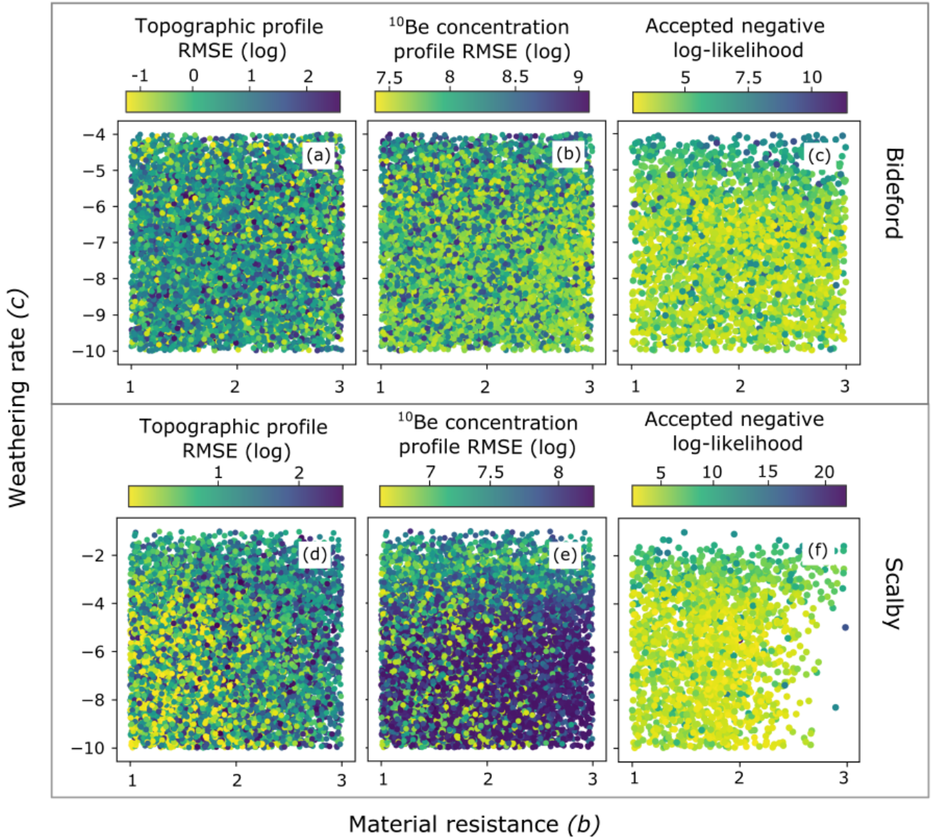
645 Figure 8: Objective function results for the material resistance ( b ) and weathering rate ( c ) parameters; constructed from 50 – 50% weighted MCMC analysis results for the Bideford site and Scalby site. The topographic profile RMSE [(a) and (d)] and ^{10}\text{Be} concentration profile RMSE [(b) and (e)] objective function spaces are constructed from all 10,000 samples visited in the MCMC analysis. The combined likelihood objective function space [(c) and (f)] is constructed just from the accepted samples from the MCMC analysis. Dark blue corresponds with the worst samples that have the highest RMSE and negative log-likelihood scores, while bright yellow corresponds with the best samples that have the lowest RMSE and negative log-likelihood scores. 650
