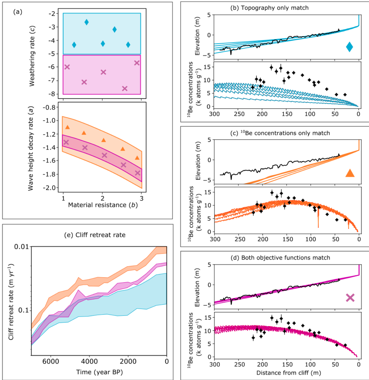
800 Figure 11: Objective function surface at Bideford (a), for parameters material resistance (b) and weathering rate (c), and material resistance (b) and wave height decay rate (a). Blue shaded region (a) shows where in the parameter space the modelled topographic profile alone can match measured data. Blue diamond's (a) correspond to example model results shown in (b). Orange shaded region (a) shows where in the parameter space the modelled ^{10}\text{Be} concentration profile alone can match measured data. Orange triangles (a) correspond to example model results shown in (c). Pink shaded region (a) shows where in the parameter 805 space both the modelled topographic profile and ^{10}\text{Be} concentration profile can match measured data. Pink crosses (a) correspond to example model results shown in (d). Cliff retreat rates (m \text{yr}^{-1} ) on a log-scale for each set of model examples are shown in (e). Model results are from the 50 - 50% weighted Pareto set simulation.
