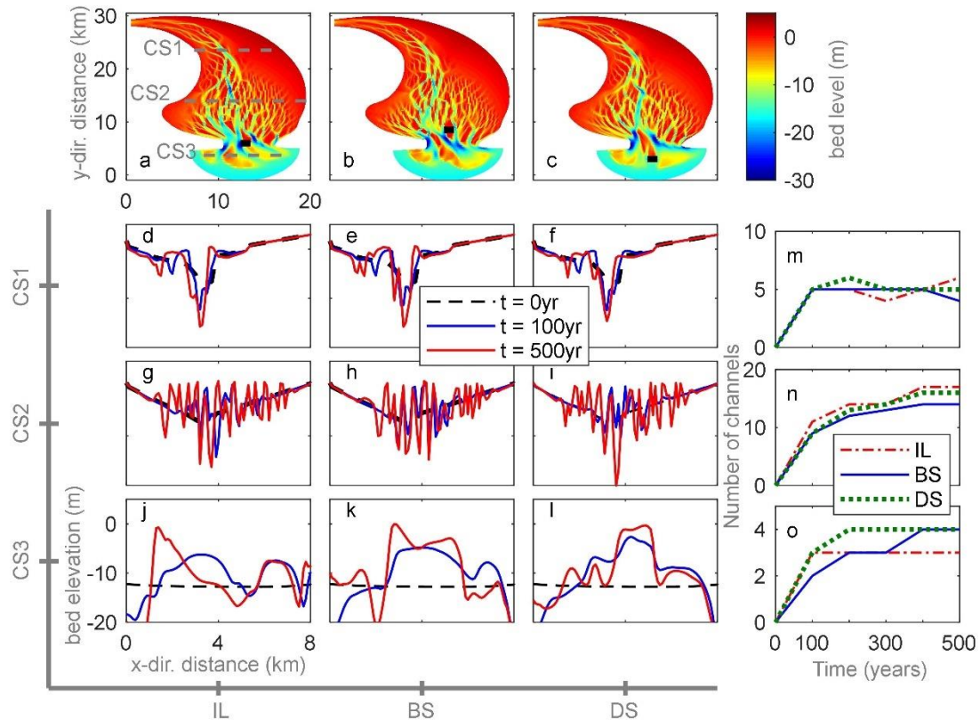
210 Figure 6: Morphological evolution after 500 years (a-c) of basin with mouth island at the inlet (“IL”), at the basin-side (“BS”) and the delta-side (“DS”) respectively. Figures d-l represent the temporal cross-sectional bed elevation of different cases: (d-f) cross-section 1; (g-i) cross-section 2 and (j-l) cross-section 3. Figures m-o represent the number of channels of different cross-sections respectively. In some subplots, the black rectangle area represents the mouth island and the grey dotted lines represent the cross-section position.
