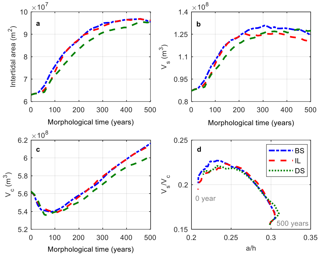
Figure 13: Temporal variation of intertidal flat area (a), intertidal storage volume (b), channel volume (c) and the ratio of V_s/V_c in the inner basin of different island locations.
