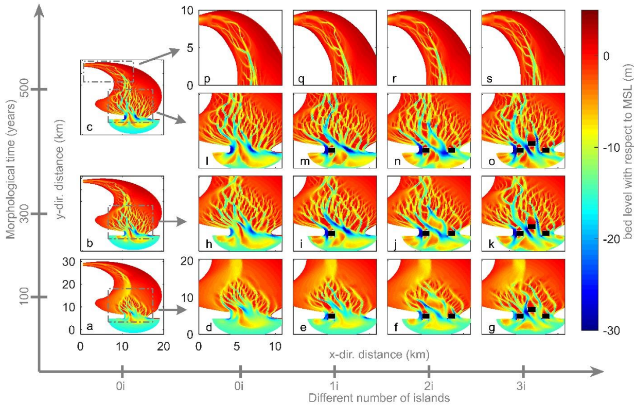
170 Figure 4: Morphological evolution after 100 years (a, d-g), 300 years (b, h-k) and 500 years (c, l-s) of basin without island (“0i”), basin with one island (“1i”), basin with two islands (“2i”) and basin with three islands (“3i”) respectively. Here we only plot part of the model domain, where the bed level changes. The black solid rectangles in subplots m, n, o, i, j, k, e, f and g represent mouth islands.
