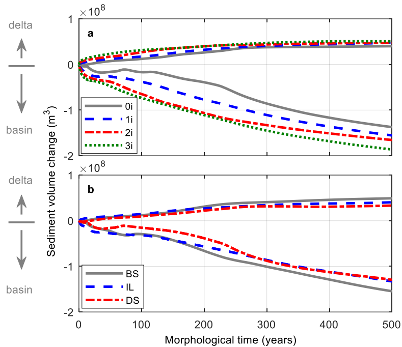
Figure 14: Cumulative sediment volume change over time of different scenarios: (a) scenarios of the different mouth island numbers, and (b) scenarios of different mouth island locations.
