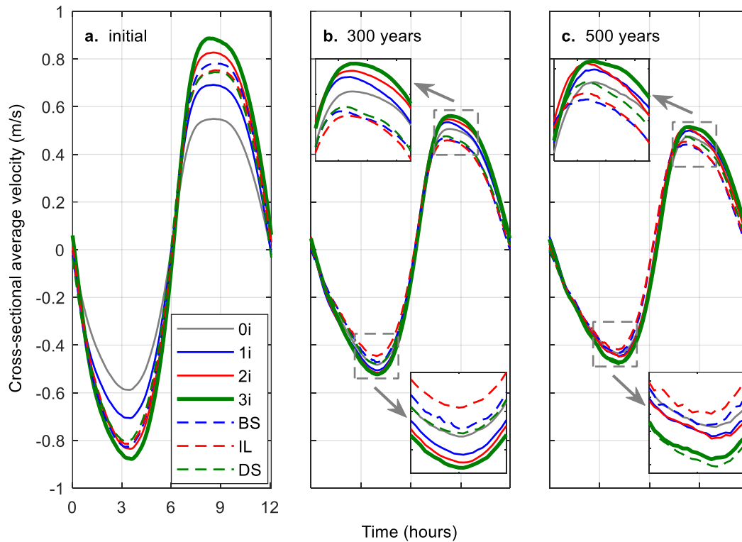
Figure 12: The cross-sectional average velocity over a tidal cycle of different scenarios after: (a) 0 years, (b) 300 years, and (c) 500 years. The flood tidal velocity is positive.
