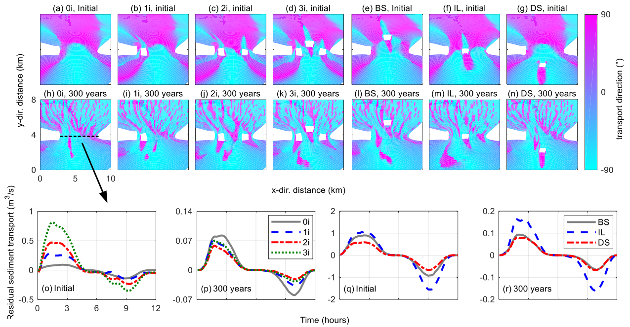
Figure 8: Residual sediment transport near the tidal inlet for different number of mouth islands (a-d, h-k) and different locations (e-g, l-n) at the beginning and after 300 years respectively. The white area in the plot represents the mouth islands and the background colour represents the direction of residual sediment transport (90 degrees indicate landward transport while -90 degrees indicate seaward transport). Tidal residual sediment transport via a cross-section of different scenarios at 0 (o, q) and 300 years (p, r) respectively. In subplots 8o-r, a positive value indicates seaward transport while a negative value indicates landward transport.
