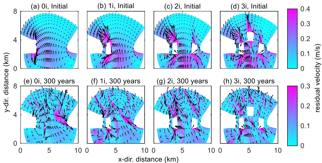
235 Figure 7: Spatial distribution of the residual current (arrow vectors indicate the direction) near the tidal inlet of four different scenarios: (a-d) represent without island (“0i”), one island (“1i”), two islands (“2i”) and three islands (“3i”) at the beginning respectively; (e-h) after 300 years. The white area in the plot represents the mouth islands and the background colour represents the magnitude of residual velocity.
