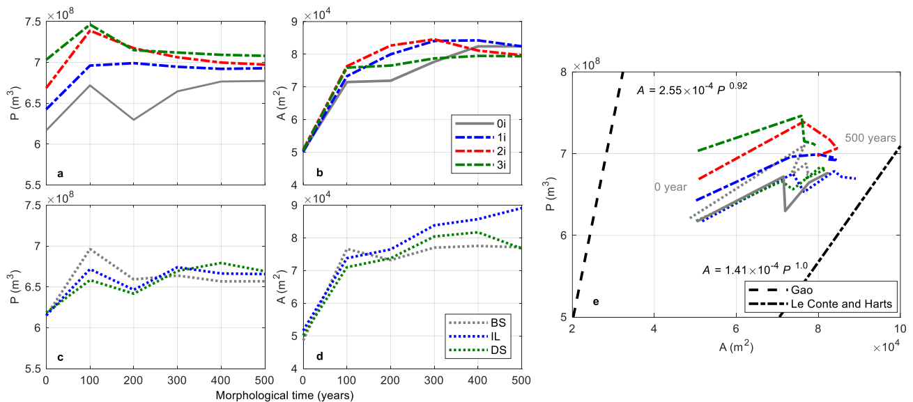
Figure 10: The evolution of tidal prism, inlet cross-sectional area and “P-A relation” for the different mouth island scenarios over 500 years. (a) and (b) for the scenarios of different mouth island numbers, (c), and (d) for the scenarios of different mouth island locations.
