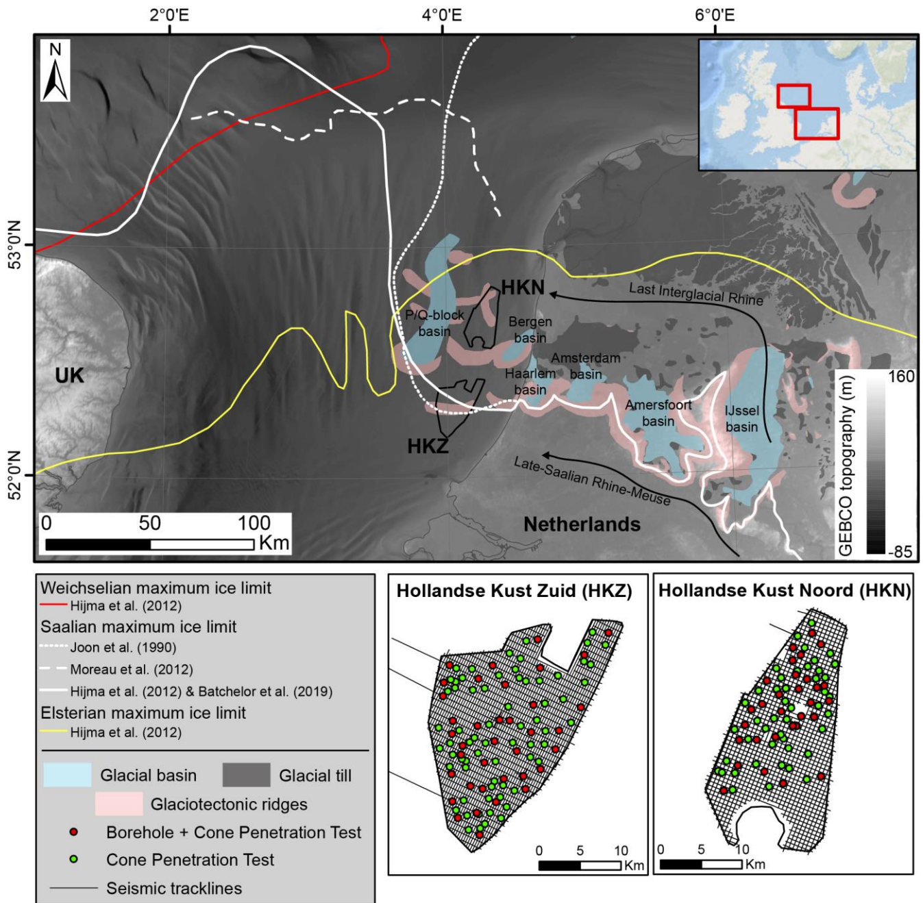
80 Figure 1. Location of the study area in the southern North Sea showing the Hollandse Kust Noord (HKN) and Zuid (HKZ) windfarm areas. The offshore maximum ice-sheet extension for the Weichselian (Marine Isotope Stage [MIS] 2), late Saalian (MIS 6; Drenthe Substage) and Elsterian (MIS 12 and/or 10) glaciations is displayed (modified from Batchelor et al., 2019; Graham et al., 2011; Hijma et al., 2012; Joon et al., 1990; Laban, 1995; and Moreau et al., 2012). The seismic tracklines displayed correspond to the multi- 85 channel sparker data. Onshore and offshore features compiled from Laban and van der Meer (2011), Joon et al. (1990) and Peeters et al. (2016). Modern bathymetry and topography from GEBCO ( https://www.gebco.net ).
