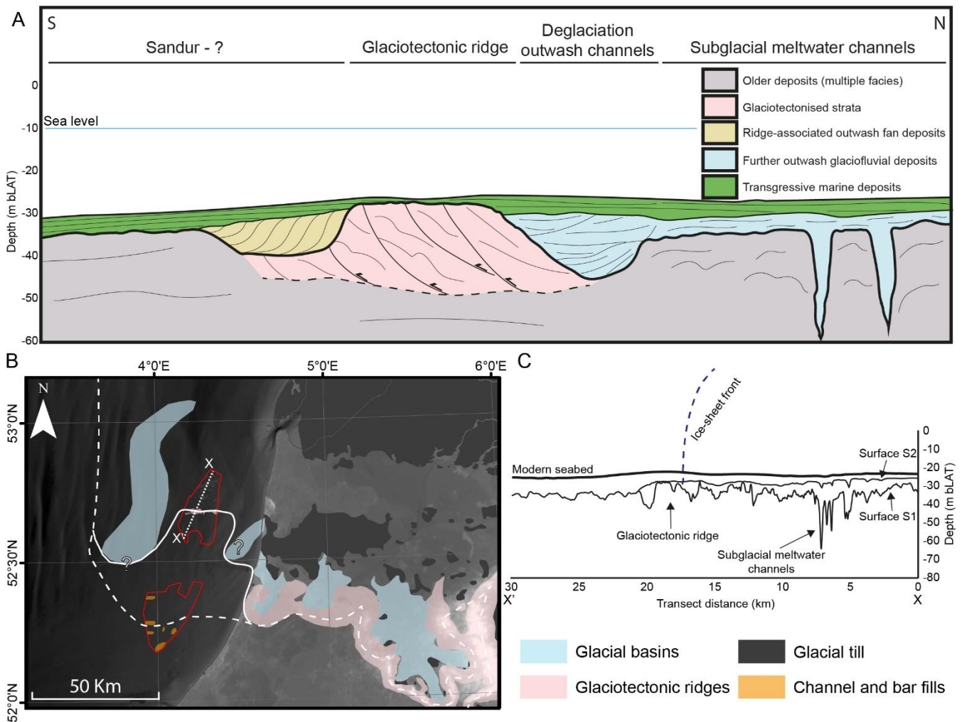
Figure 8. (A) Conceptual model of the infill (following transgression from MIS 6 to MIS 5e) showing the main glacial geomorphological features and sediments preserved in HKN windfarmHollandse Kust Noord . (B) Comparison between the previously inferred maximum Saalian ice sheet extent (dashed line) and the new limit proposed in this study (solid line). Channel and bar fills identified in HKZ windfarm are also indicated (some of them formerly interpreted as glaciotectonic ridges). Legend and sources as in Fig. 1. (C) Bathymetry profile through the HKN windfarmHollandse Kust Noord area highlighting the glacial geomorphological features identified and the approximate position of the ice front during the maximum ice sheet extent.
