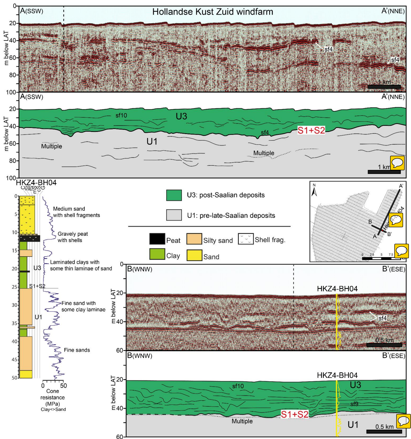
Figure 7. Representative seismic profiles showing the stratigraphy underlying the HKZ windfarm site. Section A-A' corresponds to a multi-channel sparker line, section B-B' to a single-channel sparker line. Borehole HKZ4-BH04 illustrates the sedimentological characteristics of units U1 and U3 in this windfarm. Only the upper 50 m of the borehole are shown. Cone resistance from a CPT
