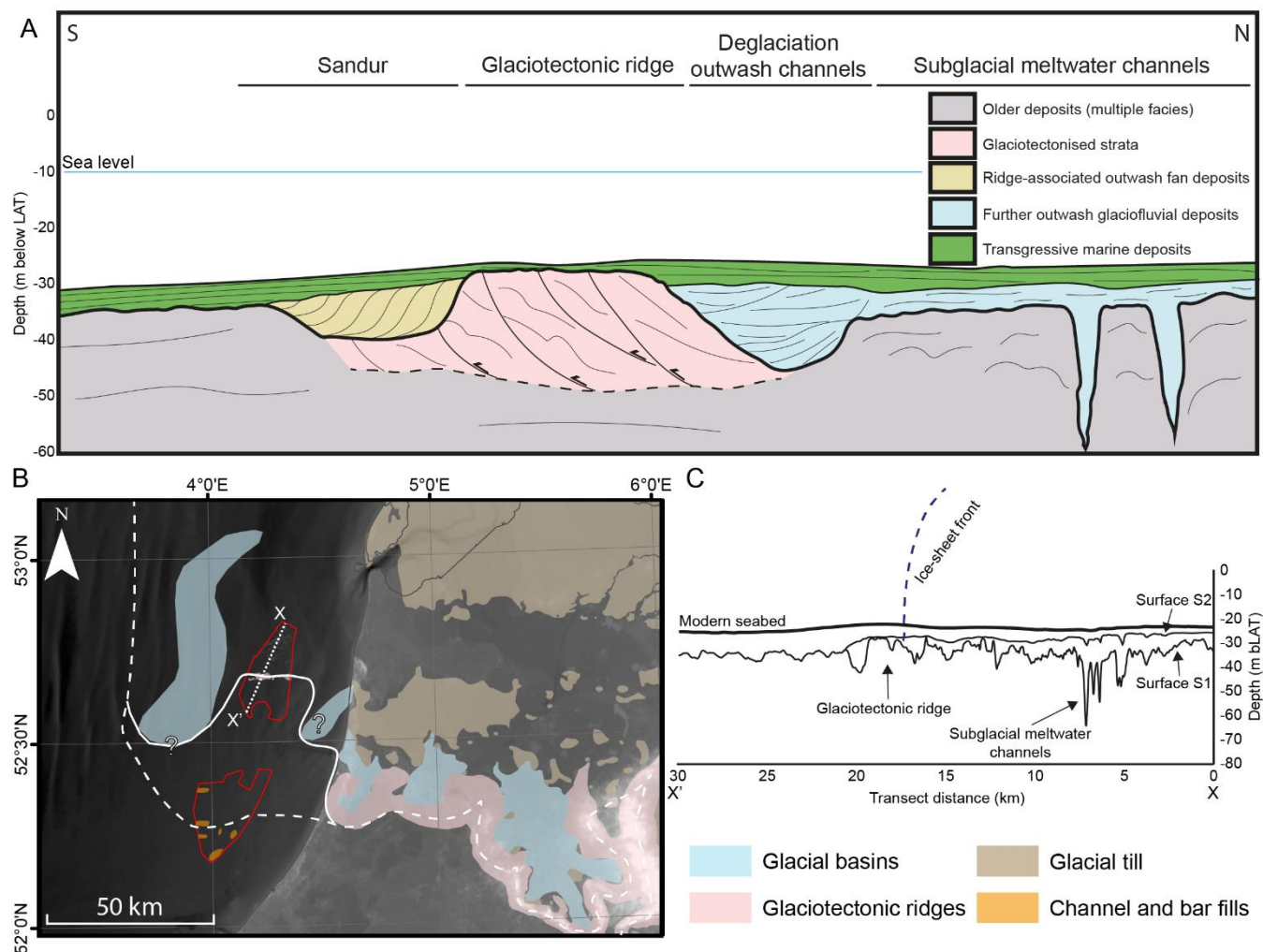
Figure 8. (A) Conceptual model of the infill (following transgression from MIS 6 to MIS 5e, but before the highstand) showing the main glacial geomorphological features and sediments preserved in HKN windfarm. (B) Comparison between the previously inferred maximum Saalian ice sheet extent (dashed line, Hijma et al, 2012, Batchelor et al., 2019) and the new limit proposed in this study (solid line). Question marks indicate sectors where the limit is uncertain and more research is needed (see text for details). Channel and bar fills identified in HKZ windfarm are also indicated (some of them formerly interpreted as glaciotectionic ridges). Sources for onshore and offshore features as in Fig. 1. (C) Bathymetry profile through the HKN windfarm area highlighting the glacial geomorphological features identified and the approximate position of the ice front during the maximum ice sheet extent.
