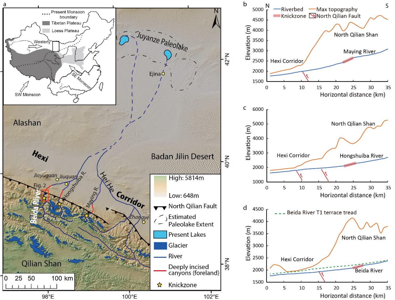
45 Figure 1 a . Digital elevation map of the research area and the Hei He drainage system . Glacial/Active glacial coverage mapped based on Raup et al., (2007). Inset figure: Location of our research area with respect to monsoon and westerly moisture sources.
