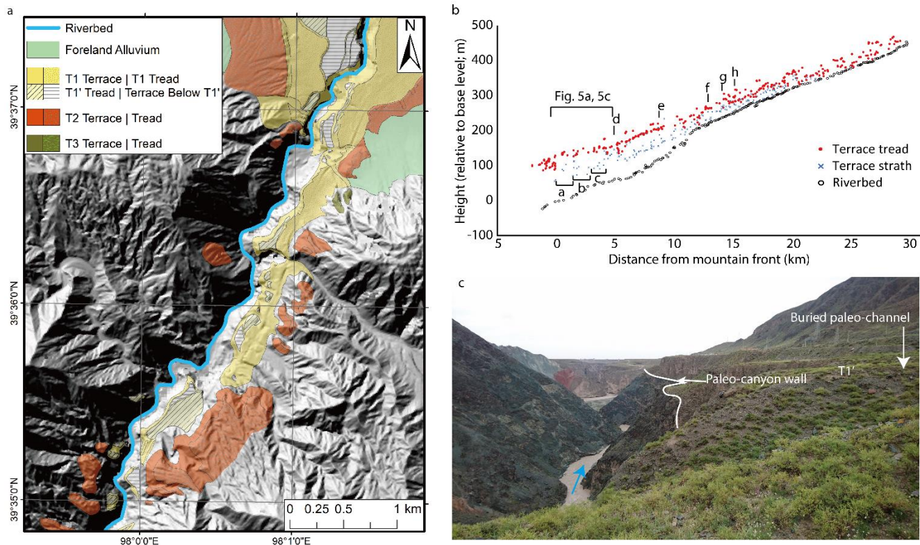
Figure 5 Bedrock incision and terrace preservation along the Beida River. a. Terrace map of the lower reach of Beida River. T1 terraces are all preserved on the east side of the canyon. b. Terrace profiles of Beida River. Letters correspond to reaches where terrace mapping indicates that the original paleocanyon is preserved and the river incised into the adjacent bedrock soon after the abandonment of T1' (See Figure S3S5). c. Photo of the lower reach of Beida River, looking downstream, with paleochannel axis and paleo-canyon wall annotated. Here the river incised mostly into bedrock along the west edge of the T1 terrace fill deposit.
