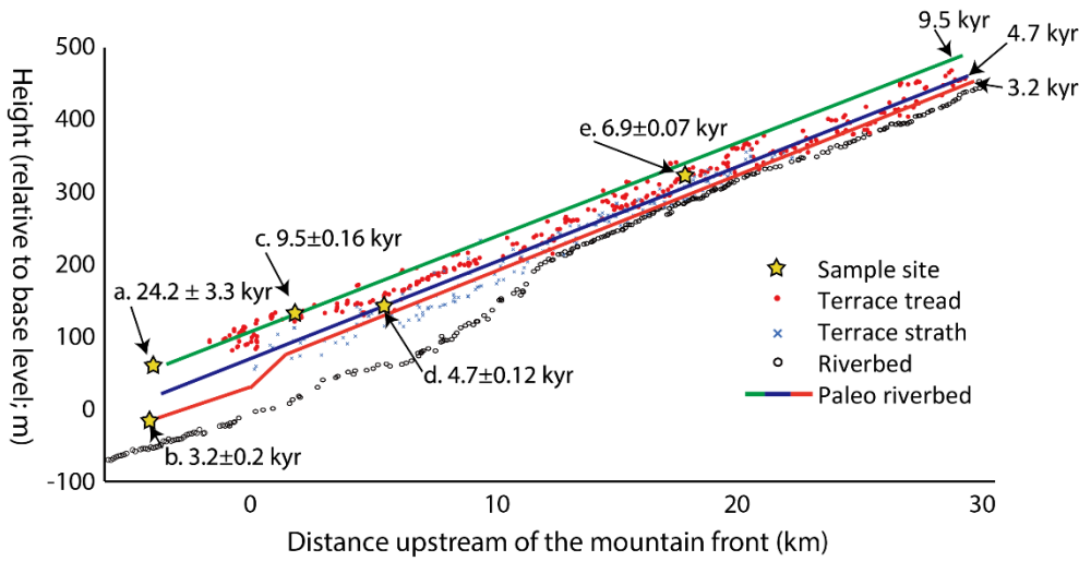
Figure 6 Simplified model for Beida River incision since 9.5 kyr. The surveyed terrace treads and the paleo riverbeds we projected are corrected for tectonic uplift, therefore slightly deviated from the sample locations. The time period between 24.2 to 9.5 kyr B.P. is not included in this model because the river was mostly incising into the T1 terrace fill, and therefore the incision of the foreland and hinterland should be synchronous.
