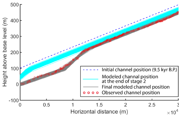
540 Figure 8 Monte-Carlo simulation of channel position at the end of stage 2 and at present, end of stage 3, compared to the observed river profile. 500 simulations results shown. Parameters for simulations were selected from valid model results for the timing, duration, and incision rate stages 2 and 3.
