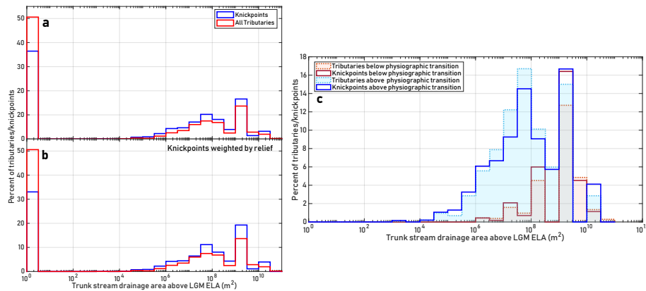
Figure 4. (a) Distribution of knickpoints ( n = 3707 ) and analysed 1 st and 2 nd order tributaries ( n = 3557 ) to 3 rd or higher order rivers with respect to the area of terrain above the ELA drained by the trunk stream. Knickpoints included in the analysis are located on a 1 st or 2 nd order tributary within 2 km of a confluence with a 3 rd or higher order trunk stream. Area is log-binned, the lowest area bin contains only knickpoints and confluences where the trunk stream does not drain any terrain above the ELA. See Methods for criteria for identifying knickpoints. (b) Same as 4A, but knickpoints are weighted by their relief. For both the relief-weighted and non-weighted knickpoint distributions, we conducted two-sample Kolmogorov-Smirnov tests for the distributions of knickpoints versus confluences with respect to above-ELA drainage areas and found the empirical CDF for the confluences is larger with P < 0.0001 . (c) Comparison of knickpoints and tributaries located above ( n = 1472 tributaries, n = 2549 knickpoints) and below ( n = 2085 tributaries, n = 1152 knickpoints) the physiographic transition (PT) (Figure 1). Including only those knickpoints and tributaries that drained to trunk streams with drainage area above the LGM ELA, we conducted two-sample Kolmogorov-Smirnov tests for the distributions of knickpoints versus confluences with respect to above-ELA drainage area, and found that the empirical CDF for the confluences is larger with P \approx 0.01 above the PT, while for the knickpoints below the PT we could not reject the null hypothesis with 95% confidence that they belong to the same distribution.
