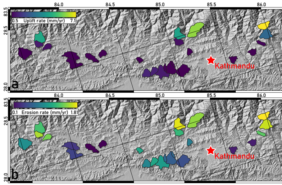
Figure 6. (a) Estimated uplift rate for basins with no or minimal drainage area above the LGM ELA (Lavé and Avouac, 2001). (b) Beryllium-10-derived basin-averaged denudation rates for the same basins (Godard et al., 2014).
