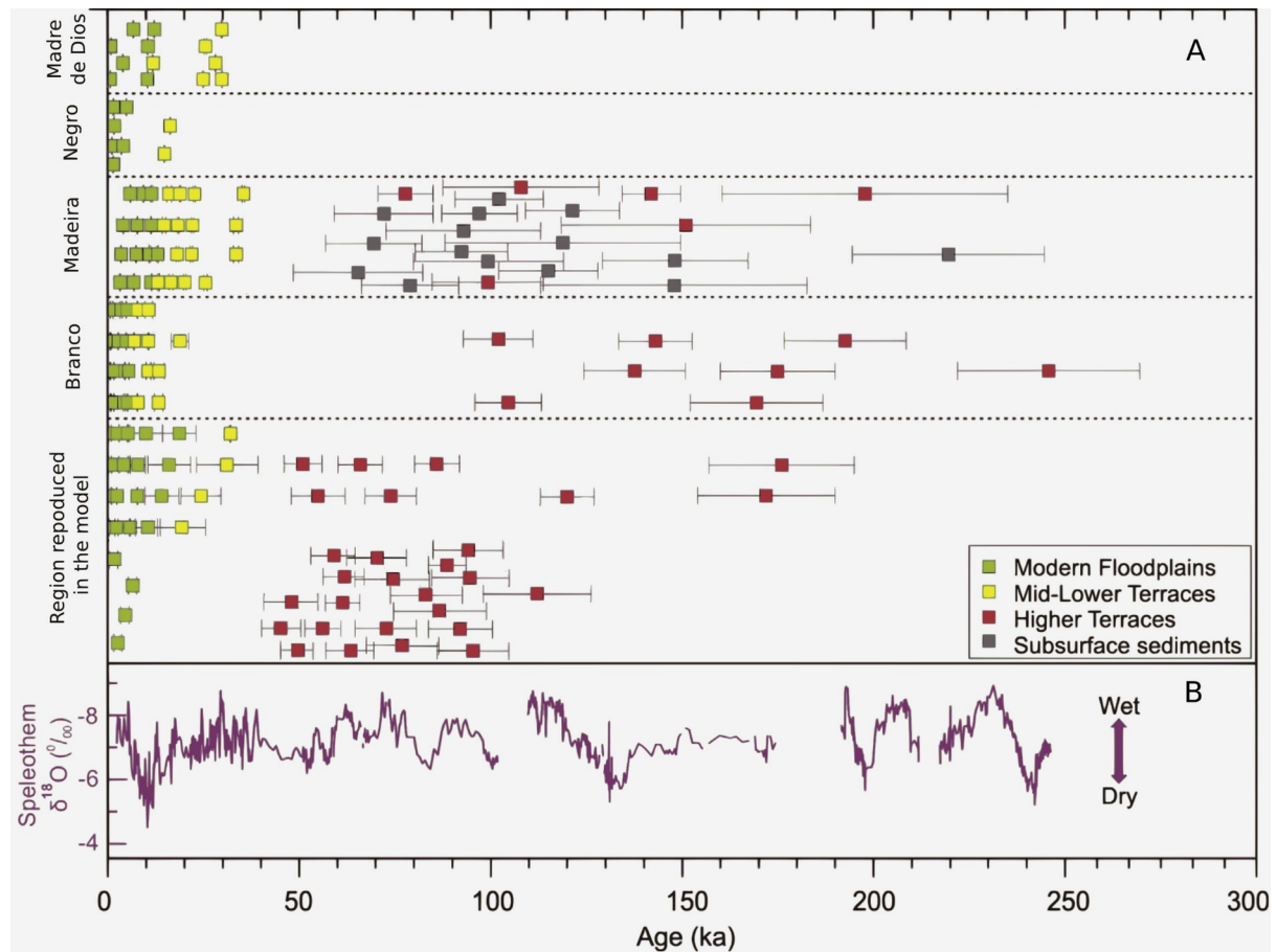
180 Figure 2 Chronology of sediment deposition representing the formation of terraces in Amazonian lowlands compared with Quaternary climate records from Pupim et al. (2019). (a) OSL and 14 C ages from late Quaternary deposits (b) Speleothem 18 O records.
