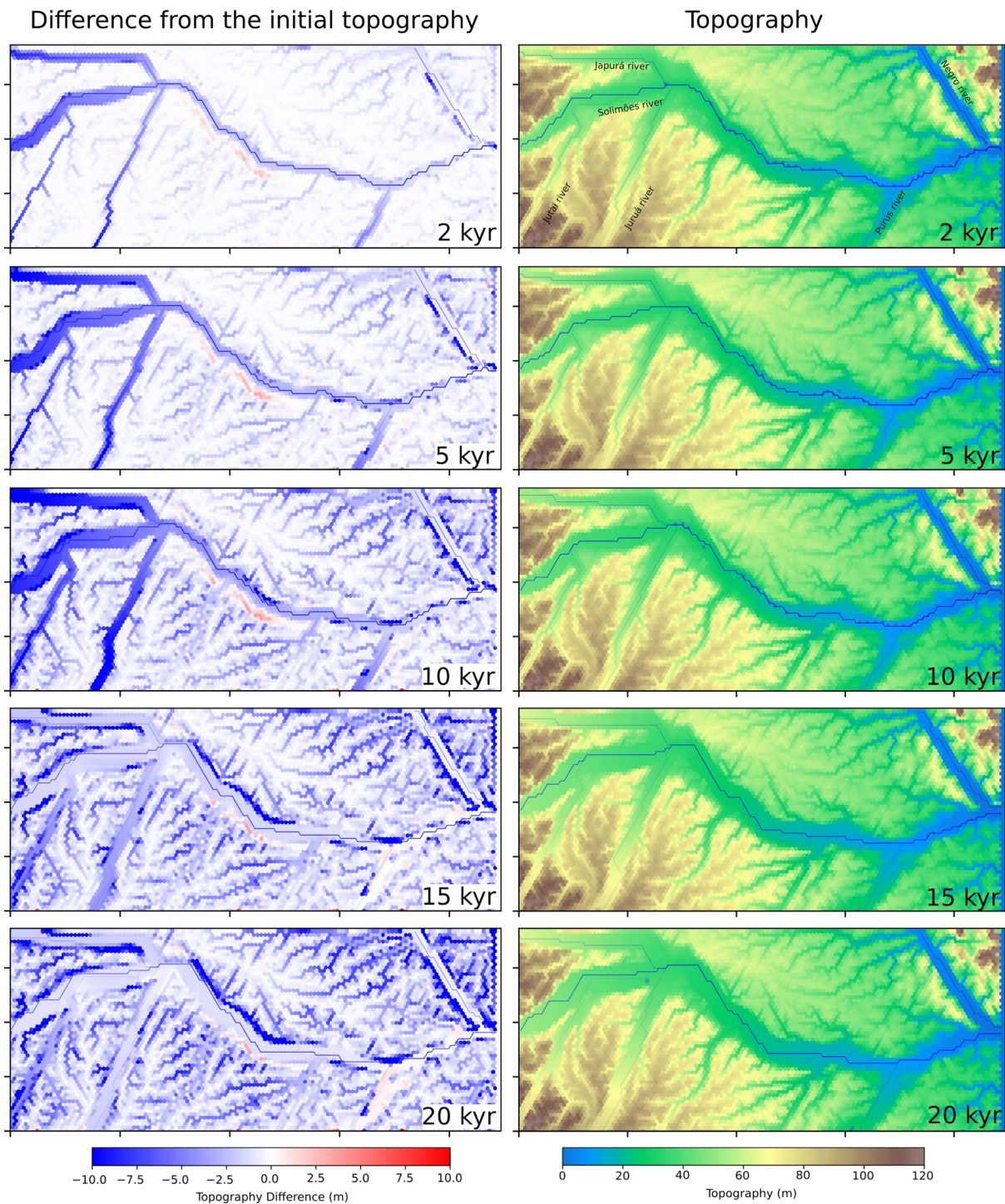
425 Figure 54 Results of the landscape evolution of scenario 21. The model water input is 30% less than the current water input (drier period) during the first 10 kyr. Subsequently, we employed a model water input that corresponds to the modern one until 20 kyr. The left figures show the difference of the model topography in relation to the initial topography, with colors saturated in red for values in elevation differences higher than 10 m, and in blue for values below - 10 m. The right column shows the topography itself. The occasional blue stains on the map represent lakes (local minima).
