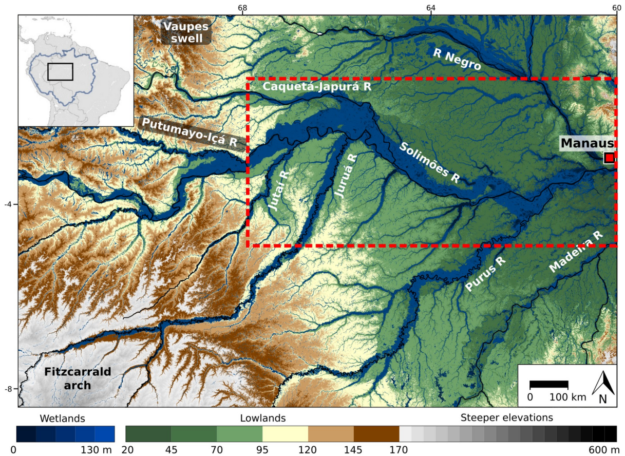
Figure 1 Topography of central Amazonia with key geographical designations such as cities, rivers, and geological and geomorphic features including terrace levels (Lowlands), floodplains (Wetlands) and drainage network. The red square illustrates the location of the city of Manaus. This illustration is based on a Digital Elevation Model from the Shuttle Radar Topography Mission. Red dotted rectangle square represents the region that is reproduced in the model and that represents the model grid. This illustration is based on a Digital Elevation Model from the Shuttle Radar Topography Mission.
