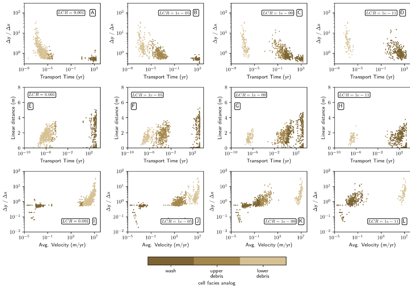
Figure 8: Scatter plots of the various transport histories of mobile regolith cells (Total Transport Time, Transport Index ( \Delta y / \Delta x ), and average transport velocity). A, B, C, D) Transport time versus transport Index for various lateral collapse rates (LCR). E, F, G, H) Transport Time versus Linear Distance for various lateral collapse rates. I, J, K, L) Average transport velocity versus Transport index. The scatter plots appear to show natural groupings of cells with similar transport histories. The color indicates our interpreted groupings of cells into analogs for the various sedimentary facies in the colluvial wedge model. These groupings are arbitrarily divided by the transport velocity with values greater than 10^5 m / day being ‘lower debris’ analog facies and cells with values lower than 1 m / day being ‘wash’ facies analogs. Cells between these values are classified as ‘upper debris’ facies analogs.
