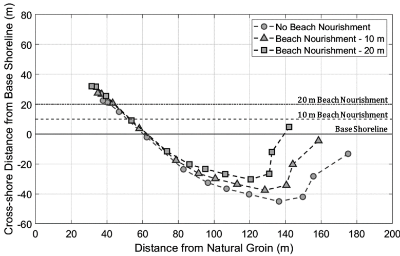
350 Figure 19: Change of maximum erosion width and indentation induced by beach nourishment of two different widths.
