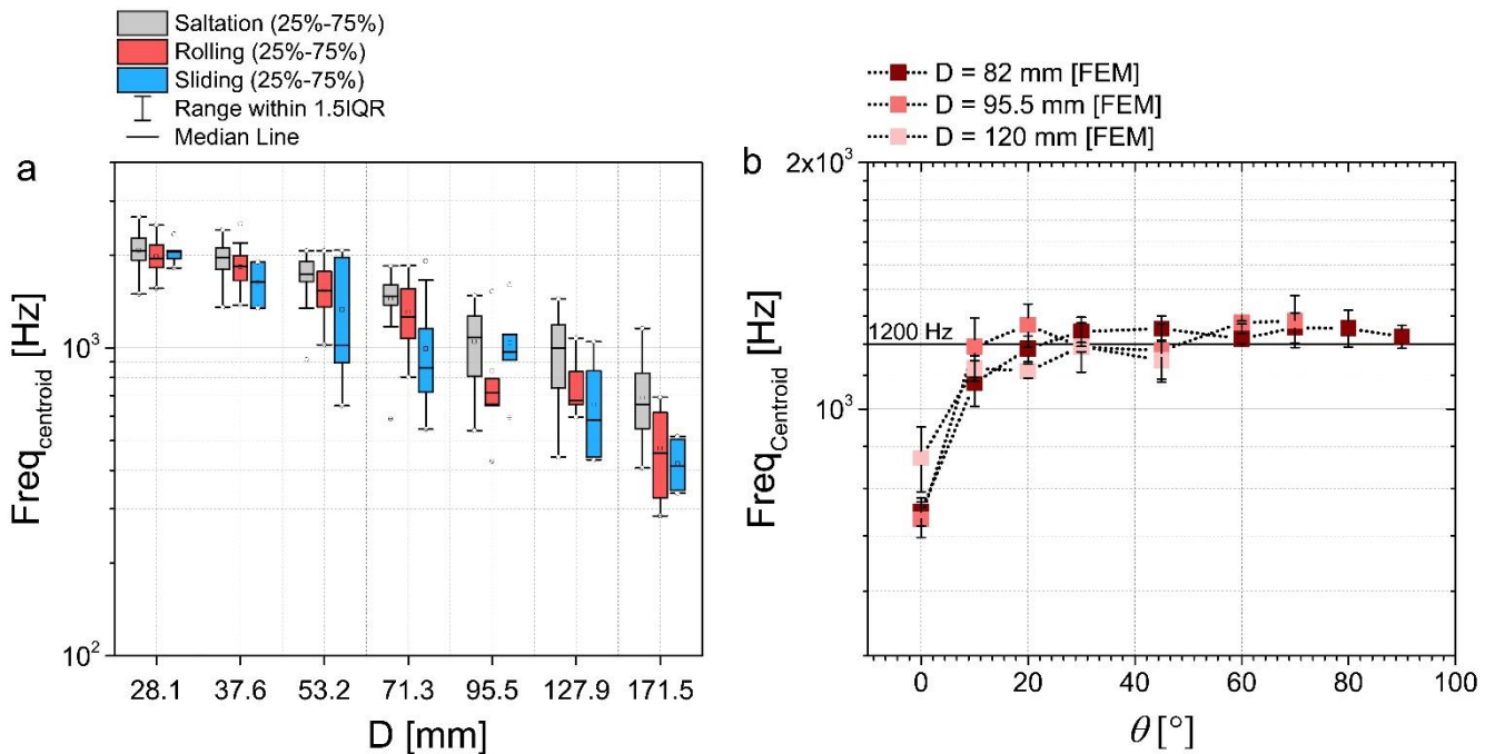
Figure 10: (a) Centroid frequency Freq_{Centroid} versus bedload particle size D for different motion modes. (b) Centroid frequency Freq_{Centroid} versus impact angle \theta for different impacting particle sizes. FEM denotes simulations with the finite element method.
