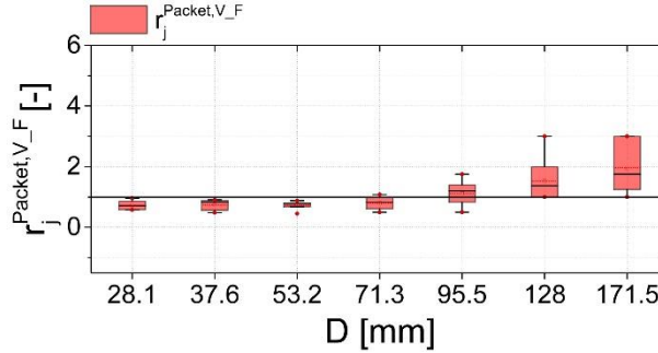
Figure 7: The ratio r_{i,j}^{Packet,V_F} of total number of real packets for all transport modes based on the video analysis to the number of real packets determined by the filtering method for each particle size class j .
