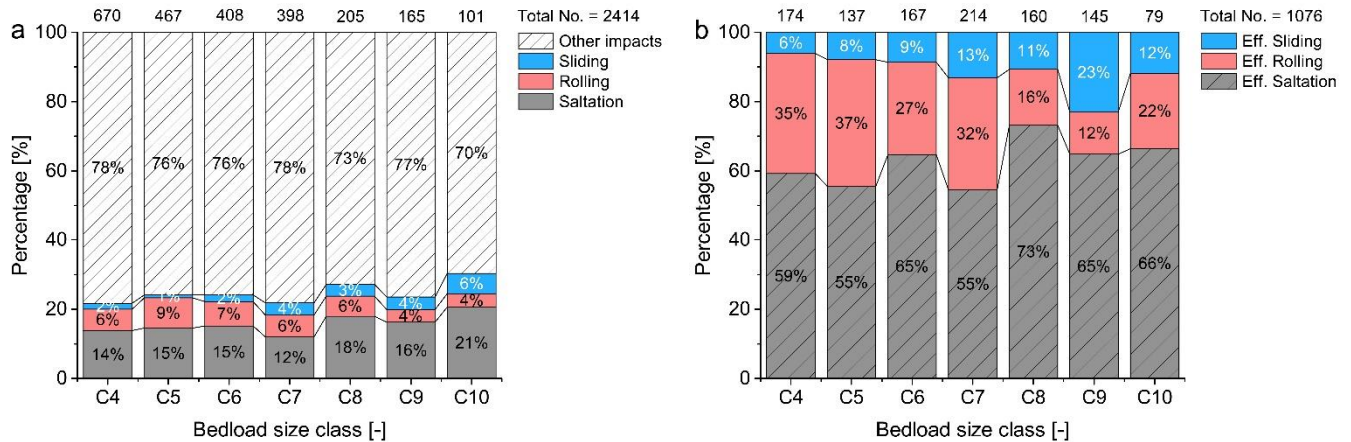
Figure 6: Percentage of impacts number for the transport mode of saltation, rolling and sliding. (a) The total impacts and the percentage of real impacts on the geophone plates for each transport mode. (b) The percentage of effective impacts for all
