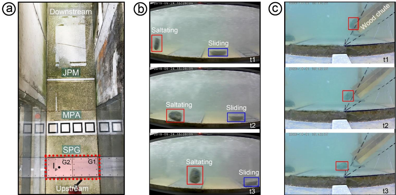
100 Figure 1: Measuring site at the Obernach experimental flume. (a) Measuring reach with different types of sensors mounted on the flume bed, including the Swiss plate geophone (SPG), the miniplate accelerometer (MPA) and the Japanese pipe microphone (JPM). (b) Frames from video recorded during a controlled flume experiment, used for the tracking of particles (mean b-axis = 127.9 mm) impacting onto and moving over the SPG plates. The particle marked with the red rectangle is transported in saltation, while the one marked with the blue rectangle is sliding. (c) Frames from video recorded during a drop 105 experiment with a wood chute inclined at an angle of 45°. G1 and G2 in (a) are two plates of the SPG system, and the black dot I_p marks the impact location of the bedload particles on the plate G2 for the inclined chute experiments. The time interval between consecutive frames for each column in (b) and (c) is 1/3 s. The length of the geophone plate in flow direction is 0.36 m.
