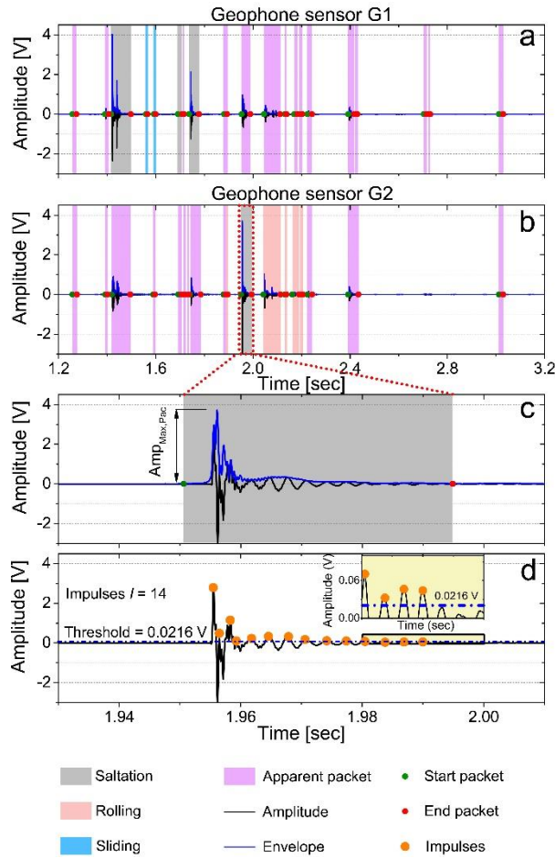
250 Figure 5: Illustration of the SPG vibrations and signal packets for different transport modes following a flume experiment with bedload particles of grain-size class C9. (a) and (b) represent signals that were recorded by geophone sensor G1 and G2, respectively, with a flow velocity of 3.3 m/s. (c) Illustration of the packet definition as the envelope (blue line) of the raw signal, computed with the Hilbert transform, and representing one impact of a saltating particle. (d) Definition of impulse counts I ( = 14 ), counting the times the signal exceeds the threshold (0.0216 V, see the blue dash-dotted line) in the positive domain.
