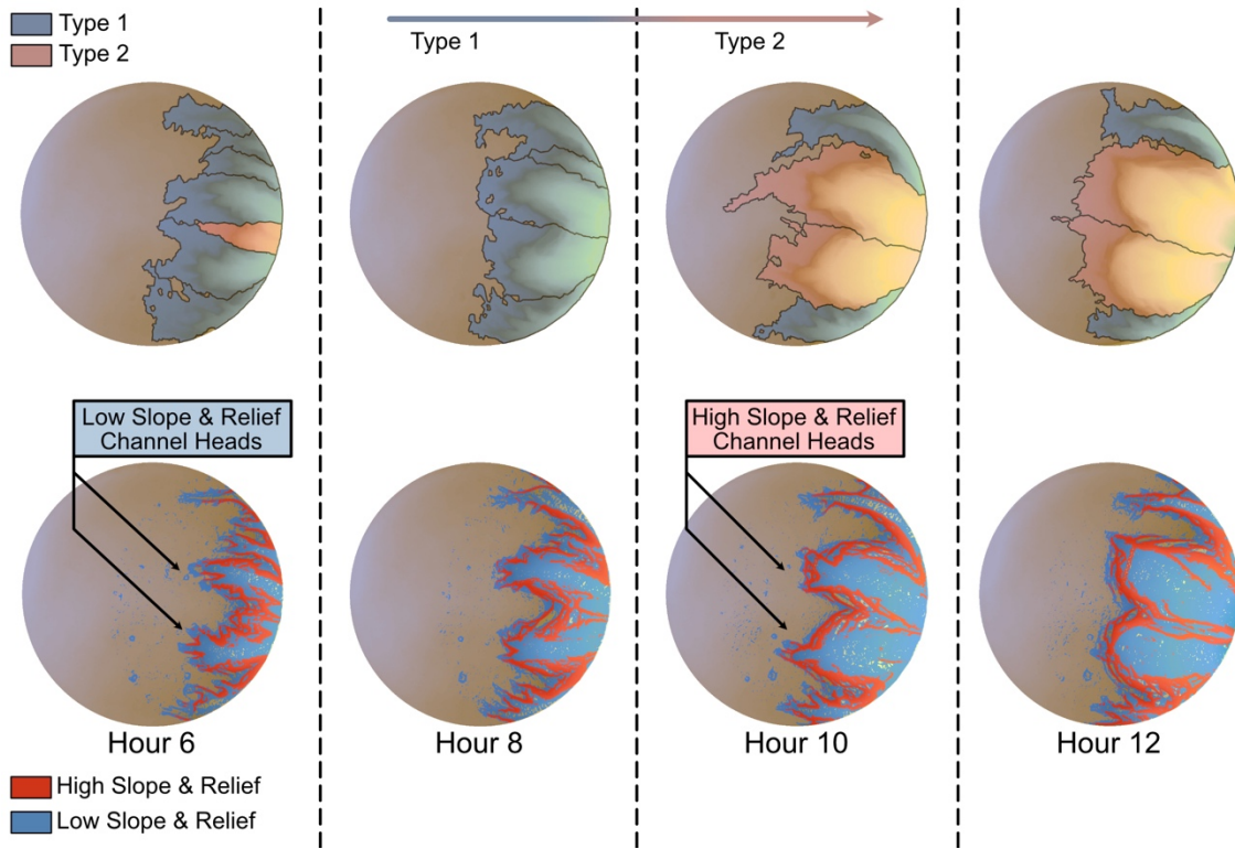
Figure 5. An example of assigning channel types based on the slope and relief classification of channel heads during Run 3. At hour 6, all but one channel was classified as Type 1 because cells in the vicinity of channel head were classified as “Low Slope & Relief.” At hour 8, more cells were classified as “High Slope & Relief” near channel heads, but several cells remained “Low Slope & Relief,” maintaining Type 1 classification. From hour 10 onwards, all cells at two central channel heads were classified as “High Slope and Relief,” therefore the channels were classified as Type 2.
