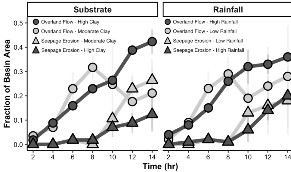
390 Figure 10. Average channelized area of overland flow and seepage channels normalized by total basin area through time for experiments with moderate or high clay substrate (left) and low or high rainfall (right). After hour 8, seepage erosion channelized area increased to a greater extent under a moderate clay substrate than high clay substrate. High clay substrates and high rainfall rates resulted in greater overland flow channelized area. Error bars are the standard deviation in the channelized area between experiments at each timestep. Channelized area values are normalized by total basin surface area.
