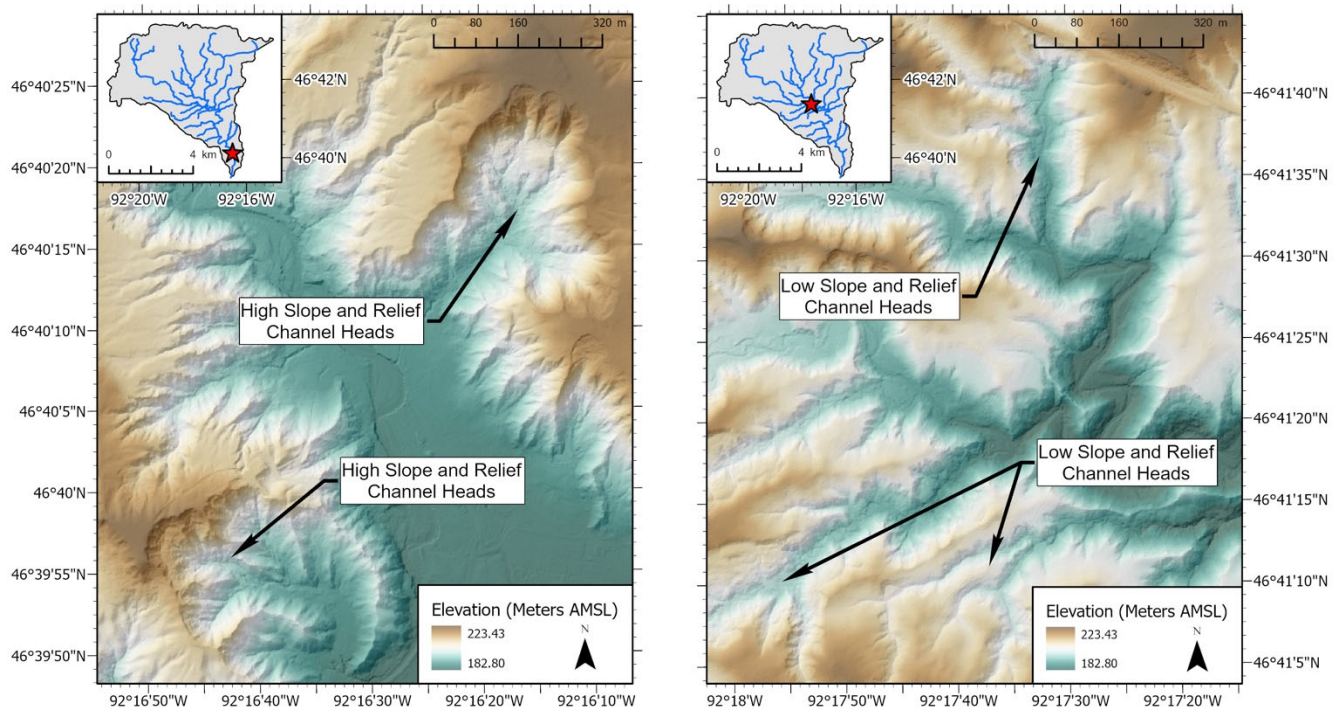
Figure 16. Comparison of channels in the lower (left) and upper portion (right) of the Mission Creek watershed in Fond du Lac, MN. High slope and relief, amphiater-shaped channel heads indicative of seepage erosion are more prominent in the lower portion compared to the upper portion,
