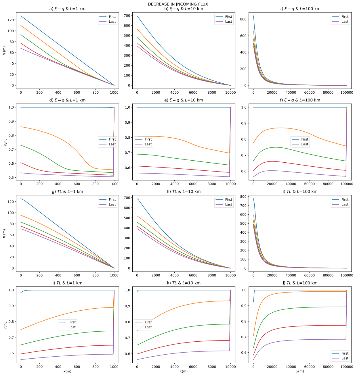
Figure 1: Same as Figure 9 but for a decrease in incoming sedimentary flux by a factor of 2.
