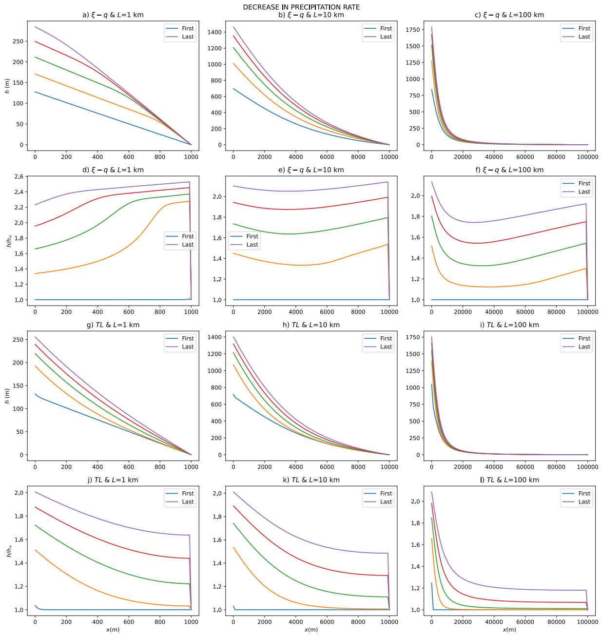
Figure 3: Same as Figure 9 but for a decrease in relative precipitation rate by a factor of 2.
