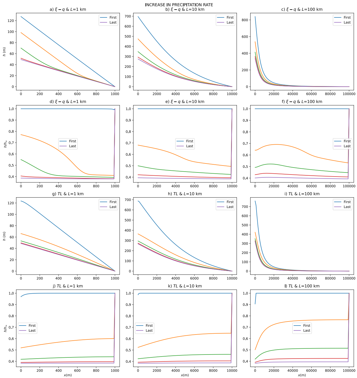
Figure 2: Same as Figure 9 but for an increase in relative precipitation rate by a factor of 2.
