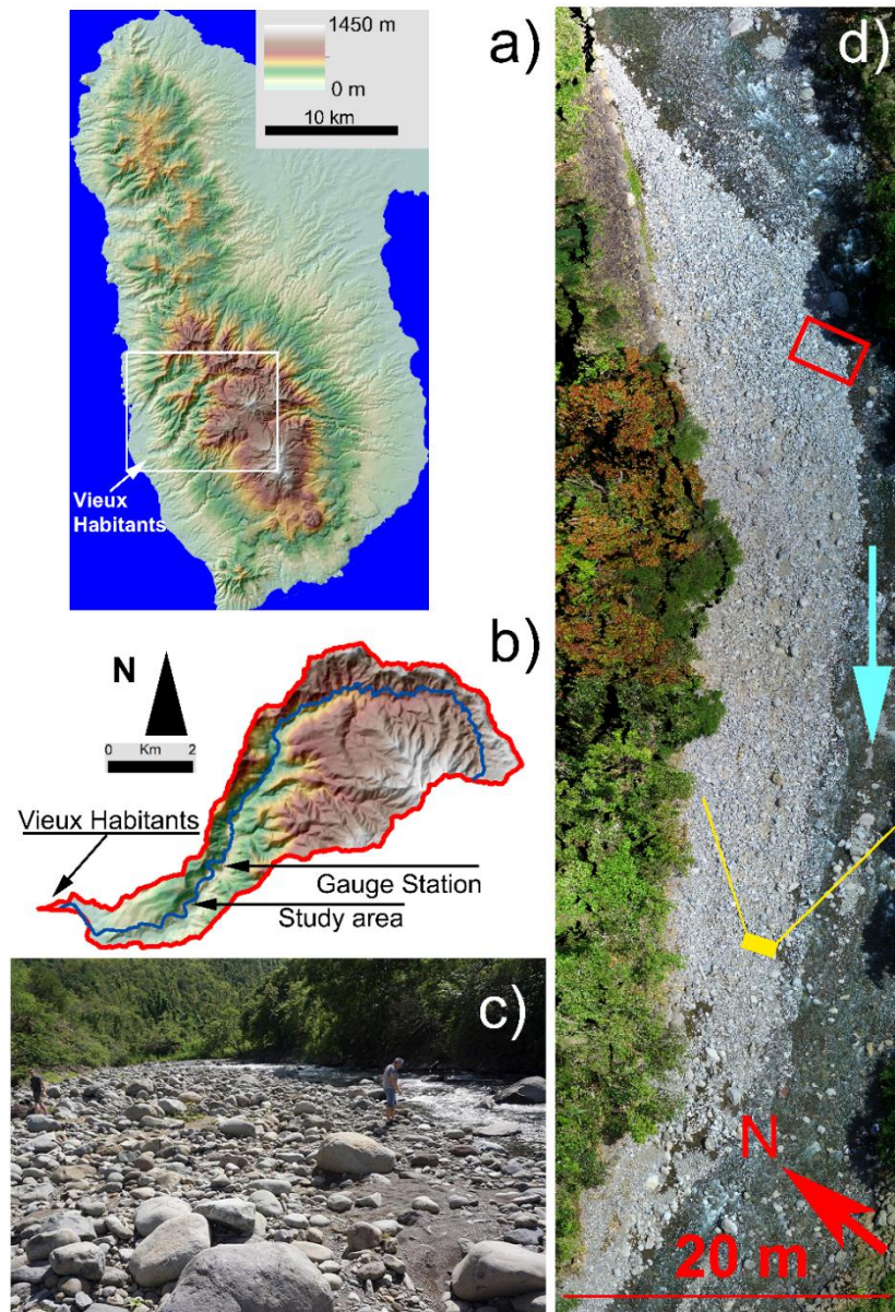
440 Figure 1: a) Basse Terre island in the Guadeloupe archipelago. The island separates the Atlantic Ocean in the East from the Caribbean Sea in the West. The white rectangle shows the position of the map displayed in b). b) The Vieux-Habitants river is located on the Caribbean 445 side of Basse Terre. The watershed of Vieux-Habitants has an area of 19 km 2 . The length of the river is 19 km. The water discharge is measured each 10 minutes at Barthole gauge station. The study area is located 2 km downstream of Barthole. c) A view of the bar from ground looking upstream shows the size of the boulders and their heterometric distribution. The two peoples give the scale d) The area of interest. The bar is about 300 m long and 15 to 35 m wide. It lies on the right side of the river 3 km upstream of the seashore. In fair weather conditions, the bar is bounded on its left by the channel of the river which is 5 to 10 m wide and less than 1 m deep. The boulder bar is flooded 1 to 3 times a year. The red square shows the location of Fig. 3. The position of the camera and the field of view of c) is shown in yellow. The flow direction is given by the turquoise arrow.
