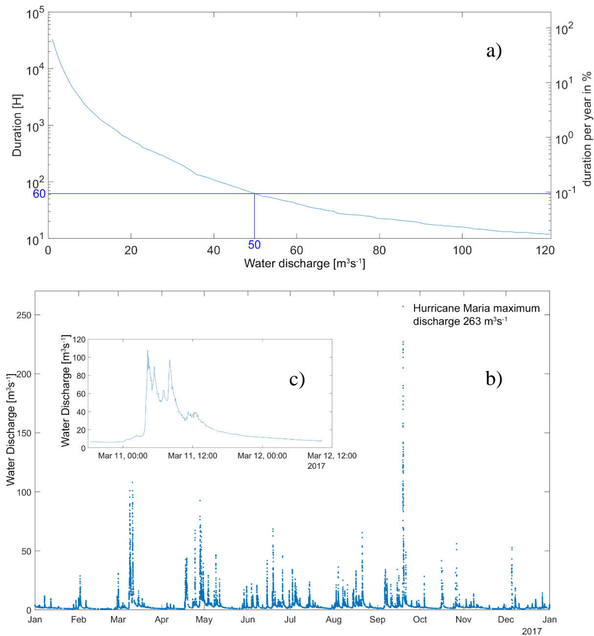
450 Figure 2: a) Duration of the water discharge above a given threshold from 2011 to 2018. A flow of 50 \text{ m}^3 \text{ s}^{-1} was exceeded around 60 hours during the 8 years of measurement (about 0.1% of the total time). b) Hydrogram of year 2017. In low flow conditions, that is most of the time, the discharge is less than 5 \text{ m}^3 \text{ s}^{-1} . The largest discharge recorded in 2017 was 263 \text{ m}^3 \text{ s}^{-1} . It was reached on September 19 during hurricane Maria. c) The inset shows a typical flood. The water discharge reaches its maximum in less than one hour. The peak of the flow is followed by a slow recession toward low flow. 455
