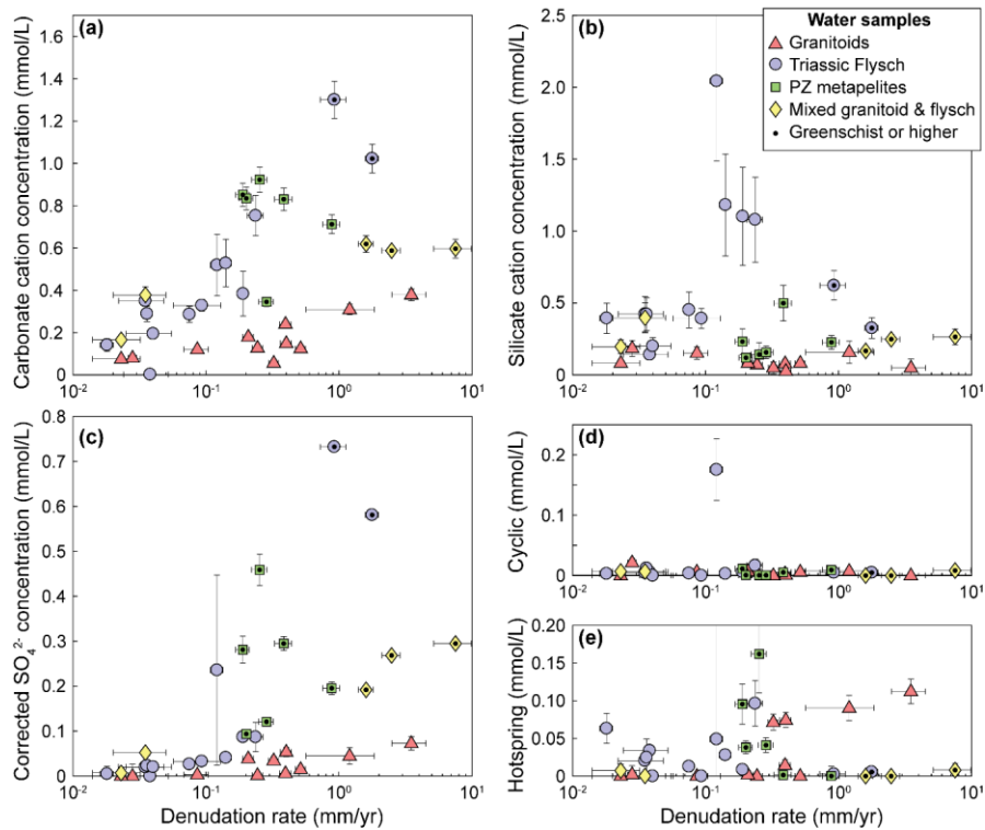
Figure 5: Unmixed contributions to the solute load
