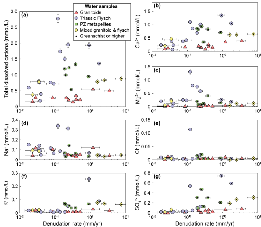
Figure 4: Solute concentrations vs. denudation rate (a) Total dissolved cations. Spearman's rank correlation coefficient and associated p-value: \rho_{granite}^{TDC} = 0.43 , p_{granite}^{TDC} = 0.19 ; \rho_{flysch}^{TDC} = 0.63 , p_{flysch}^{TDC} = 0.03 . (b) Ca^{2+} concentrations \rho_{granite}^{Ca^{2+}} = 0.63 , p_{granite}^{Ca^{2+}} = 0.04 ; \rho_{flysch}^{Ca^{2+}} = 0.73 , p_{flysch}^{Ca^{2+}} = 0.006 . (c) Mg^{2+} concentrations. (d) Na^{+} concentrations. (e) K^{+} concentrations. (f) Cl^{-} concentrations. (g) SO_4^{2-} concentrations \rho_{granite}^{SO_4^{2-}} = 0.80 , p_{granite}^{SO_4^{2-}} = 0.003 ; \rho_{flysch}^{SO_4^{2-}} = 0.76 , p_{flysch}^{SO_4^{2-}} = 0.004 . Catchments underlain by different lithologies are distinguished by symbols and color. Datapoints with a black dot are metamorphosed to greenschist facies or higher.
