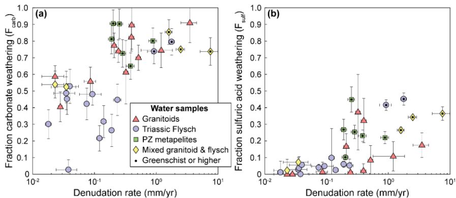
Figure 6: Fraction of carbonate weathering and weathering by sulfuric acid (a) Fraction of carbonate weathering (eq. 23). (b) Fraction of weathering by sulfuric acid (eq. 24). Symbols indicate catchment lithology. Catchments underlain by different lithologies are distinguished by symbols and color. Datapoints with a black dot are metamorphosed to greenschist facies or higher.
