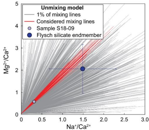
Figure A2: Example of mixing lines from Monte Carlo modelling in \text{Na}^+/\text{Ca}^{2+} – \text{Mg}^{2+}/\text{Ca}^{2+} space Monte Carlo Iterations of the mixing model for sample S18-09 (small light-blue point). Flysch silicate endmember and 1\sigma uncertainty in dark blue. 1000 out of 100,000 (1%) of mixing lines from the Monte Carlo modelling marked as grey lines. Red lines show all runs with \chi^2_{total} \leq 1 among those 1% of runs.
