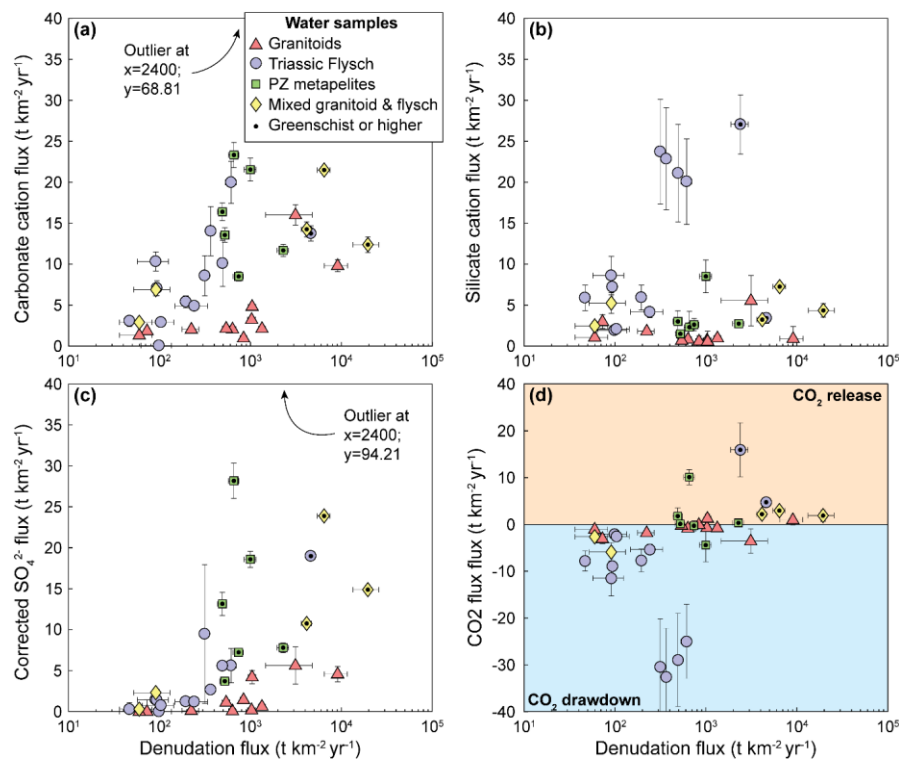
Figure A6: Inferred weathering fluxes
