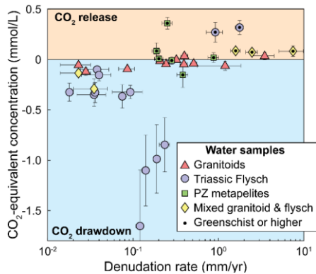
Figure 7: Influence of weathering on the carbon cycle Equivalent concentration of CO 2 released or consumed. Symbols indicate catchment lithology. Catchments underlain by different lithologies are distinguished by symbols and color. Datapoints with a black dot are metamorphosed to greenschist facies or higher.
