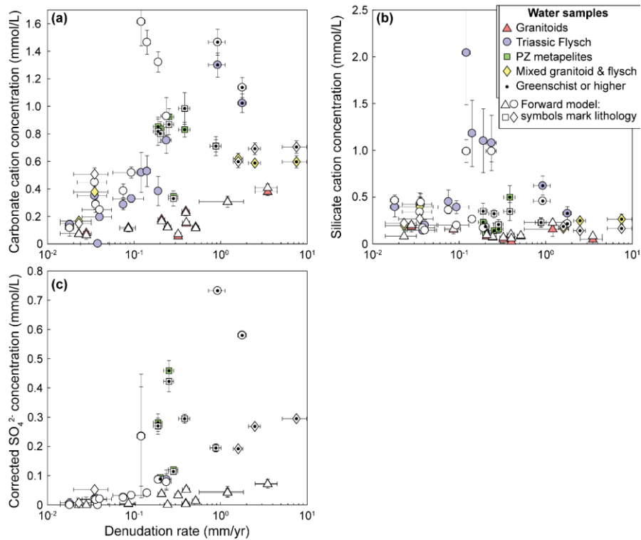
485 Figure A4: Forward model results for silicate, carbonate, and sulfide weathering contributions
