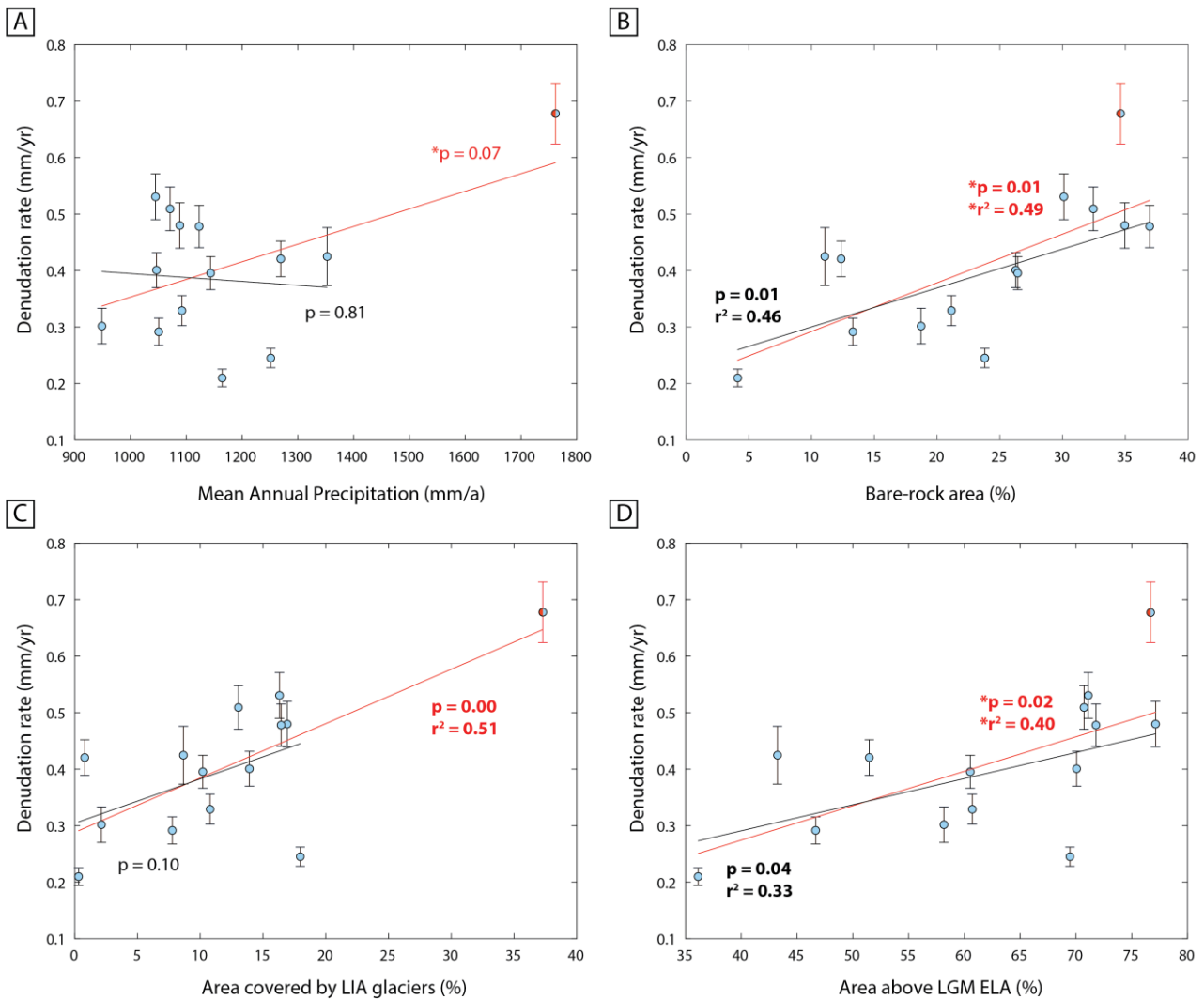
Figure 5: Relationships between tributary-catchment denudation rates and catchment (A) mean annual precipitation, (B) relative bare-bedrock area, (C) relative area covered by LIA glaciers, and (D) relative area above LGM ELA (2103 m a.s.l.). Correlations have been calculated including or not sample DB01 (red and black lines, respectively; see text for discussion). Correlation coefficients (p-value and r^2 ) are reported for each linear regression with statistical significance (p-value < 0.05). r^2 is not reported for non-significant correlations (p-value > 0.05). Asterisks indicate linear correlations for which DB01 has been considered as an outlier (based on Cook's distance, Table S3).
