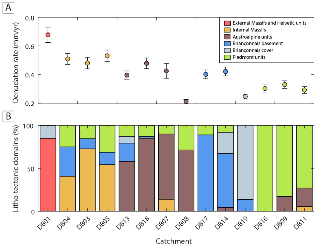
305 Figure 6: Tributary-catchment denudation rates (A) and relative proportion of litho-tectonic units within the quartz-bearing areas of the individual catchments (B). Colour code in (A) refers to the most abundant litho-tectonic unit in each individual catchment (see Figure 2 for spatial distribution of the different litho-tectonic units).
