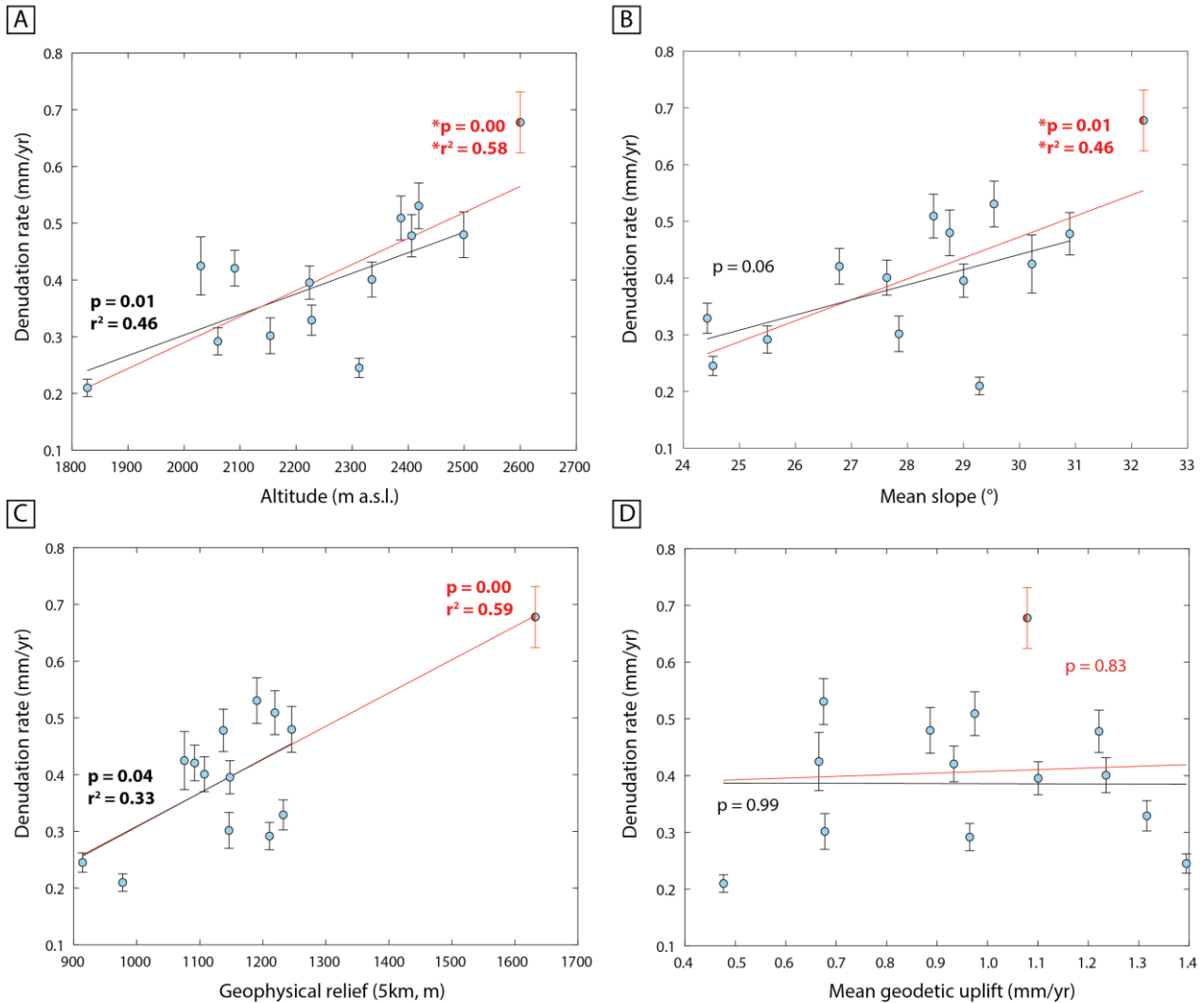
275 Figure 4: Relationships between tributary-catchment denudation rates and mean catchment (A) elevation, (B) slope, (C) 5-km geophysical relief, and (D) geodetic uplift. Linear correlations have been calculated including or not sample DB01 (red and black lines, respectively; see main text for discussion). Correlation coefficients ( p -value and r^2 ) are reported for each linear regression with statistical significance ( p -value < 0.05 ). r^2 is not reported for non-significant correlations ( p -value > 0.05 ). Asterisks indicate linear correlations for which DB01 has been considered as an outlier (based on Cook's distance, Table S3).
