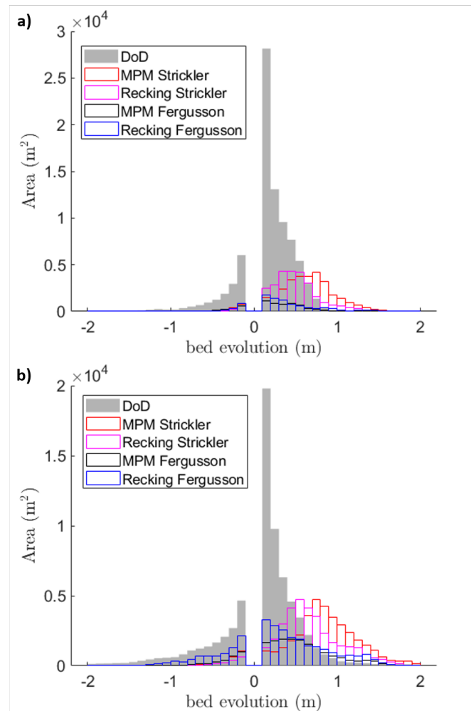
Figure 15. Statistical distribution of erosion/deposition. The grey histogram shows observed morphological change and the colored ones show model predictions with the different bedload and friction equations within the LDG a) and upstream the LDG b).
