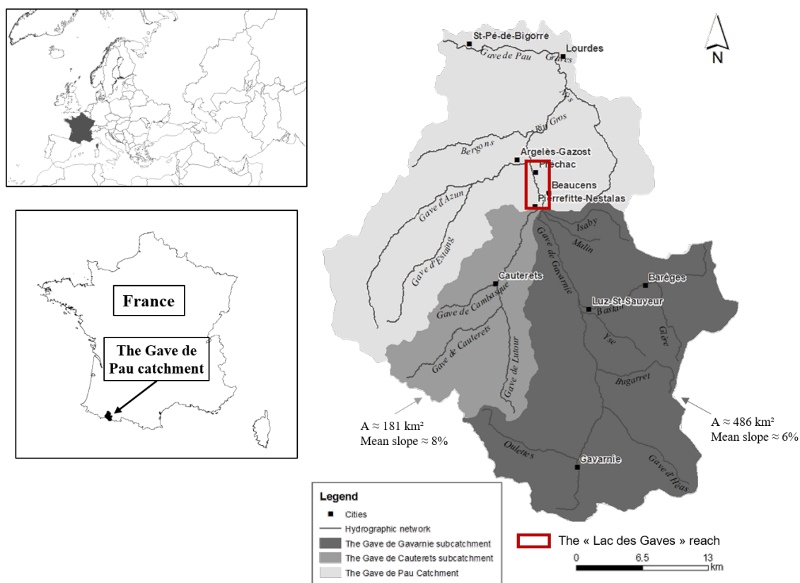
Figure 1. The "Gave de Pau" catchment and its main upstream sub-catchments: the "Gave de Caunterets" and the "Gave de Gavarnie" sub-catchments (A is the drainage area and the mean slope of the watercourses is also introduced). The LDG reach is represented by the red rectangle between the cities of Pierrefitte-Nestalas and Argelès-Gazost, Hautes-Pyrénées, France
