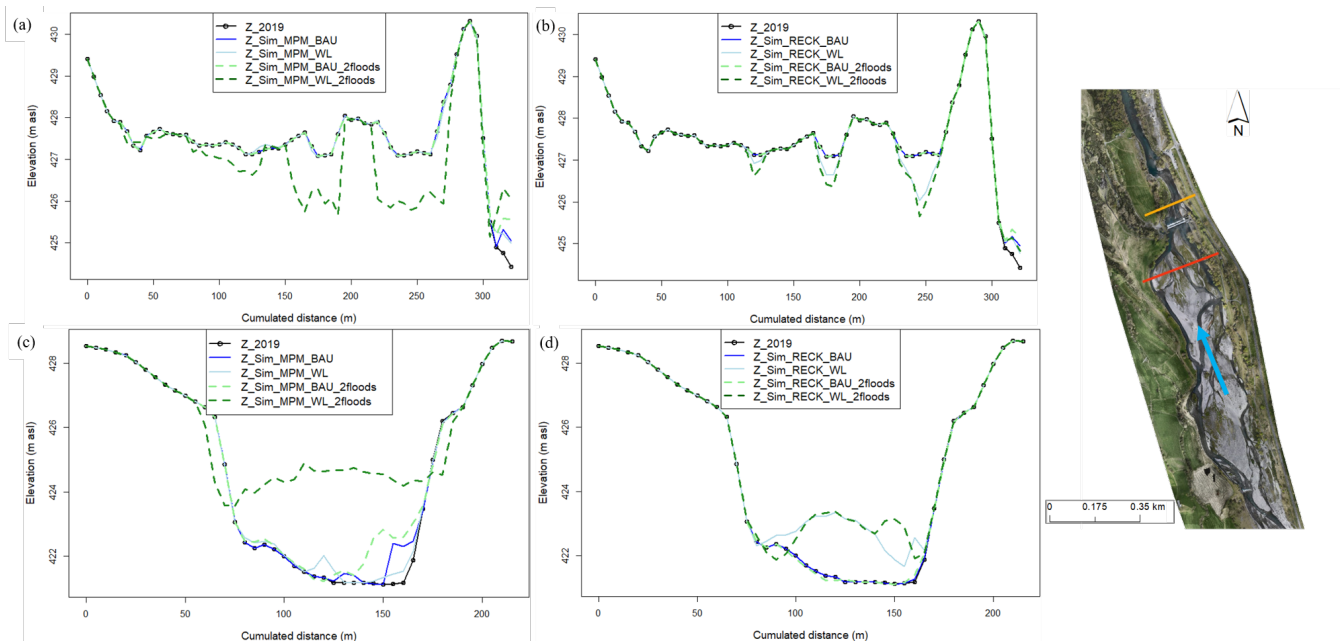
Figure 16. (a) and (b) are the simulated cross sections for the MPM formula and Recking formula respectively upstream the Préchat weir (red cross-section on the right) for the BAU and the WL scenarios. (c) and (d) are the simulated cross-sections for the MPM formula and the Recking formula respectively downstream the Préchat weir (orange cross-section on the right) for the same scenarios. Z_{2019} represents the LiDAR DEM surveyed in 2019 that is the initial topography.
