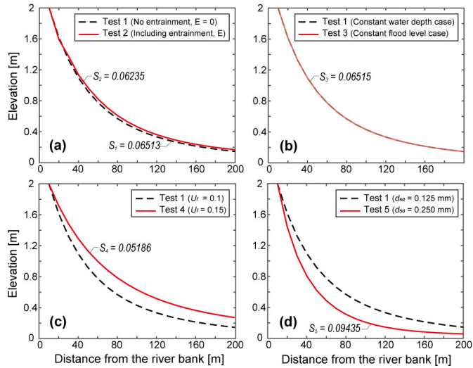
285 Figure 3. Levee surface profiles taken at the end of each model. The black dotted line represents the results of Test 1 and the red 290 lines are other test results.
