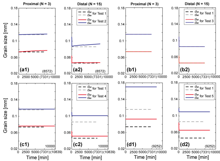
340 Figure 6. Time series of grain sizes d_{50} and d_{90} at the top levee surface at the proximal ( N = 3 , x = 30 m) and distal ( N = 15 , x = 150 m) locations marked with each simulation time, T in parenthesis . The red and blue solid lines indicate the grain sizes d_{50} and d_{90} for each test, and the black and grey dotted lines are for Test 1, respectively.
