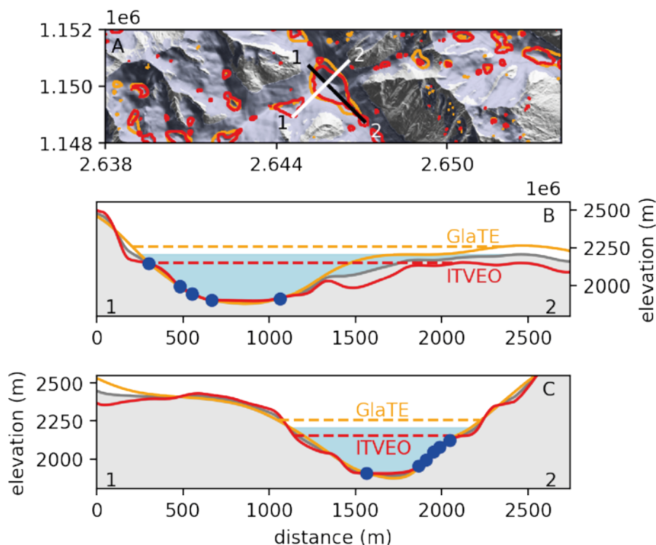
Figure 6 (A) Comparison between the potential lakes detected by GlaTE (orange) and ITVEO (red) in the Aletsch region. The glacier area of the SGI2016 is marked in blue. The black and white lines provide the locations of the profiles displayed in panels B and C, respectively. (B-C) Illustration of the bedrock topography (orange: GlaTE; red: ITVEO; grey: mean) for the profiles given in panel A. GPR measurements are indicated (blue dots) together with the lake levels resulting from the three topographies (blue is the lake for the mean topography).
