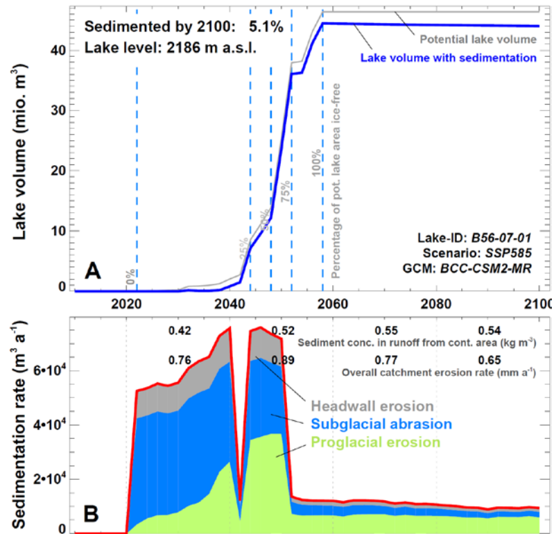
Figure 5 Temporal dynamics of lake volume growth and modelled sedimentation for the example of Gornergletscher (SGI-ID B56-07), harbouring the third-largest new glacier lake in Switzerland (cf. Table 1). Results refer to a selected GCM amid the climate scenario SSP585. (A) Lake volume evolution when neglecting (grey) or accounting for (blue) sedimentation. Percentages of exposed potential maximum lake area over time are shown (grey vertical numbers). (B) Modelled lake sedimentation rate, including the partitioning of the three considered sediment sources (cf. Section 3.3). The strong temporal variations are due to the appearance and re-filling of smaller glacier lakes located above the considered lake. Numbers in the upper part of the panel show (i) sediment concentrations in the runoff from the catchment area contributing to the lake at a given point in time, and (ii) modelled catchment erosion rates. The numbers are evaluated over 20-year time steps.
