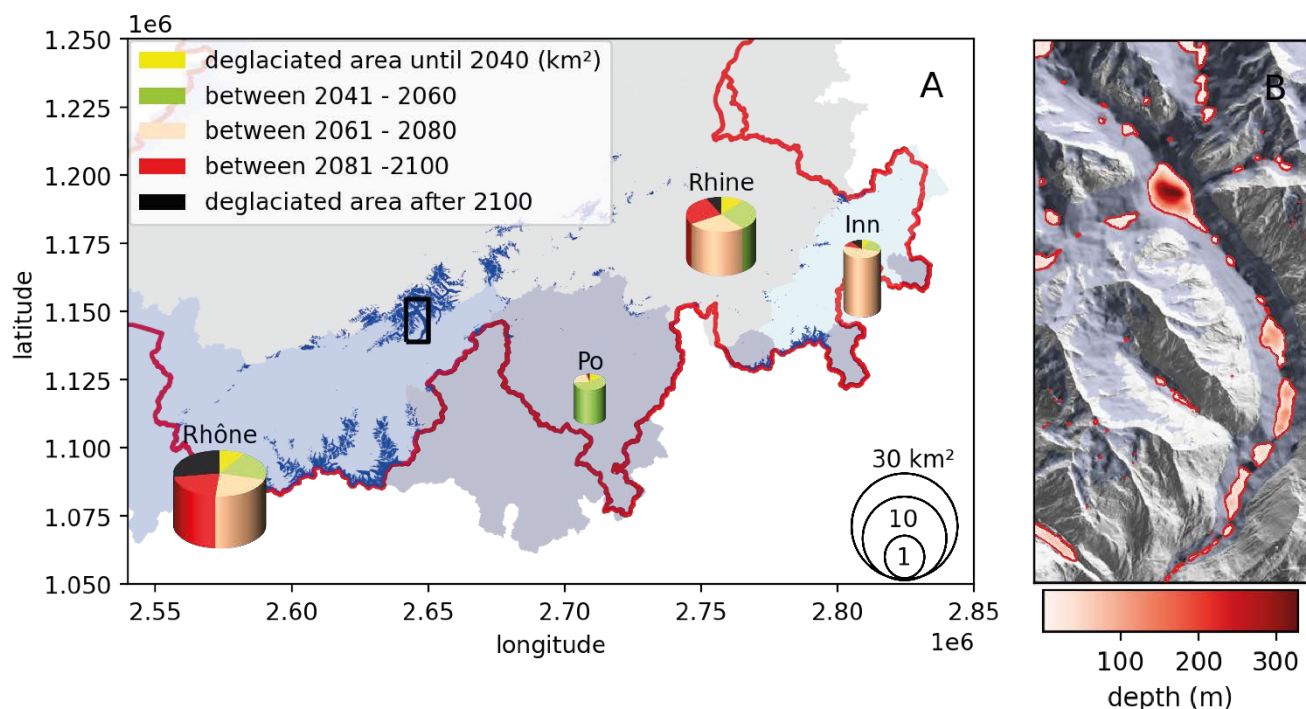
Figure 1 (A) Map of Switzerland showing the four main river basins (background colours) used for aggregating the results. Glacier extents according to the SGI2016 (Linsbauer et al., 2021) are shown in dark blue. For each catchment, the temporal evolution of the total area of the detected potential glacier lakes is indicated (pie chart area on logarithmic scale, legend at bottom right). The results are given in 20-year intervals (see legend at top left) and correspond to the simulations driven by the median scenario SSP245. Sedimentation is neglected in this graph. The height of the pies indicates the mean depth of the potential lakes within a given catchment. The black box shows the area enlarged in panel B. (B) Map of the lower part of Grosser Aletsch glacier, illustrating the morphology of potential glacier lakes. Lakes are contoured in red with depths given by the reddish colours. The SGI 2016 glacier extent (blueish background) is given together with a relief of the swissALTI3D surface DEM and the subglacial topography (grey shading).
