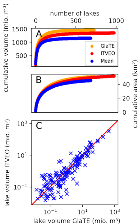
Figure 5 Cumulative (A) volume and (B) area of all potential lakes detected with GlaTE (orange), ITVEO (red), and the mean bedrock topography (blue). (C) Comparison of the volume of potential lakes per glacier detected with GlaTE and 515 ITVEO. Along the red line, the volume calculated with the two models is equal. Note the logarithmic scale.
