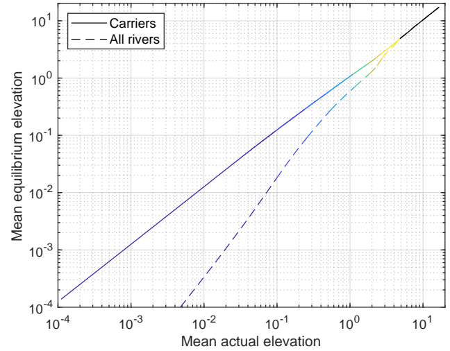
Figure 8. Mean equilibrium elevation vs. mean actual elevation for carriers (solid lines) and all rivers (dashed lines). The data were obtained from averaging over lines in the x_2 -direction and over 401 snapshots. The colors refer to the regions defined in Fig. 1.
