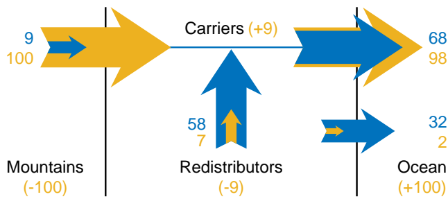
Figure 14. Balance of water and transported sediment for the scenario with instantaneous consolidation ( K_d = K_t = 1 in the erosive regime). Blue arrows describe discharges, equivalent to catchment sizes. The values are normalized to the total catchment size and expressed in percent, so that 100 corresponds to the total catchment size. Orange-colored arrows describe sediment fluxes normalized to the sediment flux from the mountain range (also expressed in percent). The numbers in parentheses describe the sediment balances of the individual system components.
