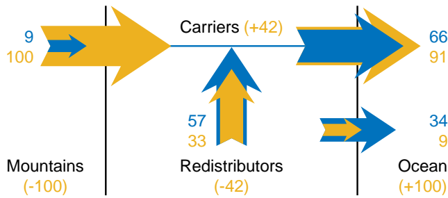
Figure 9. Balance of water and transported sediment. Blue arrows describe discharges, equivalent to catchment sizes. The values are normalized to the total catchment size and expressed in percent, so that 100 corresponds to the total catchment size. Orange-colored arrows describe sediment fluxes normalized to the sediment flux from the mountain range (also expressed in percent). The numbers in parentheses describe the sediment balances of the individual system components.
