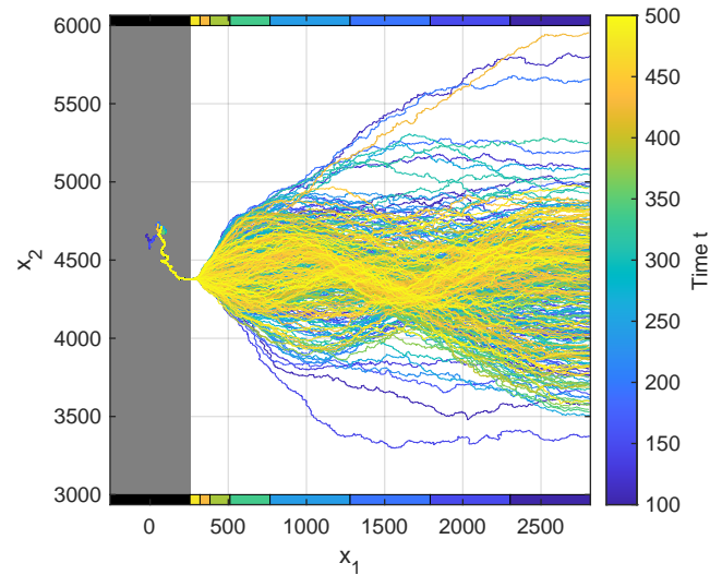
Figure 4. Snapshots of the river with the largest catchment at the edge of the mountain range (orange-colored line in Fig. 1). The gray-shaded area depicts the mountain range.
