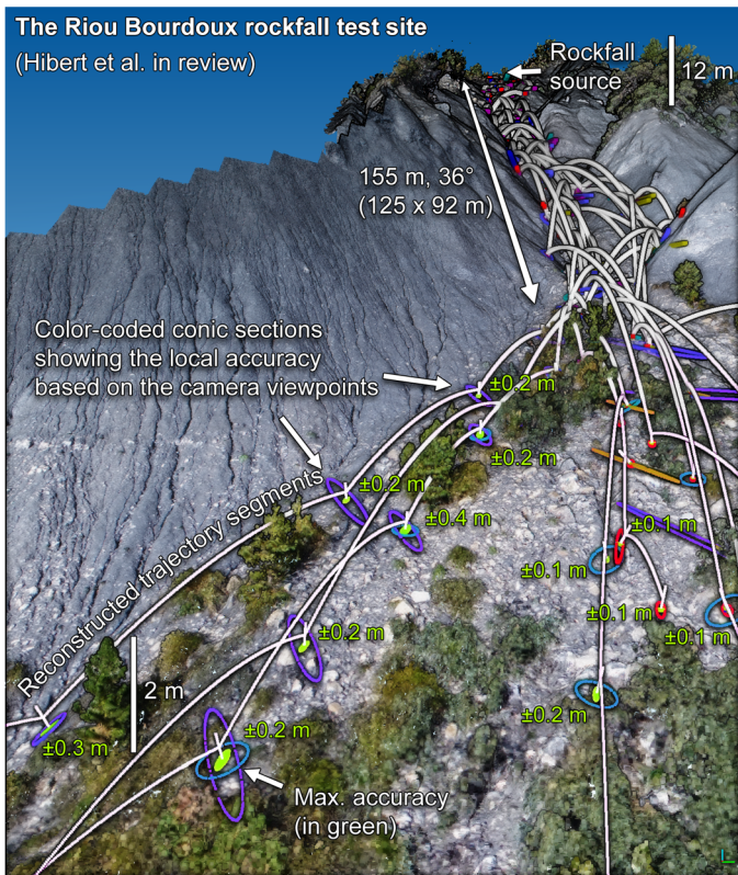
270 Figure 4: Examples of spatial accuracies from the projection of \pm 4 px picking accuracies for the Riou Bourdoux rockfall test site that involved multiple ground based and airborne camera viewpoints (Hibert et al. in review). The maximized local precision and accuracy of the 376 constrained areas of the overlapping ellipses are shown in bright green like in the previous figure. The maximal sizes (worst values) of some maximized local accuracies are written in bright green next to their impacts. Note that each impact accuracy is unique and depends on many variables like the impacted terrain geometric configuration and texture, its distance from the viewpoints and the video acquisition setup that influence locally the ease of visually identifying the impact location.
