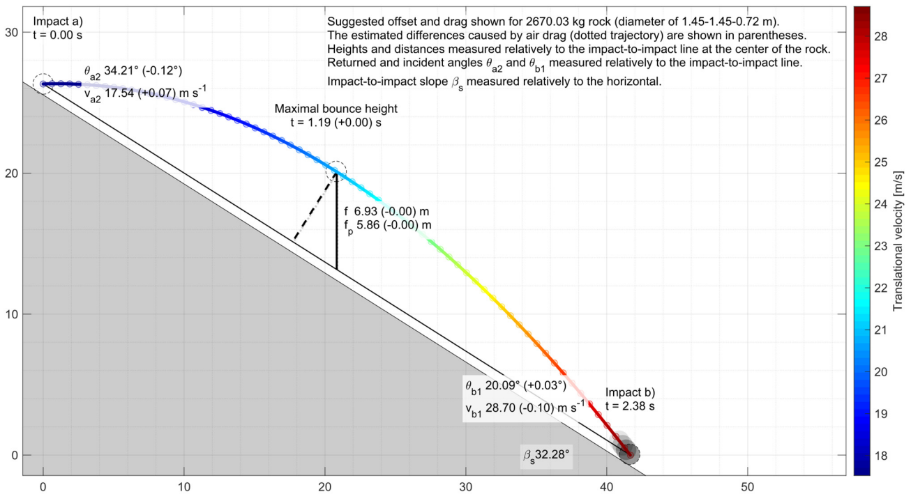
750 Figure A3: 2D vertical profile of the longest parabola of r1 reconstructed with and without air drag.
