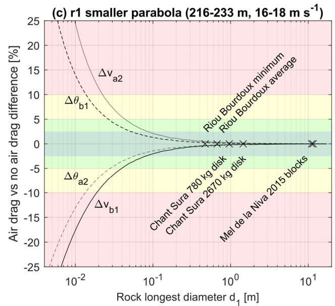
730 Figure A2: Chosen parabolas to evaluate the significance of air drag on the reconstructed results and the positioning and timing precision in Appendix B. Note that \theta_{a2} and \theta_{b1} are calculated relatively to the impact-to-impact line in 2D vertical profiles and not in 3D in that case. The differences when comparing the reconstructed incident and returned velocities and angles with vs. without drag for different rock sizes are shown in the graphs. Cross markers are placed as indicative rock d_1 diameters as references for the Riou Bourdoux test site (Hibert et al., in review), the Chant Sura test site (Caviezel et al. 2019, 2020, 2021; Sanchez and Caviezel, 2020), and the Mel de la Niva Mountain 2015 rockfall event (Noël et al., in preparation; Lu et al., 2018).
