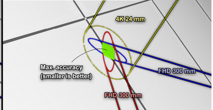
Figure 3: Conceptualization of the spatial accuracy from projecting the picking accuracy to the terrain. The picking accuracy is degraded to \pm 100 px to better illustrate the concept. In reality, the precision and accuracy depend on the resolving power and the acutance of the lens used, sensor size and resolution, general quality and sharpness of the footage and ease at distinguishing the rock projectile from the background. The elongation of the resulting conic section ellipses depends on the viewing “incident angle” with the terrain. The accuracy is maximal when the ellipses are small and not elongated, but they can also be maximized by combining two or more viewpoints. The size of the projected pixels depends on the resolution and the FOV used. The local accuracy can be better, even at a lower resolution, by using lenses with a small FOV. This also helps to distinguish the rock from the background, improving the picking precision and accuracy, which in turn also improves the local precision and accuracy.
