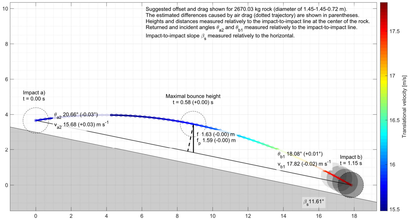
760 Figure A4: 2D vertical profile of the smaller parabola of r1 reconstructed with and without air drag.
