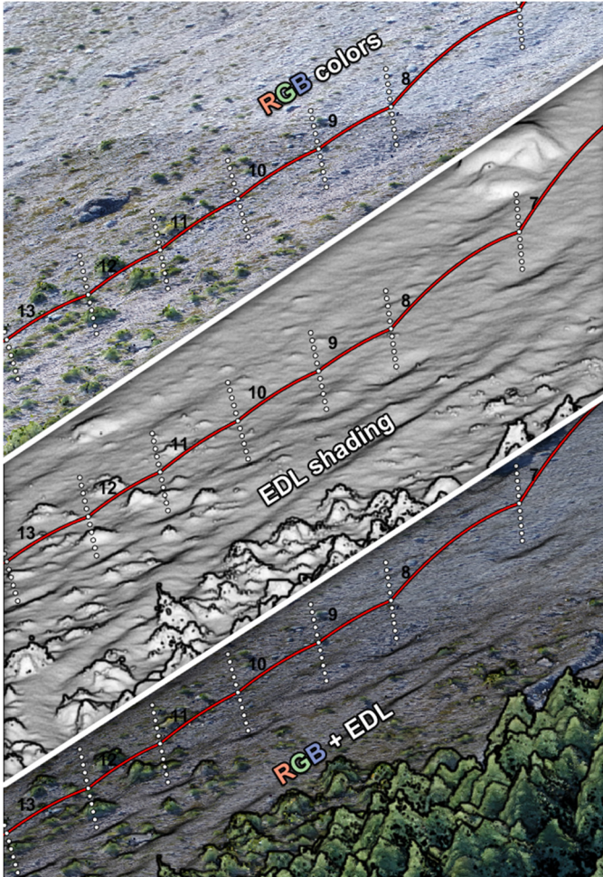
385 Figure 8: Same 3D scene with different rendering settings of the 3D terrain model. The EDL shading filter can be very useful for highlighting artifacts and impact marks. The scenes are rendered in a custom tool developed to help assist the reconstruction process, as later described. The trajectory under reconstruction shown in red with white dotted normal vectors from each impact mark visible on the ground corresponds to the block with the longest runout from the 2015 Mel de la Niva rockfall event (Noël et al., in preparation; Lu et al., 2018). It transitions from longer freefalling phases to a “rolling-bouncing” phase.
