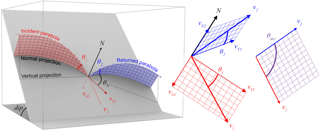
170 Figure 2: Geometric configuration at impact of the reconstructed translational velocity vectors and the related angles (see Table 1 for the variable's descriptions). Note that such angles are measured based on the normal vector to the terrain (N) and not to the vertical. For a perfectly reflected impact, such as a light beam on a flat mirror, the incident and the returned velocity vectors ( v_1 and v_2 ) would be coplanar with N. Here, the lateral deviation ( \theta_N ) is measured as the angle around N making v_2 deviate from the previous coplanar situation. Note that this rotation axis should be tilted slightly toward where the rock projectile is from depending on the amount of scarring, slipping, and skidding, but it is kept around N for simplicity. The total deviation ( \theta_{dev} ) 175 is simply measured as the angle between v_1 and v_2 . It is close to the sum of the incident and the returned angles ( \theta_1 and \theta_2 ) when \theta_N is small.
