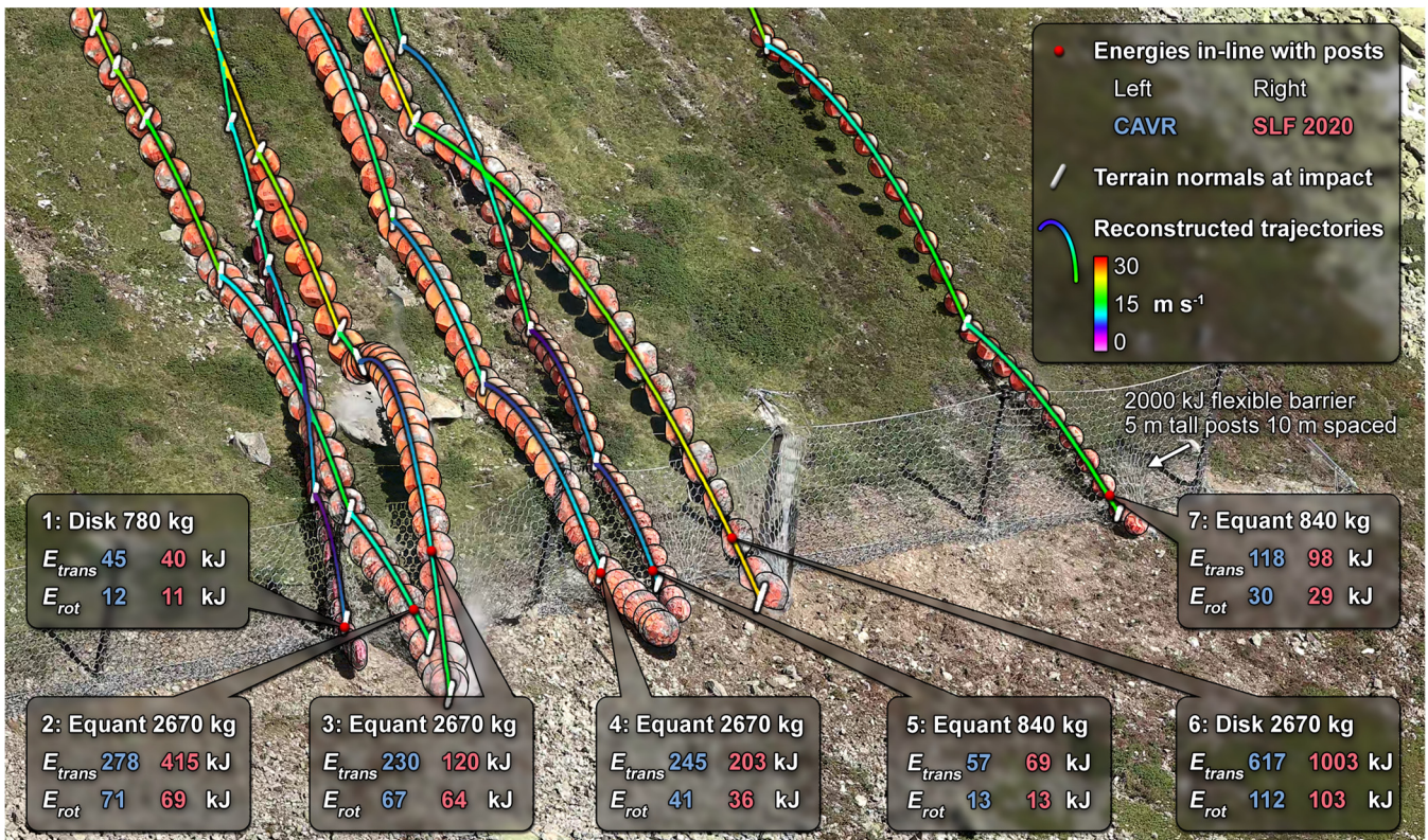
600 Figure 12: Reconstructed trajectories using the CAVR method overlaid on the stacked video frames of the different rockfall runs from the SLF experiment performed on 2019 September 13 th . One frame out of ten is shown for each trajectory from the 119.88 fps footage captured with the FHD camera setup shown in Fig. 6. All these rocks that are intercepted by the flexible ROCCO barrier from Geobruigg are stopped (Sanchez and Caviezel, 2020). The reconstructed energies in line with the posts from both methods are put side-by-side.
