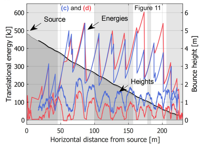
535 Figure 10: Side-by-side comparison of the reconstructed translational velocities, positions, translational energies, and bounce heights of the reconstructed trajectories with the CAVR method compared to the older trajectories from the SLF (Caviezal et al., 2020). The r1 and r2 rockfall runs correspond to the 6 th and 7 th runs performed by the SLF on September 13 th , 2019. The 3D reconstructed trajectories are overlaid on the stacked frames showing the rock positions every 10 frames (every ~1/12 th of a 540 second for the footage captured at 119.88 fps with the camera setup shown in Fig. 6). For scale, the dimensions of the 2670 kg orange reinforced disk or wheel shaped concrete rock are 1.45 m ( d_1 and d_2 ) by 0.72 m ( d_3 ). The reconstructed trajectory segments are shown in black with their respective slope profiles in gray as background elements of the 2D vertical profiles shown in (e) and 545 (f). The characteristic sawtooth shape of the energy profiles helps distinguish them from the bounce heights. The values from the CAVR method are shown in blue while those from the SLF are shown in red for a quantitative comparison. The portion of reconstructed trajectory segments shown over stacked video frames in (a), (b), (c), (d) and in Fig. (11) are highlighted in the 2D profiles (e) and (f) with white vertical bands.
