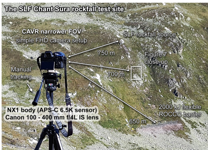
315 Figure 6: Simple camera setup based on the presented acquisition concepts for the CAVR method tested here at the Chant Sura rockfall test site during the September 13 th 2019 SLF experiment. The white rectangle shows the close-up area of the site used in Fig. 7 to compare the SLF RED video footage to the FHD footage from this simple camera setup. The Samsung NX1 camera body from 2014 could deliver 4K UHD footage (6.5K full sensor readout downscaled to 4K), but the lens from 1998 used here does not have the resolving power for the resolution on the ~super 35 / APS-C sized sensor (23.5 x 15.7 mm, crop factor of 1.53). Thus, the footage was recorded at FHD and could reach a higher frame rate instead (119.88 fps).
