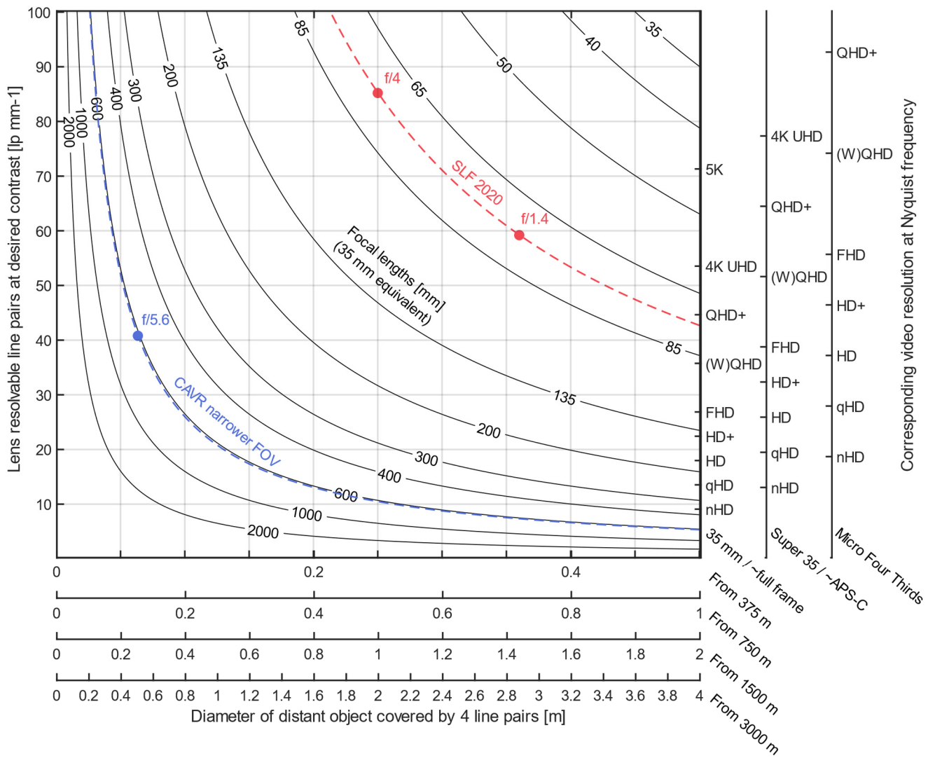
285 Figure 5: Abacus putting in relation to the lens resolvable line pairs given by the modulation transfer function (MTF) to the corresponding video resolution at maximum resolving capacity for different common sensor sizes and perpendicular distant object diameters equivalent to 4 line pairs that can be resolved through lenses of different fields of view (FOVs) given by their 35 mm equivalent focal lengths. The equivalent focal lengths of the Canon at 400 mm and Zeiss 55 mm lenses used on cameras with Super 35 / ~APS-C sensor sizes for the Chant Sura rockfall test site used as an example are shown with blue and red dashed lines. The 290 central MTF values at 50% contrast for the lenses are shown with dots for different aperture values. Unless capturing objects with fine grid patterns where aliasing could be a problem, it is recommended to sample above the Nyquist frequency to avoid being constrained by the camera body/sensor before downscaling to the resolvable video resolution. For example, the Samsung NX1 camera body used for the CAVR method samples at ~6.5K from the whole ~APS-C sensor readout before performing the in-body downscaling).
