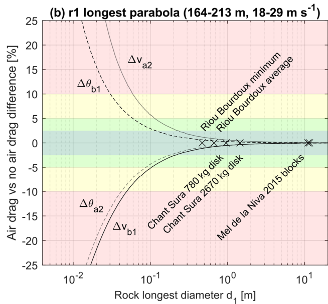
730 Figure A2: Chosen parabolas to evaluate the significance of air drag on the reconstructed results and the positioning and timing precision in Appendix B. Note that \theta_{a2} and \theta_{b1} are calculated relatively to the impact-to-impact line in 2D vertical profiles and not in 3D in that case. The differences when comparing the reconstructed incident and returned velocities and angles with vs. without drag for different rock sizes are shown in the graphs. Cross markers are placed as indicative rock d_1 diameters as references for the Riou Bourdoux test site (Hibert et al., in review), the Chant Sura test site (Caviezel et al. 2019, 2020, 2021; Sanchez and Caviezel, 2020), and the Mel de la Niva Mountain 2015 rockfall event (Noël et al., in preparation; Lu et al., 2018).
