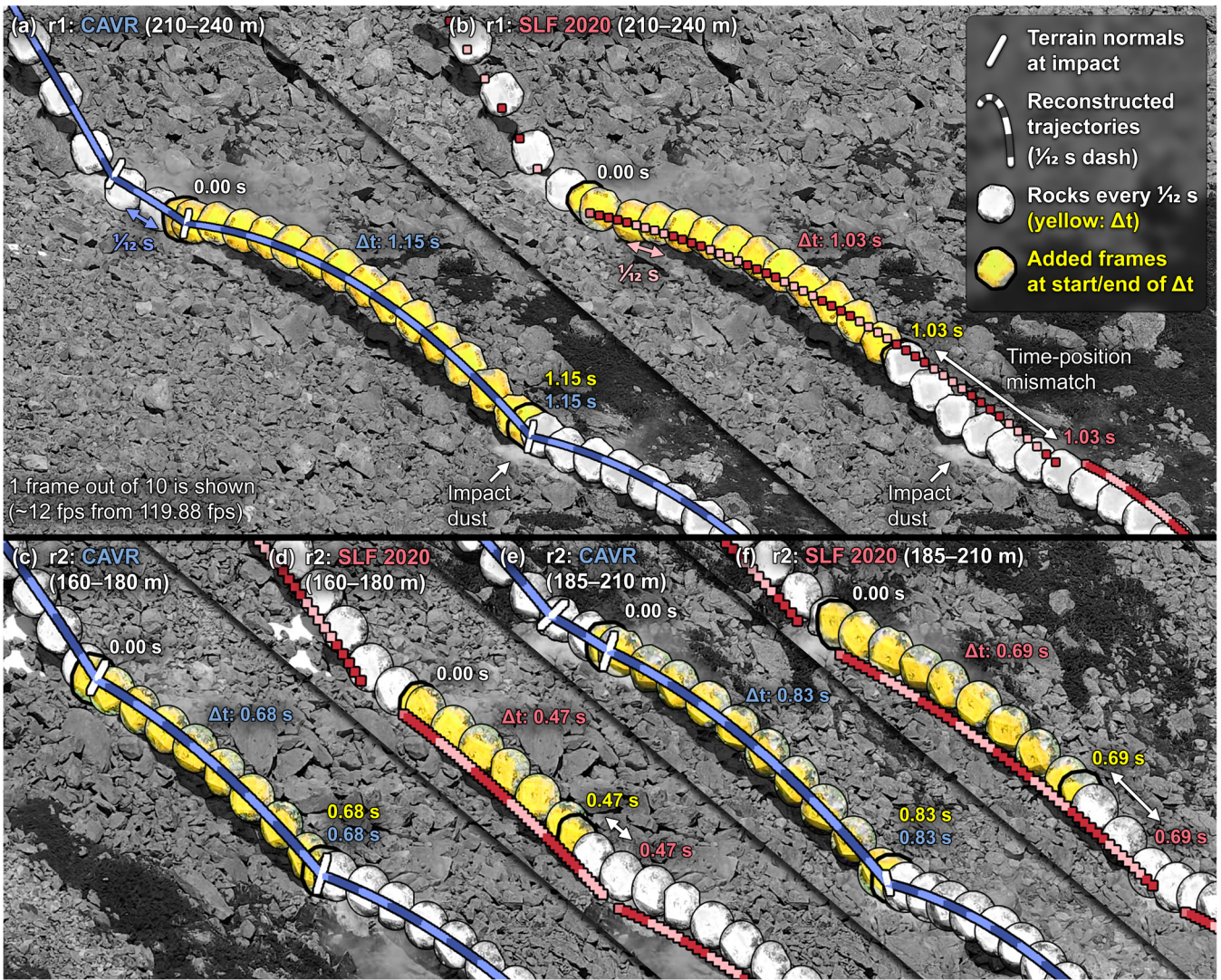
580 Figure 11: Detailed portion of the three abnormally mismatching reconstructed trajectory segments previously highlighted in Fig. 10e and Fig. 10f. The reconstructed trajectories repeatedly change colors every 1/12^{\text{th}} of a second. They are overlaid on the stacked video frames showing the rock's position every 10 frames (every \sim 1/12^{\text{th}} of a second for the footage captured at 119.88 fps). 585 The rocks from the frames corresponding to the chosen period for the three freefalling phases with the energy mismatches are colored in yellow. The visible rocks in yellow from the added frames corresponding to the beginning and the end of the chosen period for the reconstructed parabola are highlighted with a thicker black contour.
