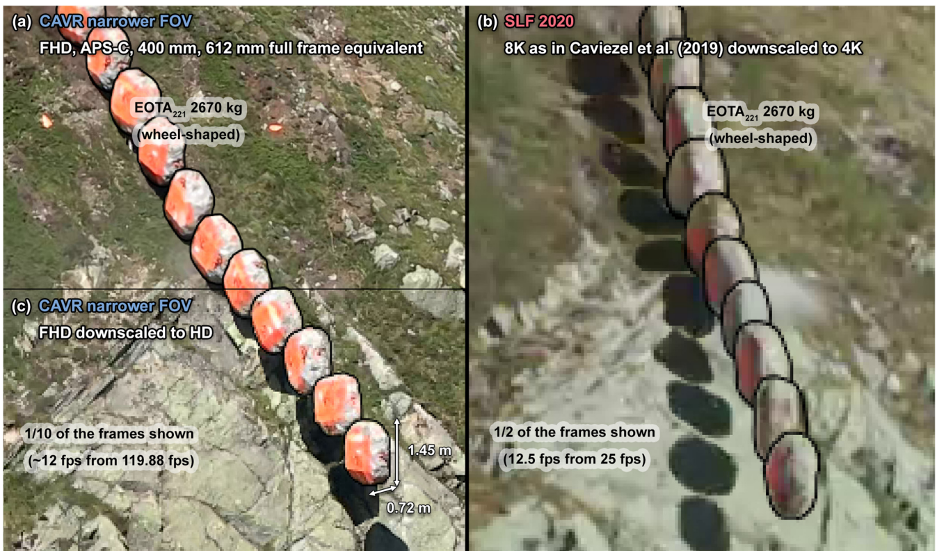
320 Figure 7: Comparison of the FHD (a) and HD (c) narrower FOV video footage captured with the CAVR camera setup shown in Fig. 6 with the wider SLF RED video footage (b) from Caviezel et al. (2020), described in Caviezel et al. (2019) for rocks with similar trajectories. The visible outline of the rocks is highlighted with a black line roughly hand drawn on the stacked frames to help distinguish the rocks from their background. Note the difference in sharpness and the level of details of the footage related to the captured resolutions and the field of view. For scale, the 1 m 3 2670 kg rocks have their rotations aligned around their shortest 325 diameters of 0.72 m and have their longest diameters equal to 1.45 m. They are the largest blocks tested at that site in Caviezel et al. (2021), and therefore, are the easiest to see on the video footage. The smallest equant blocks of 45 kg are approximately one- fifth of the length of these blocks and require detailed footage for proper tracking.
