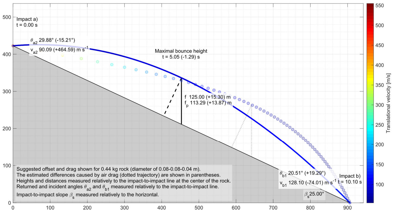
725 Figure A1: Unlikely/unrealistic extreme bounce of a hockey puck sized rock over an impact-to-impact distance ( s ) and slope ( \beta_s ) of 1 km and 25^\circ . The dotted trajectory considers the resistance caused by air drag but neglects the compressibility drag. The latter may play an important role in this extreme example however due to the high velocities beyond the speed of sound in the air. The drag is approximated numerically by updating g_t every \Delta t/1000 (0.01 s in that case), with one dot of the trajectory shown every 15 iterations.
