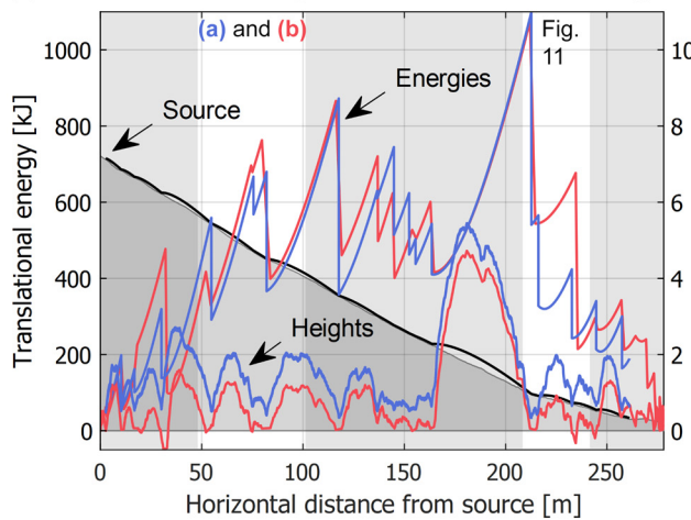
535 Figure 10: Side-by-side comparison of the reconstructed translational velocities, positions, translational energies, and bounce heights of the reconstructed trajectories with the CAVR method compared to the older trajectories from the SLF (Caviezal et al., 2020). The r1 and r2 rockfall runs correspond to the 6 th and 7 th runs performed by the SLF on September 13 th , 2019. The 3D reconstructed trajectories are overlaid on the stacked frames showing the rock positions every 10 frames (every ~1/12 th of a 540 second for the footage captured at 119.88 fps with the camera setup shown in Fig. 6). For scale, the dimensions of the 2670 kg orange reinforced disk or wheel shaped concrete rock are 1.45 m ( d_1 and d_2 ) by 0.72 m ( d_3 ). The reconstructed trajectory segments are shown in black with their respective slope profiles in gray as background elements of the 2D vertical profiles shown in (e) and 545 (f). The characteristic sawtooth shape of the energy profiles helps distinguish them from the bounce heights. The values from the CAVR method are shown in blue while those from the SLF are shown in red for a quantitative comparison. The portion of reconstructed trajectory segments shown over stacked video frames in (a), (b), (c), (d) and in Fig. (11) are highlighted in the 2D profiles (e) and (f) with white vertical bands.
