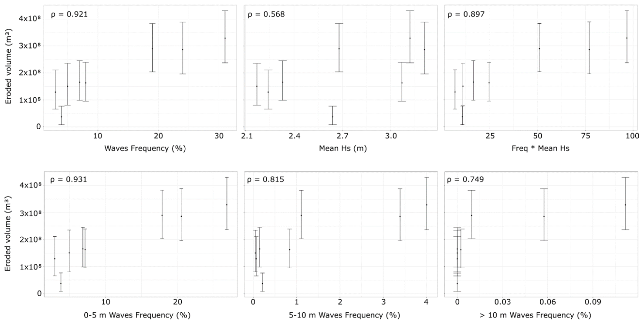
Figure 7: Quantification of the correlations ( \rho ) between the coastal cliff retreat and eroded volume, and the mean significant wave height (Hs) and frequency. Each point is a direction sector measuring 45°.
