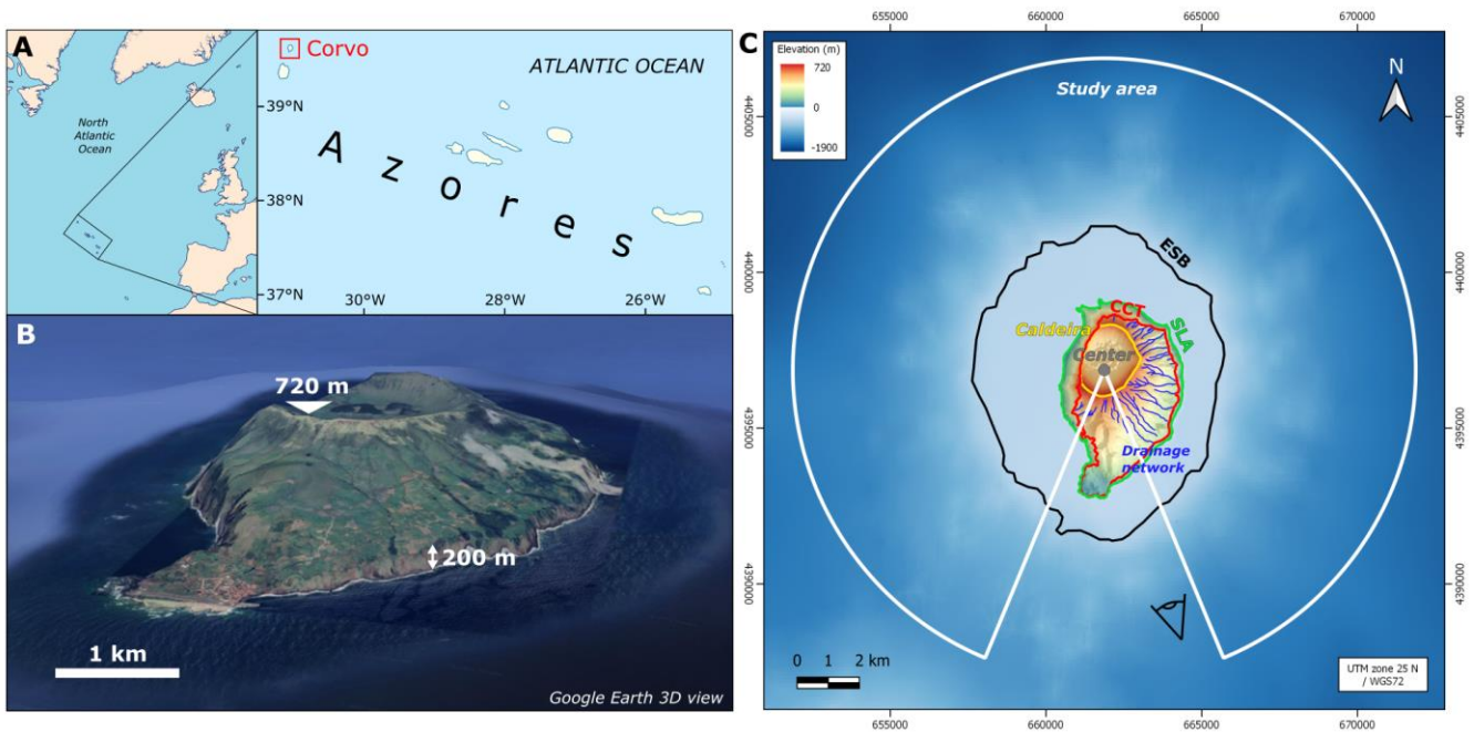
395 Figure 3: A: Location of Corvo Island. B: Corvo Island seen from the southeast (Google Earth 3D view). C: Topographic shaded relief map of the volcanic edifice of Corvo (ASTER and EMODnet data). White line: study area. Black line: ESB. Green line: coastline, SLA. Red line: CCT. Yellow line: edges of the Central Volcano caldera. Blue lines: drainage network on the slopes of Central Volcano. Grey dot: center of the volcanic edifice.
