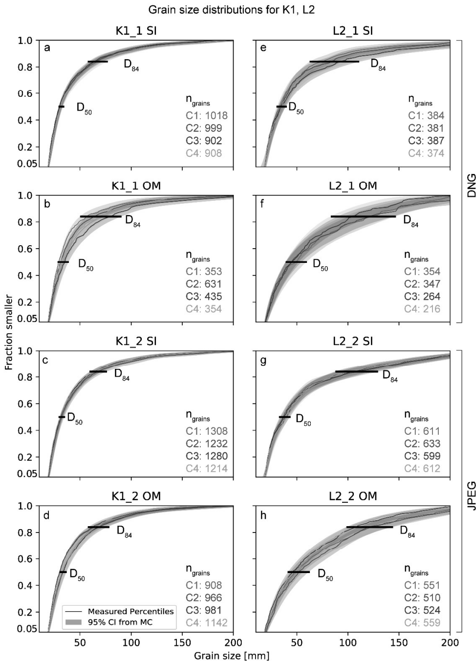
380 Figure 5: Selected grain size (i.e., b-axis length) distributions measured in different images (SI = single orthoimage, OM = orthophoto mosaic) from various UAV models (see Fig. 2 for model characteristics and colour legend) with the modelled 95% confidence interval (CI) for each percentile. All Kander (K1) data (a-d) in this figure refer to the region A, while all Luetschine (L2) data (e-h) correspond to the respective region B (see Fig. 1 for location). DNG = raw image acquisition format, JPEG = JPEG image acquisition format; D_{50} , D_{84} = Percentiles 50 and 84, respectively; n_{\text{grains}} = Number of segmented grains.
