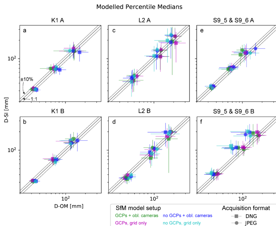
Figure 8: Modelled median values for percentiles D_{50} , D_{84} and D_{96} from single orthoimages (SI) and orthophoto mosaics (OM) for selected regions of the survey sites. Different SfM model setups are colour-coded, please see Fig. 2 for detailed legend. Displayed uncertainties represent modelled 95% confidence intervals. Please note the logarithmic scale.
