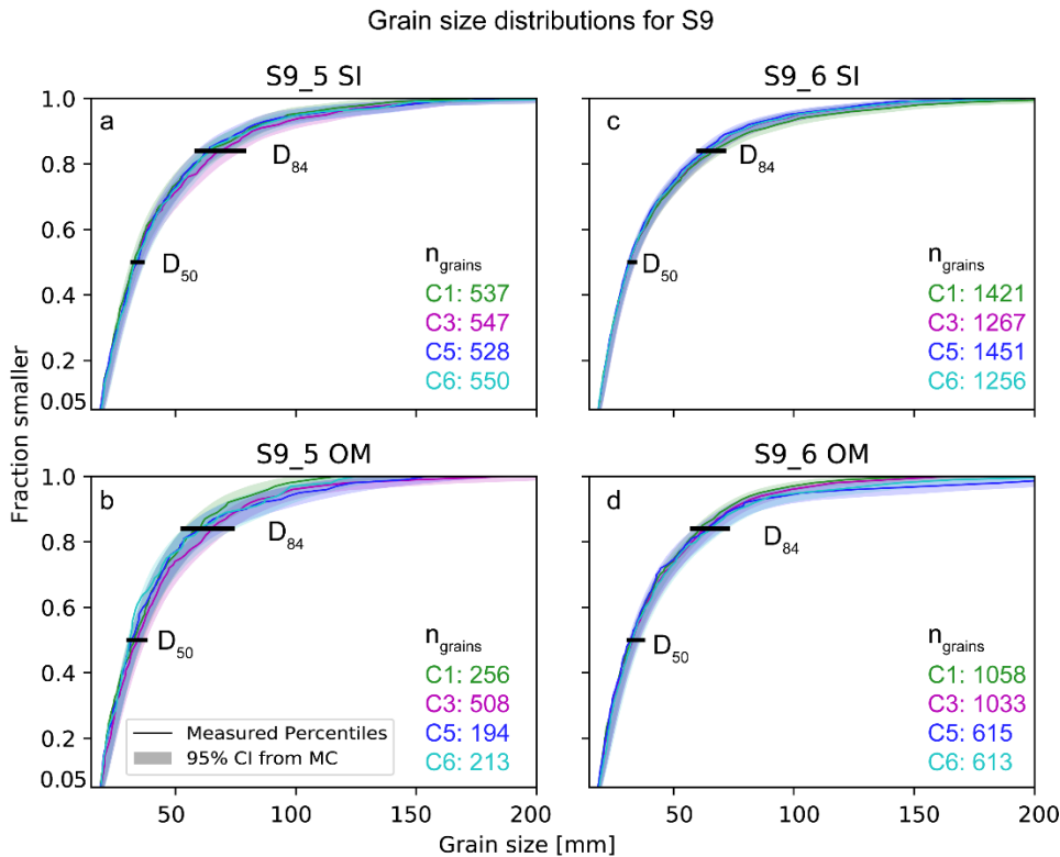
Figure 6: Grain size distributions and percentile uncertainty (modelled 95% confidence interval; CI) for the Entle surveys (S9) for different UAV imagery (SI = single orthoimage, OM = orthophoto mosaic; see Fig. 2 for model characteristics and colour legend). All data refer to the region A (see Fig. 1 for location). D50, D84 = Percentiles 50 and 84, respectively; n grains = Number of segmented grains. Please note that S9_5 (a, b) was acquired in raw image format (DNG) while S9_5 images (c, d) were acquired as JPEG images.
