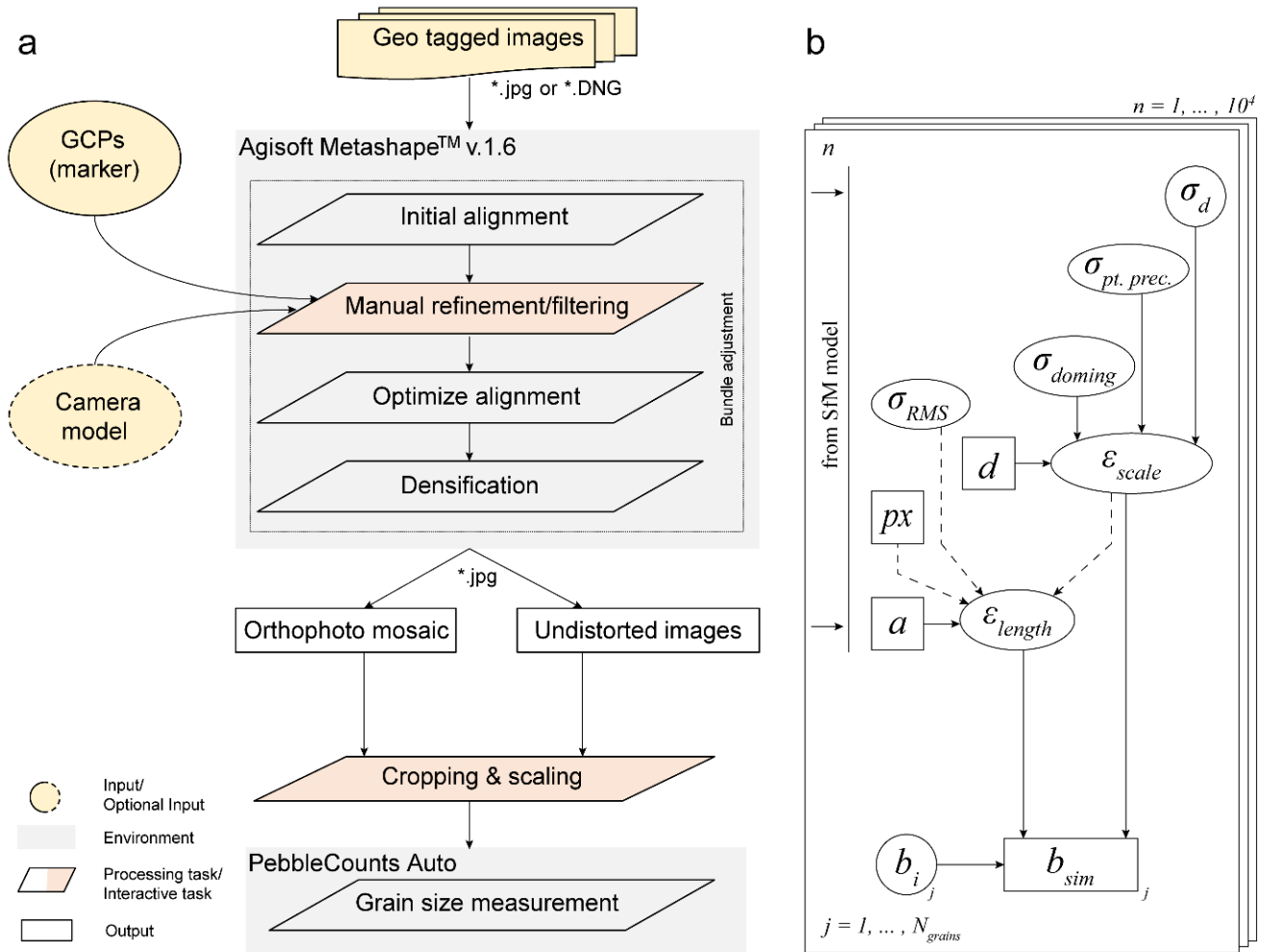
215 Figure 3: Workflow for grain size estimations from UAV-derived images. (a) Structure from motion workflow with PebbleCountsAuto (Purinton and Bookhagen, 2019) for grain size estimation. (b) Quantities used for estimating the uncertainty of the grain sizes. Quantities in squares denote image/survey-specific values, while variables in circles/ellipses are represented by a probability density function (pdf). Dashed arrows indicate quantities only used for uncertainty estimation in orthomosaics. For variable explanation, see S2.3 in the main text.
