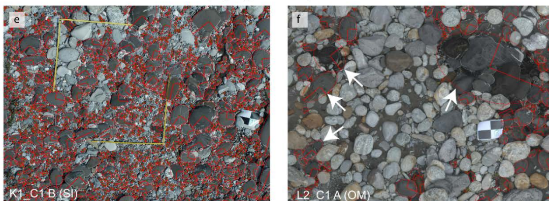
570 Figure 10: Systematic factors that influence grain size estimation from UAV imagery, especially from orthophoto mosaics (OM). (a,b) Effect of varying accuracy of SfM (Structure from Motion) used for referencing for orthophotomosaics which should display the same extent. (c,d) Comparison of undistorted single images (SI) with orthophoto mosaics, which highlight small scale image warping and artefacts: 1) Duplication from incorrect image stitching, 2) Blurring of pebble boundaries, and 3) irregular grain shapes. (e,f) Selected results highlighting the varying image segmentation performance. Examples of systematic under-segmentation marked with white arrows.
