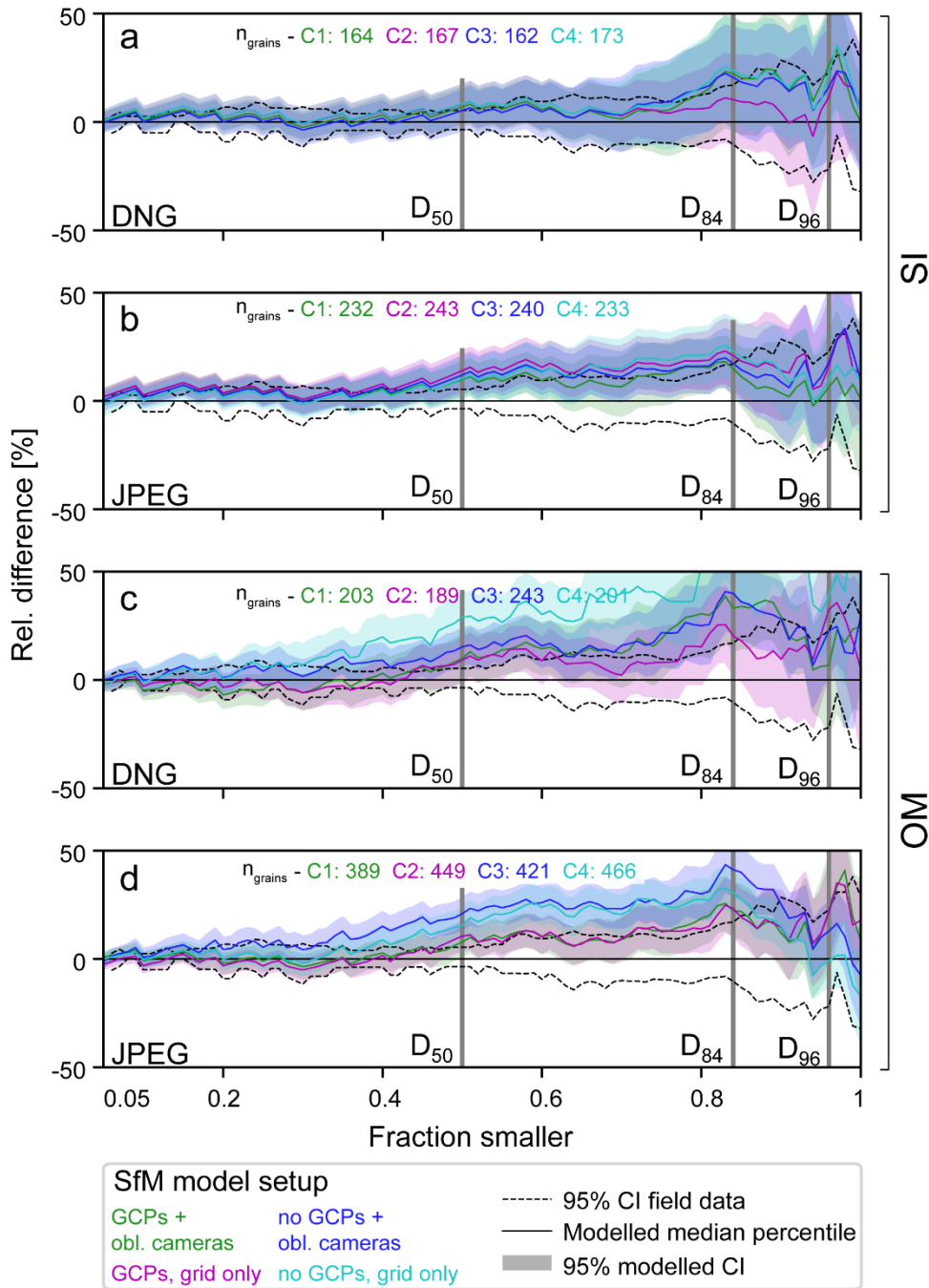
545 Figure 9: Relative difference between grain size percentiles estimated from UAV imagery to grain sizes, which were measured in the field for the region A of the Kander survey (K1). (a, b) Results for data from single orthoimages (SI). (c, d) Results for orthophoto mosaics (OM). DNG and JPEG indicates the image acquisition format. Key percentiles, i.e., D_{50} , D_{84} and D_{96} , are highlighted. The number of detected grains ( n_{\text{grains}} ) and the data are colour-coded for SfM model setup (see Fig. 2 for detailed legend).
