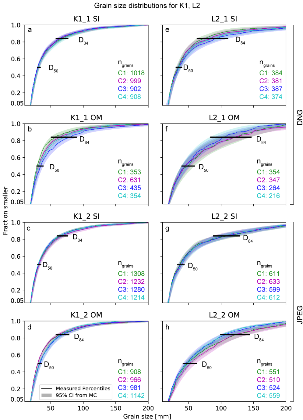
380 Figure 5: Selected grain size (i.e., b-axis length) distributions measured in different images (SI = single orthoimage, OM = orthophoto mosaic) from various UAV models (see Fig. 2 for model characteristics and colour legend) with the modelled 95% confidence interval (CI) for each percentile. All Kander (K1) data (a-d) in this figure refer to the region A, while all Luetschine (L2) data (e-h) correspond to the respective region B (see Fig. 1 for location). DNG = raw image acquisition format, JPEG = JPEG image acquisition format; D_{50} , D_{84} = Percentiles 50 and 84, respectively; n_{\text{grains}} = Number of segmented grains.
