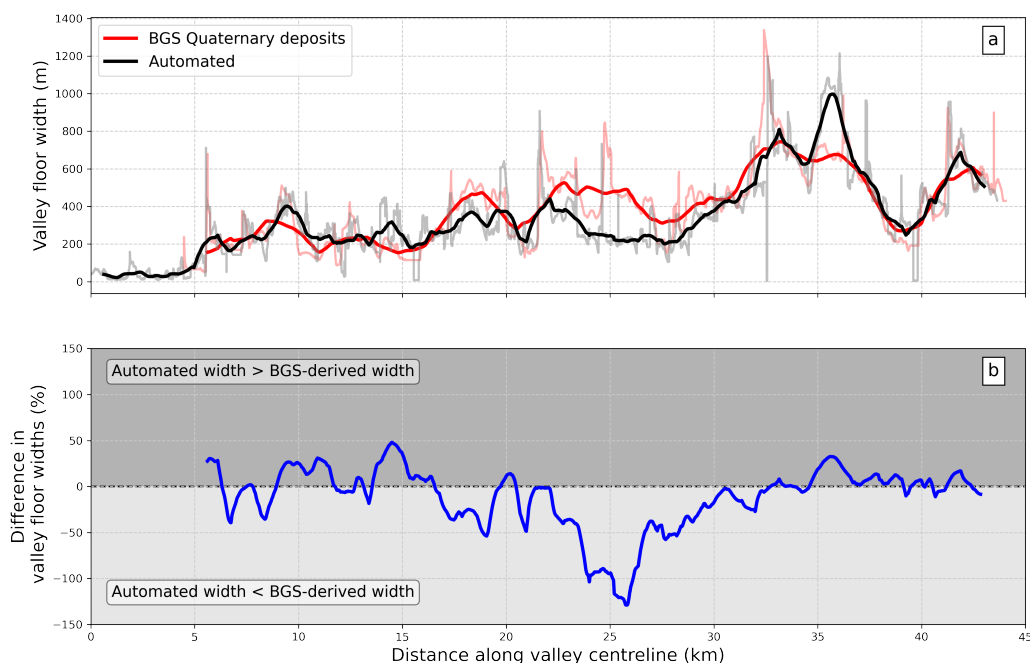
Figure 6. Results of valley floor width comparison for Weardale. (a) valley floor width from upstream to downstream along the centreline for the automated method (black) and derived from the BGS Quaternary maps (red). The light grey and red lines show the raw data, and the darker lines show a rolling average of width over a 500 m window. (b) Percentage difference between the two datasets along the centreline, where positive values indicate a wider automated width than BGS-derived, and negative values indicated a narrower automated width than BGS-derived.
