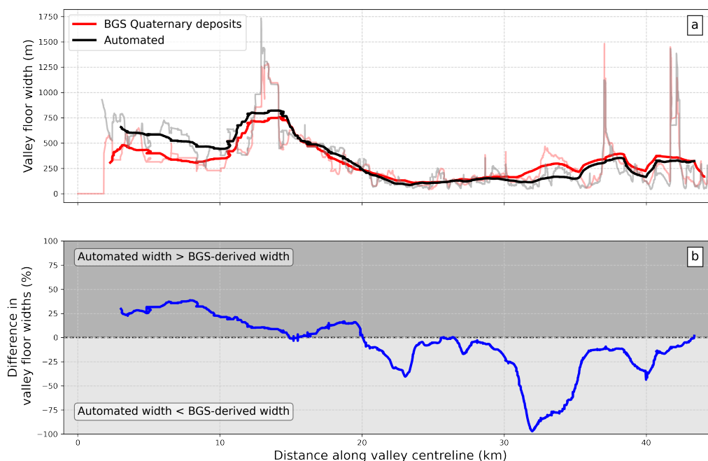
Figure 4. Results of valley floor width comparison for the River Tweed. (a) valley floor width from upstream to downstream along the centreline for the automated method (black) and derived from the BGS Quaternary maps (red). The light grey and red lines show the raw data, and the darker lines show a rolling average of width over a 500 m window. (b) Percentage difference between the two datasets along the centreline, where positive values indicate a wider automated width than BGS-derived, and negative values indicated a narrower automated width than BGS-derived.
