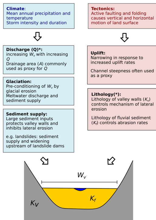
Figure 1. Conceptual model highlighting key controls on valley floor width ( W_v ). Climate affects river discharge, sediment supply, and the extent of glaciation within catchments. Tectonics controls uplift rates and lithology by juxtaposing contrasting lithological units. The influence of each factor on valley floor width is highlighted in the respective box. Factors labelled with an asterisk(*) are those included within existing models predicting valley floor width.
