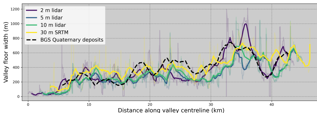
Figure 7. Valley floor width along the valley centreline for the Weardale catchment, tested on DEMs of varying resolution. We show the results from lidar-derived datasets at 2 m, 5 m, and 10 m, along with the SRTM 30 m dataset. The black dashed line shows the results from the valleys identified using the BGS Quaternary deposits maps (scale of 1:50,000, corresponding to a DEM resolution of \approx 25 m).
