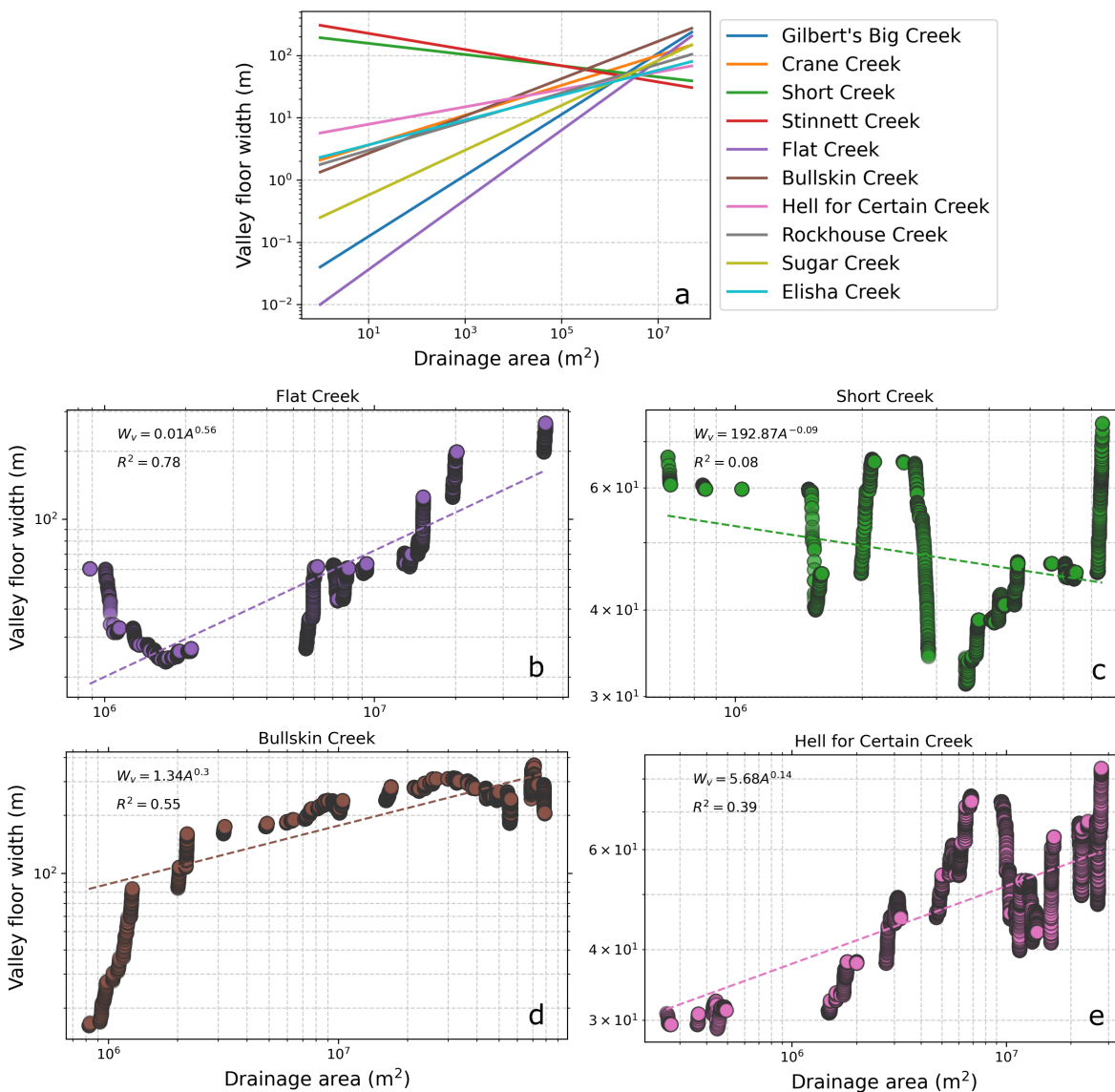
Figure 11. Width-area analysis for rivers in the Cumberland Plateau, Kentucky, USA. a) Fitted power-law relationships for each of the rivers, showing eight of the rivers demonstrated a positive W_v - A relationship while two of the rivers showed no relationship between W_v and A . Example width-area plots for b) Flat Creek; c) Short Creek; d) Bullskin Creek; and e) Hell for Certain Creek showing variability between basins.
