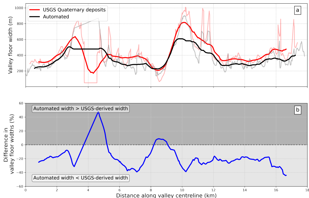
Figure 9. Results of valley floor width comparison for the Russian River. (a) Valley floor width from upstream to downstream along the centreline for the automated method (black) and derived from the USGS Quaternary maps (red). The light grey and red lines show the raw data, and the darker lines show a rolling average of width over a 500 m window. (b) Percentage difference between the two datasets along the centreline, where positive values indicate a wider automated width than USGS-derived, and negative values indicated a narrower automated width than USGS-derived.
