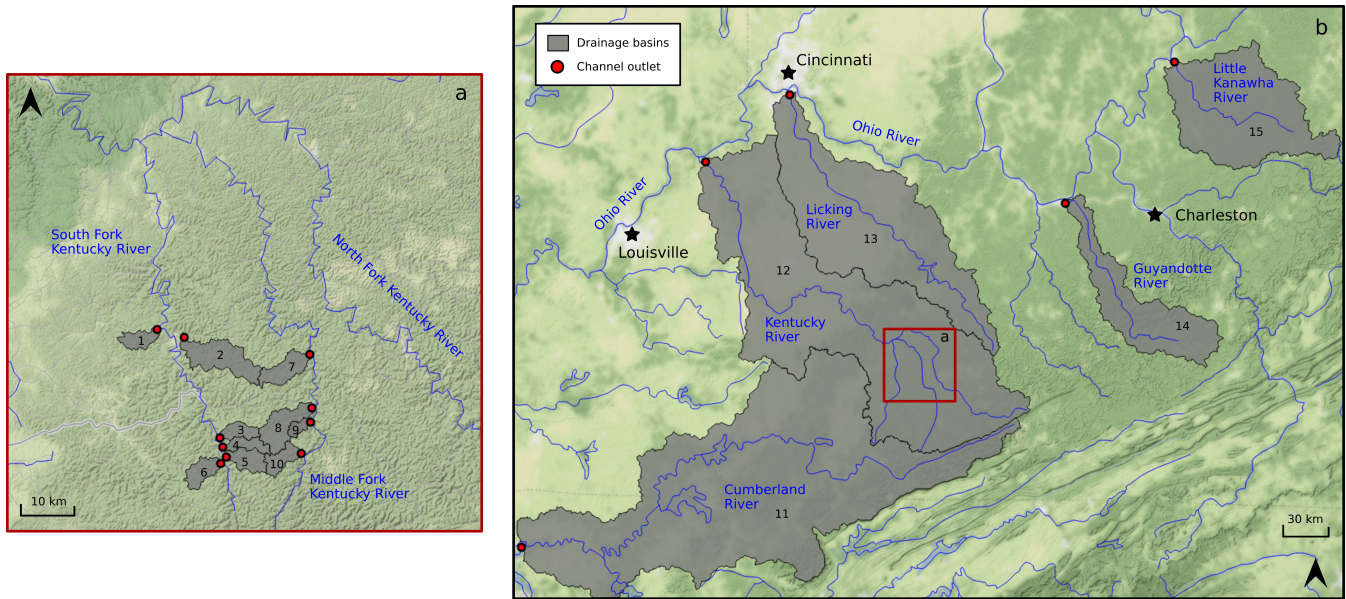
Figure 10. Location of the sites for width-area analysis in the Cumberland and Allegheny Plateaus, southwestern Appalachians, USA. a) Small creeks in the Cumberland Plateau; b) large rivers in the Cumberland and Allegheny Plateaus. The red circles mark the outlet of each catchment analysed, labelled 1-15. The tributary where the North and South Forks of the Kentucky River join is located at 37°34'13"N, 83°42'39"W (WGS84). Map tiles by Stamen Design under CC BY 3.0; data © OpenStreetMap contributors. Distributed under the Open Data Commons Open Database License (ODbL) v1.0.
