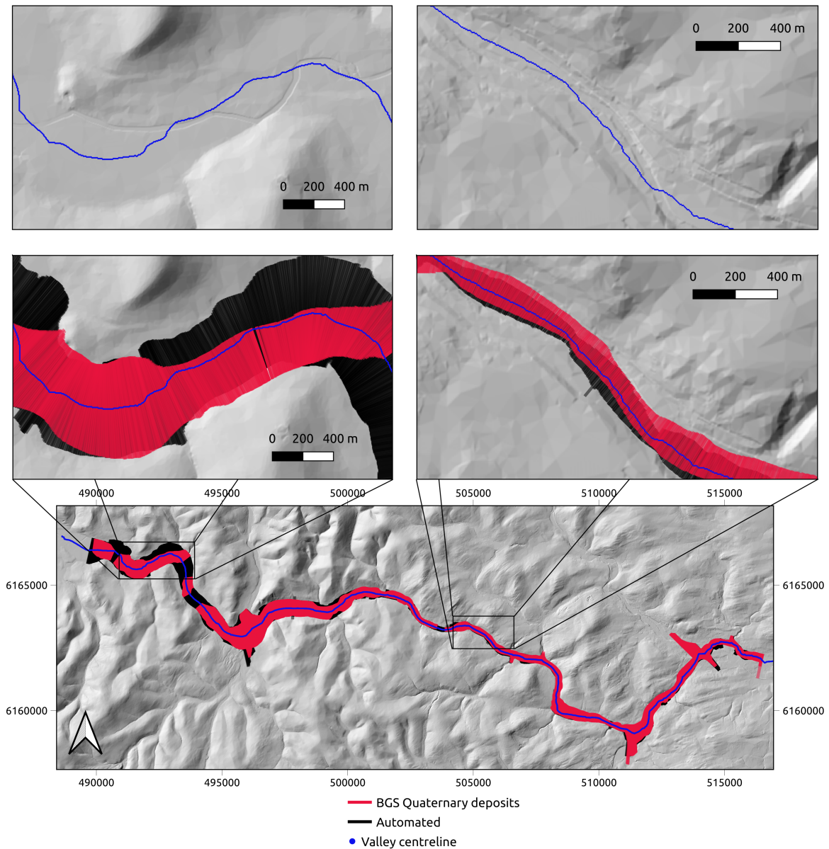
Figure 5. Hillshade of the River Tweed showing the valley floor widths extracted using the automated method (black) and those derived from the BGS Quaternary maps (red). The valley centreline is shown in blue. The left zoomed-in region shows an example of where the automated method is wider than the BGS Quaternary, but picks up the break-in-slope transition to the hillslopes. The right zoomed-in region shows an example of where the two datasets are consistent. The coordinate system is WGS UTM Zone 30N.
