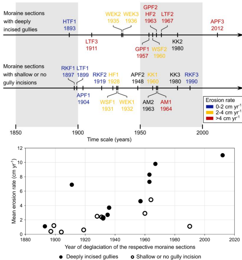
Figure 11: Mean erosion rates in time period 3 (see Table 4 for specific DoDs) in dependence on the years of deglaciation of the moraine sections with deeply incised gullies and shallow or no gully incision. Timeline with the years of deglaciation of the moraine sections, individually for slopes with deeply incised gullies and slopes with only little or no gully incisions. Colouring of the moraine sections regarding the mean erosion rates of the DoDs in time period 3 (see Table 3 for specific DoDs; erosion rate of 0–2 cm yr -1 in blue, 2–4 cm yr -1 in orange and >4 cm yr -1 red)
