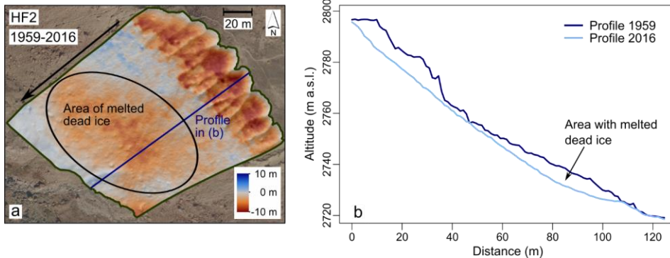
385 Figure 5: Reaction of lateral moraine slopes to dead ice melting on base of the example of moraine section HF2: (a) DoD of 1959-2016 and (b) length profile through the DEMs of 1959 and 2016 (Sources of aerial images: 1959 IGMI, 2016 Hydrographic Office, Agency for Civil Protection, Autonomous Province of Bolzano-South Tyrol)
