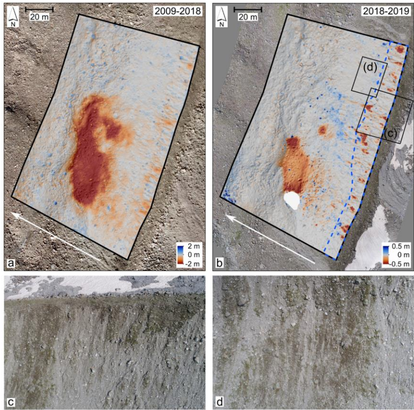
505 Figure 9: Slope with little incised gullies or rills illustrated for moraine section APF2 in the Alpeiner Ferner forefield: (a): DoD 2009–2018 (Source of aerial images 2009: Office of the Tyrolean government), (b) DoD 2018–2019 with the erosion area (blue), (c) – (d): Drone images of the slope of 01.08.2019
