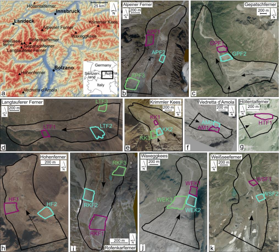
125 Figure 1: Study areas: (a) Map with an overview over the location of the glacier forefields (ASTER DEM of NASA, METI and J-spacesystems), (b) – (k) orthophotos showing the ten investigated glacier forefields and the moraine sections which were investigated in detail, arrows showing the flow direction of the glacier. Orthophotos calculated on base of the following aerial image datasets: Alpeiner Ferner 2009 (Office of the Tyrolean government, Department of Geoinformation, Austria), Langtaufferer Ferner 2016
