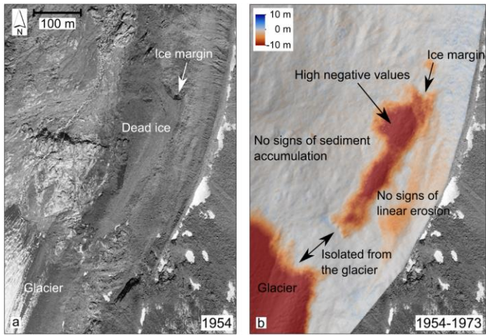
265 Figure 2: Detection of debris covered dead ice using the example of the Alpeiner Ferner: (a) Orthophoto of 1954 and (b) DoD of 1954–1973 (Sources of aerial images: 1954 BEV, 1973 Office of the Tyrolean government)
