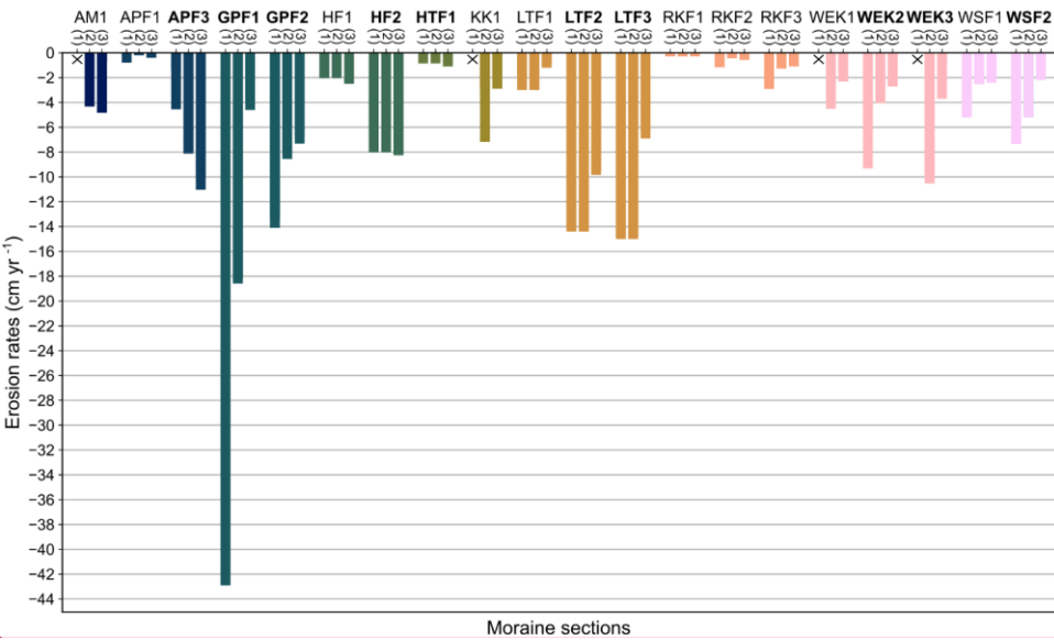
Figure 10: Erosion rates for 20 investigated moraine upper slopes for the three time periods 1950s–1970s (1), 1970s–2000s (2) and 2000s–2018 (3) (see Table 4 for specific DoDs). Moraine sections written in bold represent upper slopes with deeply incised gullies (colour map batlow10 from Crameri et al., 2020)
