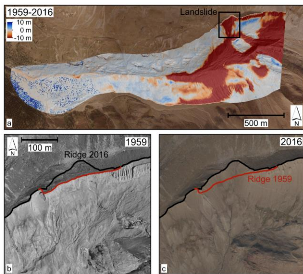
Figure 7: Landslide on the lateral moraine of Langtauferer Ferner: (a) DoD 1959–2016 of the entire glacier forefield, (b) aerial image of 1959 and (c) aerial image of 2016 (Sources of aerial images: 1959 IGMI, 2016 Hydrographic Office, Agency for Civil Protection, Autonomous Province of Bolzano-South Tyrol)
