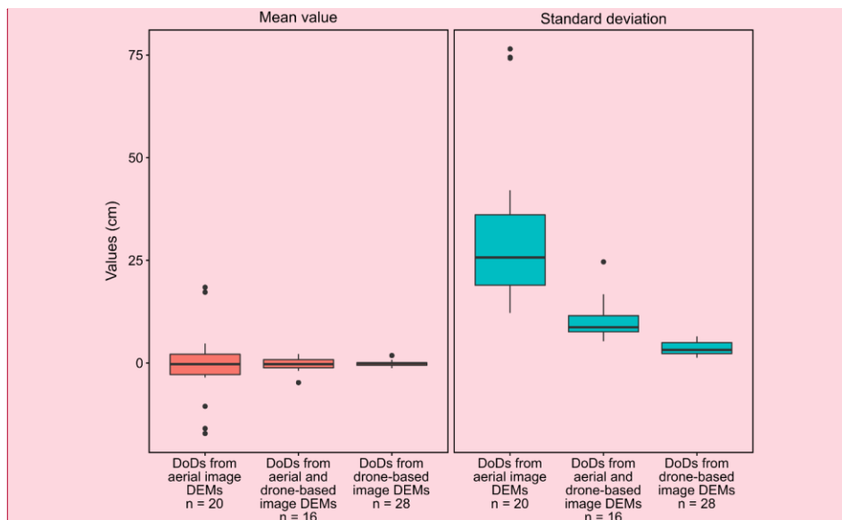
Figure 4: Boxplots showing the distribution of the mean values and standard deviation for different types of DoDs: DoDs calculated on base of aerial images, DoDs calculated on base of aerial and drone images and DoDs out of two sets of drone images
