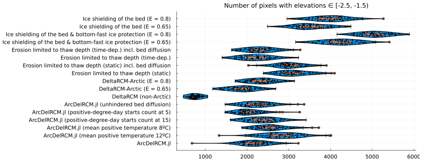
Figure 7. An analogous plot to Figure 6, but showing the number of pixels with elevation \in [-2.5, -1.5) m. Since the modelled ramp feature that forms under h_{ice,max} = 2 m lies mostly in this elevation range, we use this value as a proxy to the size of the ramp, even though it inevitably include delta pixels that are not part of a ramp feature but happen to be in the same elevation range. This is evident when comparing the DeltaRCM-Arctic ( E = 0.8 ) and ArcDelRCM.jl cases with Figures 5a and b. The pixels with relevant elevations are more concentrated around channel outlets in the former, while they are more distributed along the delta shore in the latter (forming the ramp).
