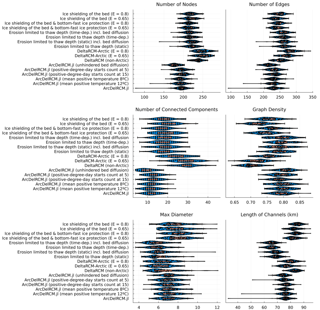
Figure 6. Bed-elevation-output Plots showing delta metrics determined by the graph analysis we performed on each of DeltaRCM-Arctic (a), ArcDelRCM the configurations described in Section 3.2. jl (b) The blue violin plots show the kernel density estimate, the orange box and with modifications described in Sect whisker plots show the central 50%, maximum, median, and minimum values, and the black dots show the actual values of the individual simulations. 2.2.4 applied individually or in tandem, as indicated by the title titles of each panel (e-h) sub-figures in Figure 5. Note The metrics of the 2-m-ramp variant cases not explicitly shown in the full model this text (i.e., all cases with E = 0.65 , ArcDelRCM.jl with unhindered bed diffusion, and the case in which ice-shielding and ice-protections non-Arctic DeltaRCM ) are applied together included for comparison.
