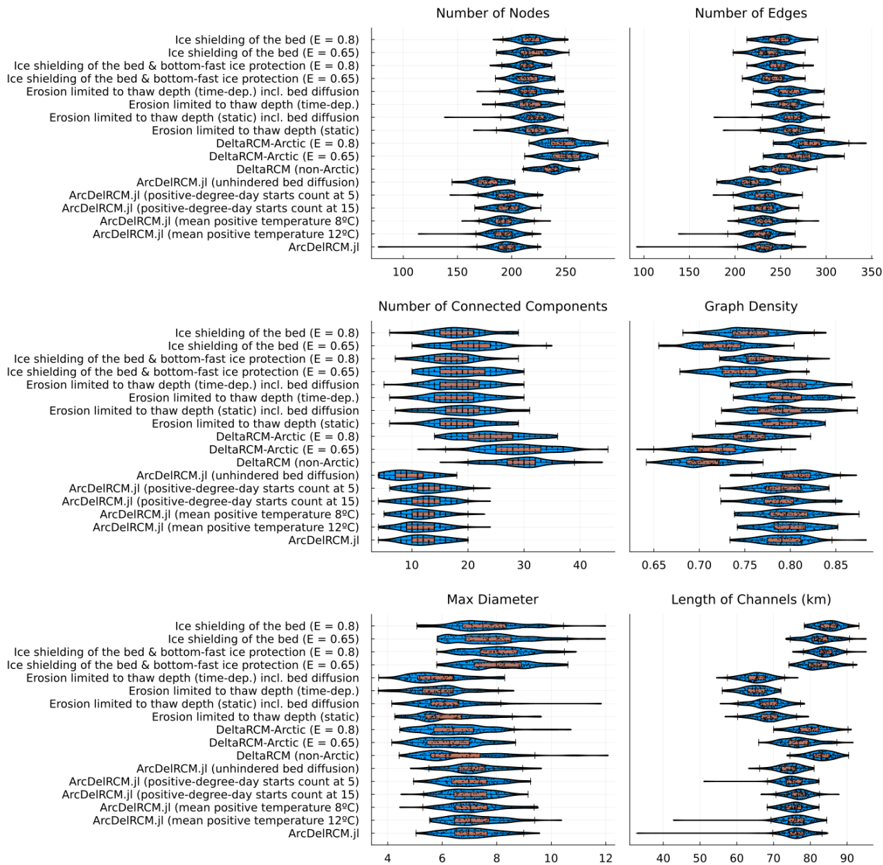
Figure 6. Plots showing delta metrics determined by the graph analysis we performed on each of the configurations described in Section 3.2. The blue violin plots show the kernel density estimate, the orange box and whisker plots show the central 50%, maximum, median, and minimum values, and the black dots show the actual values of the individual simulations. The labels along the vertical axes correspond to the titles of each sub-figures in Figure 5. The metrics of the variant cases not explicitly shown in this text (i.e., all cases with E = 0.65 , ArcDeIRCM.jl with unhindered bed diffusion, and the non-Arctic DeltaRCM) are included for comparison.
