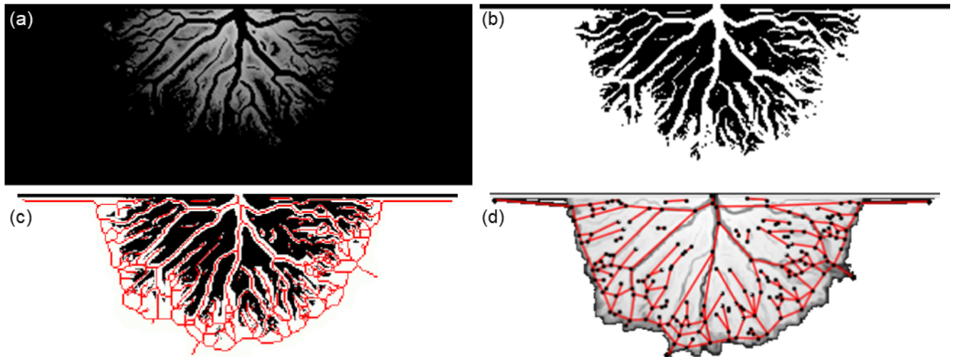
Figure 3. Exemplary overview of workflow to extract the hydrological graph from the imaged delta simulation. (a) bed elevation, (b) binarization of bed elevation to differentiate between channels and non-channels, (c) skeleton (in red) of the channels overlaid on the binary image (b), (d) graph of the channel network derived from the skeleton in (c) with edges in red and nodes in black overlaid on the delta elevation.
