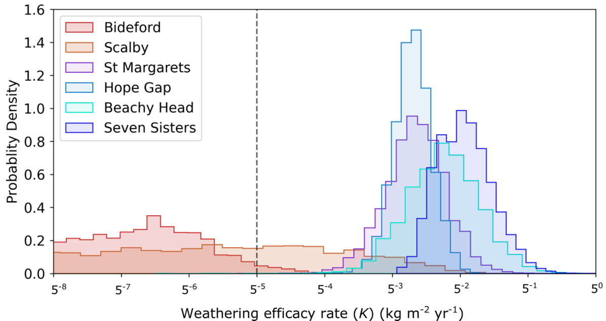
635 Figure 8: Posterior histograms of likelihood-weighted, accepted MCMC weathering efficacy rate ( K ) samples. Here weathering rate is calculated as F_R \times K . Red and orange histograms show the results for the two sandstone sites: Bideford and Scalby. Blue, purple, green histograms show the results for the four chalk sites: St. Margarets, Hope Gap, Beachy Head and Seven Sisters. Above the dashed line (where K < 5^{-5} ) is when weathering is active across the shore platform. Below the dashed line (where K < 5^{-5} ) is when weathering processes are negligible.
