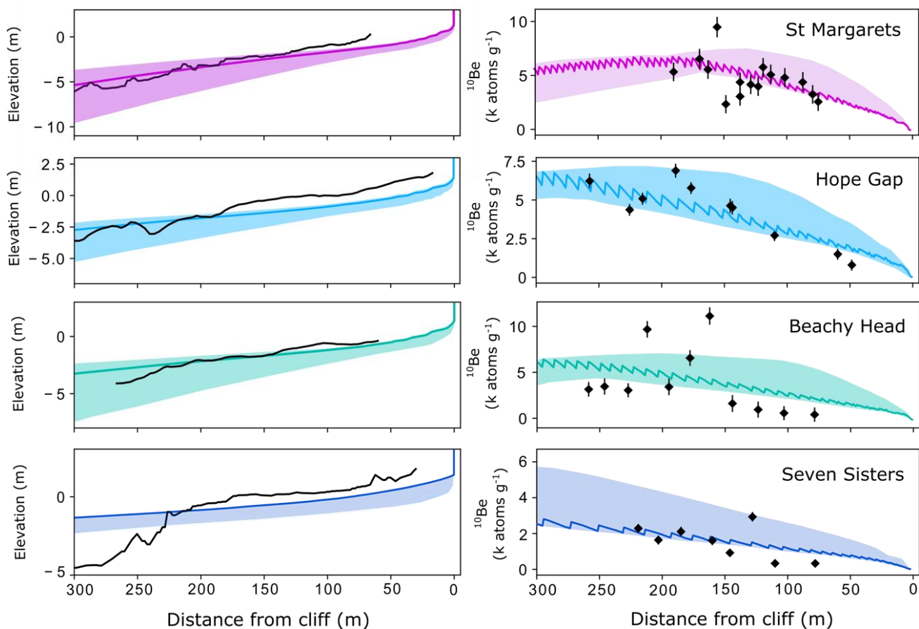
445 Figure 5: Best-fit model results from a 50–50% topographic– ^{10}\text{Be} concentration weighted MCMC inversion for chalk sites at St Margaret’s, Hope Gap, Beachy Head and Seven Sisters. Dark lines show best-fit results and shaded areas show the confidence interval range. The 16%–84% confidence interval for each free parameter in the MCMC inversion ( F_R , K , and y ) was simulated against the median results for the other parameters. The shaded uncertainty was constructed from the upper and lower limits of the model outputs. For both the topographic profile and ^{10}\text{Be} concentrations, the width of the modern-day, 300 m intertidal shore platform is shown. The modern-day cliff position is at 0 m. The panels on the left side compare the modelled results (coloured) to the measured data (black line) of the topographic profile. The panels on the right side compare the modelled results (coloured) to the measured data (black scatter) of the ^{10}\text{Be} concentration profile. 450
