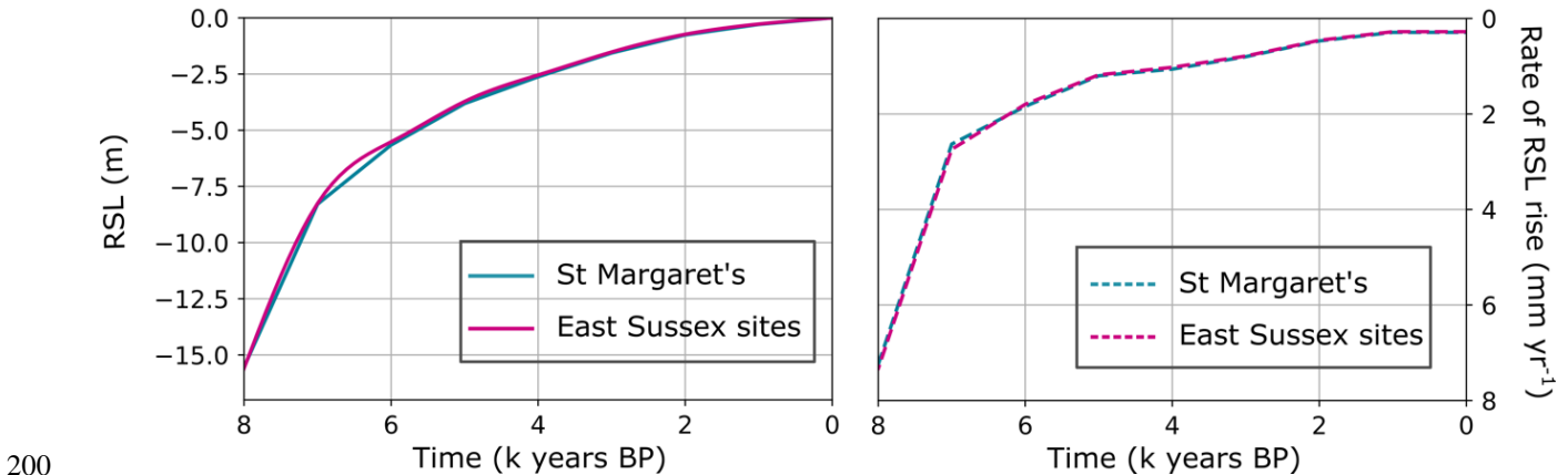
Figure 2: Relative Sea Level (RSL) (m) and the rate of RSL rise (mm yr -1 ) calculated every 1000 years for the site St Margaret's (blue) and the East Sussex sites, including Seven Sisters, Beachy Head, and Hope Gap (pink). RSL histories were provided by the GIA model of Bradley et al. (2011).
