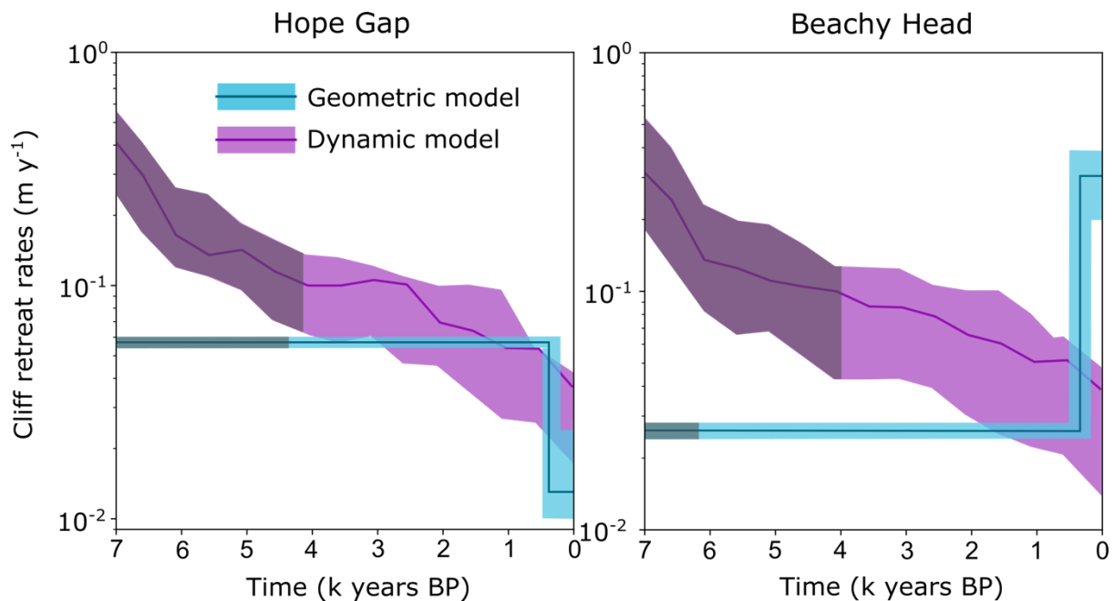
580 Figure 7: Comparisons between cliff retreat rates produced from a dynamic coastal evolution (Matsumoto et al., 2016) model and a geometric coastal evolution model (Hurst et al., 2016) for sites Hope Gap and Beachy Head. Cliff retreat rates (m yr -1 ) are shown for 7000 years BP to present day. The shaded regions highlight the timeframes that extend beyond the measured data in the past.
