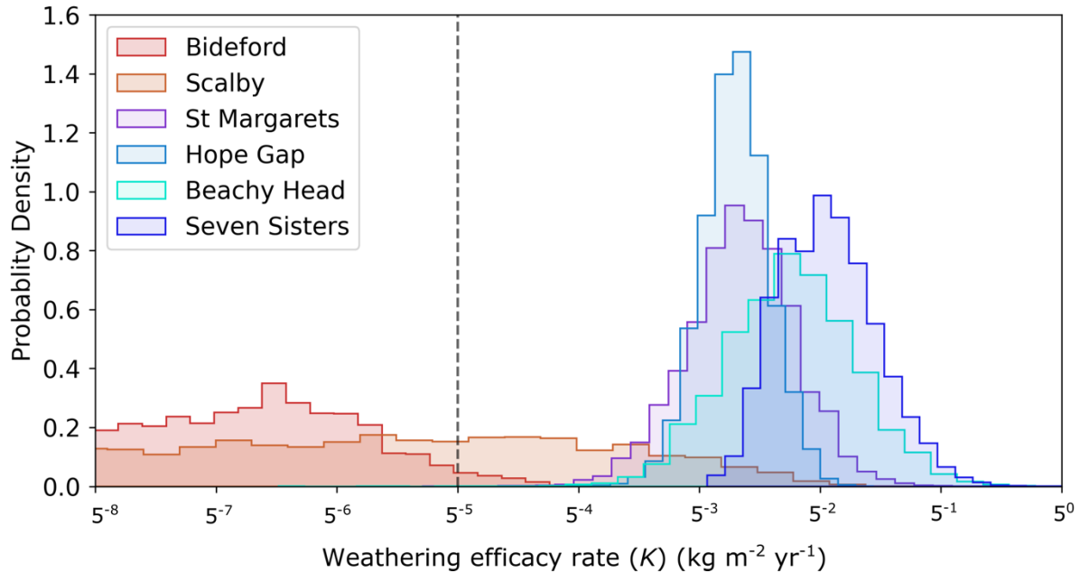
630 Figure 8: Posterior histograms of likelihood-weighted, accepted MCMC weathering efficacy rate ( K ) samples. Here weathering rate is calculated as F_R \times K . Red and orange histograms show the results for the two sandstone sites: Bideford and Scalby. Blue, purple, green histograms show the results for the four chalk sites: St. Margarets, Hope Gap, Beachy Head and Seven Sisters. Above the dashed line (where K < 5^{-5} ) is when weathering is active across the shore platform. Below the dashed line (where K < 5^{-5} ) is when weathering processes are negligible.
