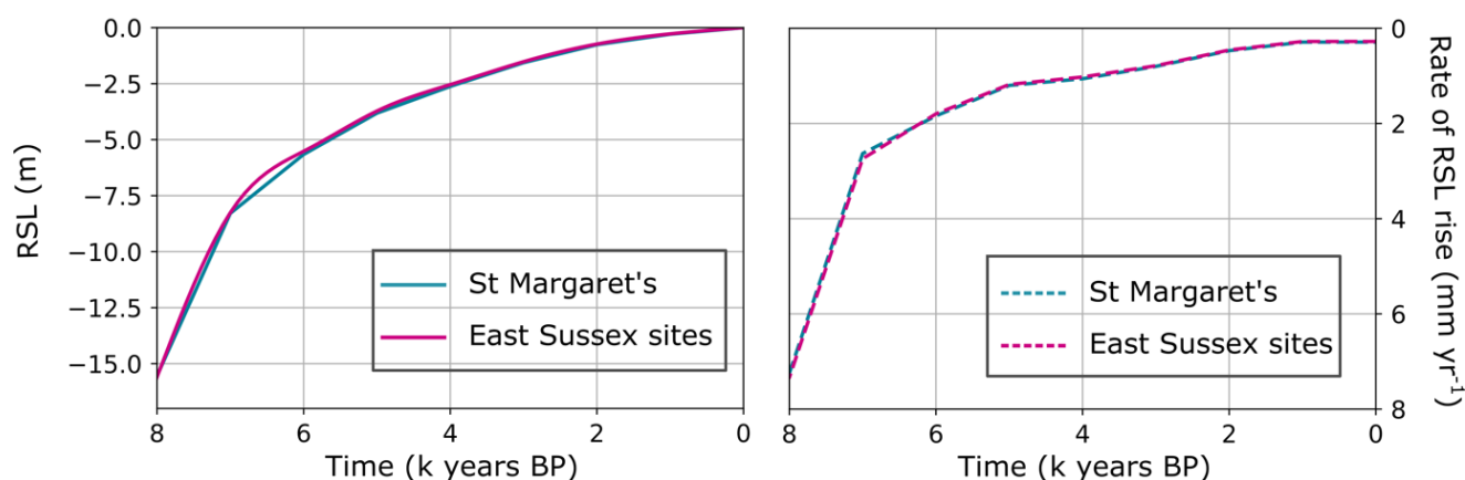
Figure 2: Relative Sea Level (RSL) (m) and the rate of RSL rise (mm yr -1 ) calculated every 1000 years for the site St Margaret's (blue) and the East Sussex sites, including Seven Sisters, Beachy Head, and Hope Gap (pink). RSL histories were provided by the GIA model of Bradley et al. (2011).
