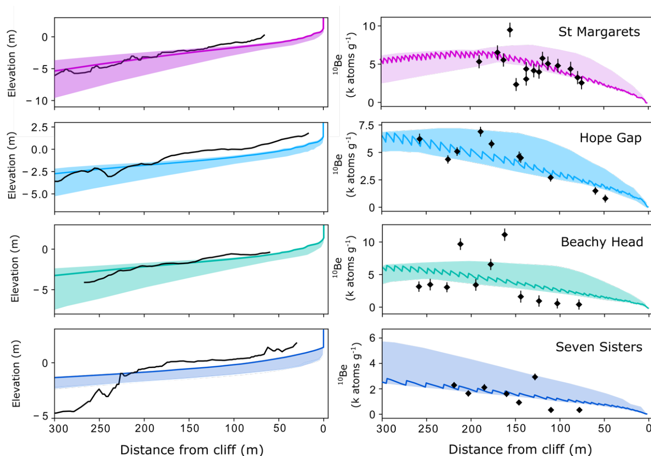
435 Figure 5: Best-fit model results from a 50–50% topographic– ^{10}\text{Be} concentration weighted MCMC inversion for chalk sites at St Margaret’s, Hope Gap, Beachy Head and Seven Sisters. Dark lines show best-fit results and shaded areas show the confidence interval uncertainty range. The 16%–84% confidence interval for each free parameter in the MCMC inversion ( F_R , K , and y ) was simulated against the median results for the other parameters. The shaded uncertainty was constructed from the upper and lower limits of the model outputs. For both the topographic profile and ^{10}\text{Be} concentrations, the width of the modern-day, 300 m intertidal shore platform is shown. The modern-day cliff position is at 0 m. The panels on the left side compare the modelled results (coloured) to the measured data (black line) of the topographic profile. The panels on the right side compare the modelled results (coloured) to the measured data (black scatter) of the ^{10}\text{Be} concentration profile. 440
