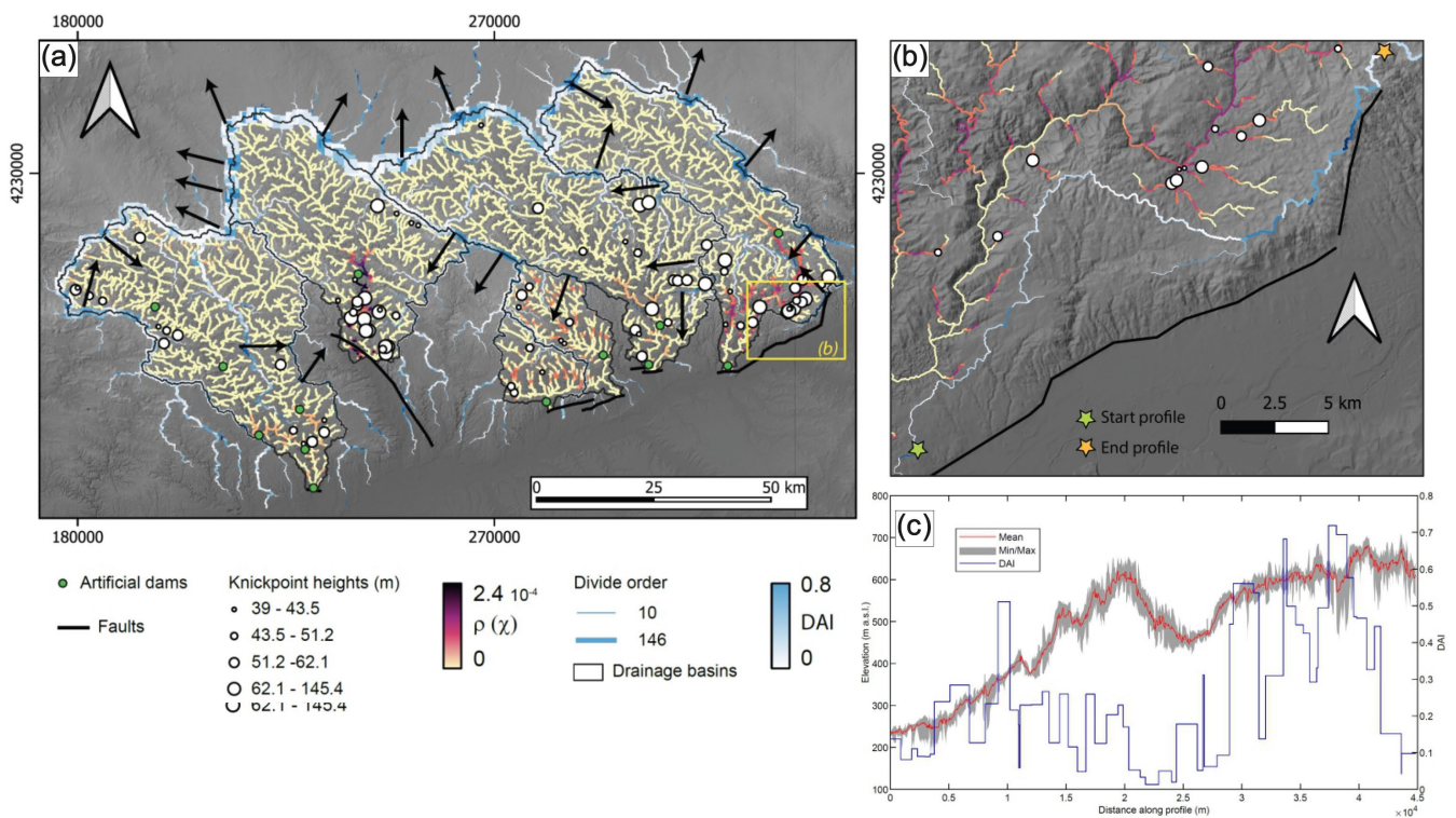
595 Fig. 11. (a) Observed and expected spatial patterns of knickpoints in the selected Sierra Morena basins. The intensity ( \rho ) values are computed on the knickpoint dataset without artificial dams. The drainage divide network asymmetry (DAI) sized by order is reported and the inferred movement is indicated by the black arrows. The elevation base is the 12 m resolution TanDEM-X DEM (Wessel, 2016). The reference system is WGS84 UTM 30N. (b) Detail of Fig.11a with ( \rho ) and DAI values of S6 in the sector of the capture elbow. (c) Along divide swath profile with a width of 1000 m and 600 corresponding DAI values (note the presence of wind gaps along the SE divide).
