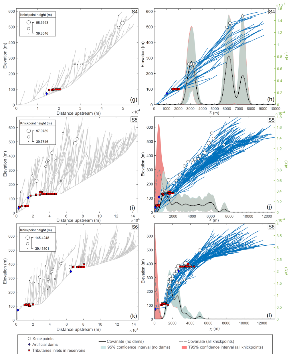
500 Fig. 9. Knickpoint distribution along S1-S6 stream networks. (a), (c), (e), (g), (i) and (k) river longitudinal profiles; (b), (d), (f), (h), (j), and (l) \chi transformed longitudinal profiles. The covariance estimates for knickpoints, calculated on the \chi transformed distance from the outlet (spatial covariate) with and without dams, indicate the probability of having knickpoints along the transformed profile. Knickpoints, sized by height, artificial dams, and tributary inlets into the reservoirs are projected on profiles.
